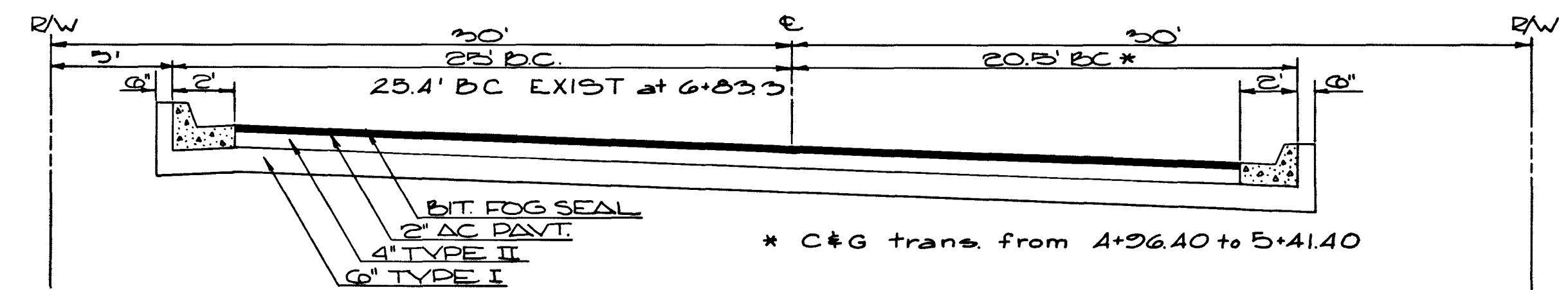
SECTION J 4+26.40-6+83.30 DESERT(N)
