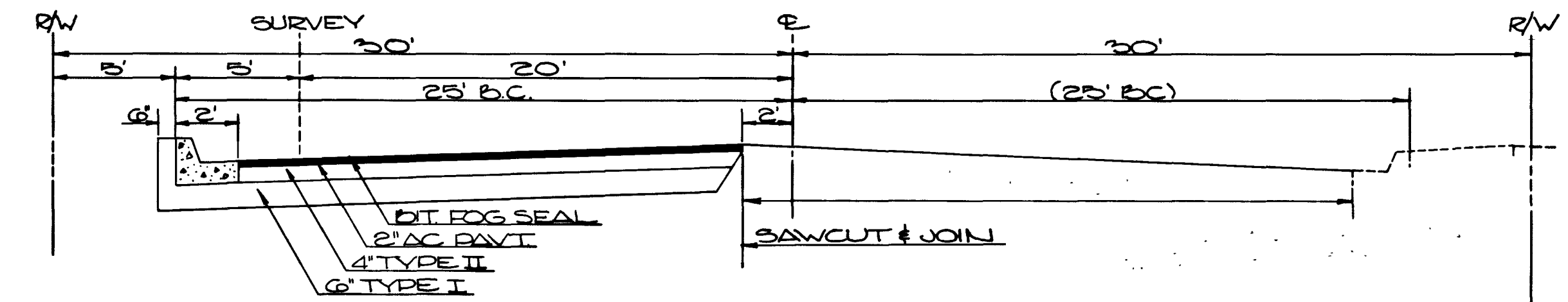
SECTION F 7+60.50-10+85 ELLIS NOTE - TRANSITIONS TO CROSSFALL @ INTERSECTION WITH DESERT(S)
