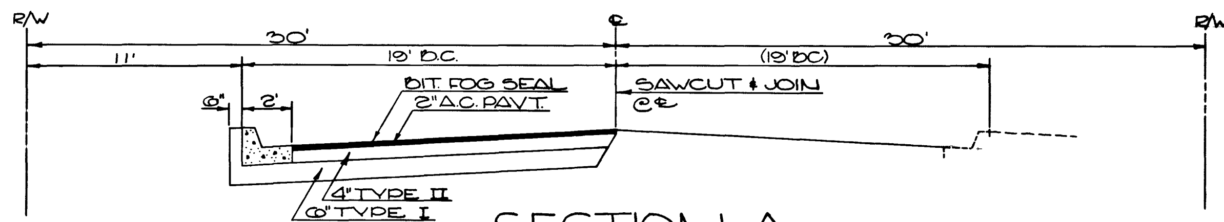
SECTION A 0+00-2+46.60 WALDMAN
