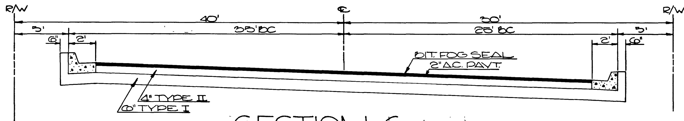
SECTION G 4+00-9+31.28 DESERT(S)
