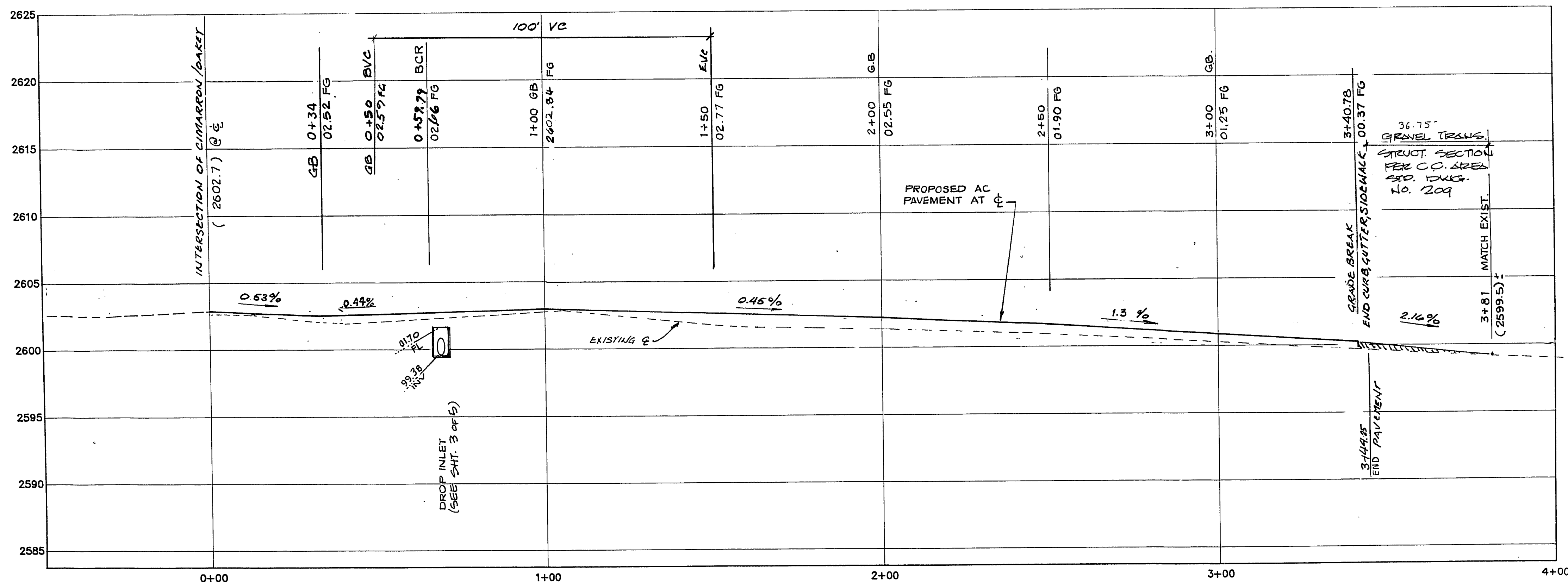
CIMARRON ROAD PROFILE SCALE: 1" = 20' - HORIZONTAL 1" = 5' - VERTICAL
