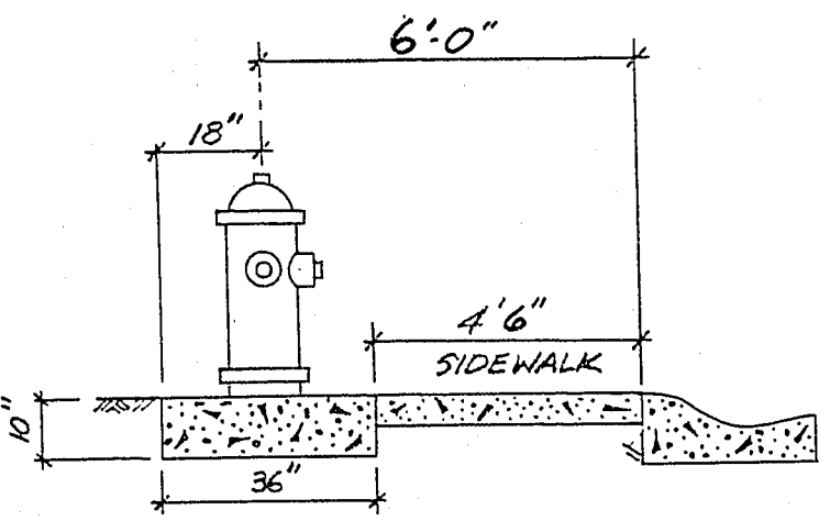
FIRE HYDRANT LOCATION DETAIL
