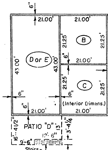
2ND FLOOR PLAN (REGULAR UNITS)
