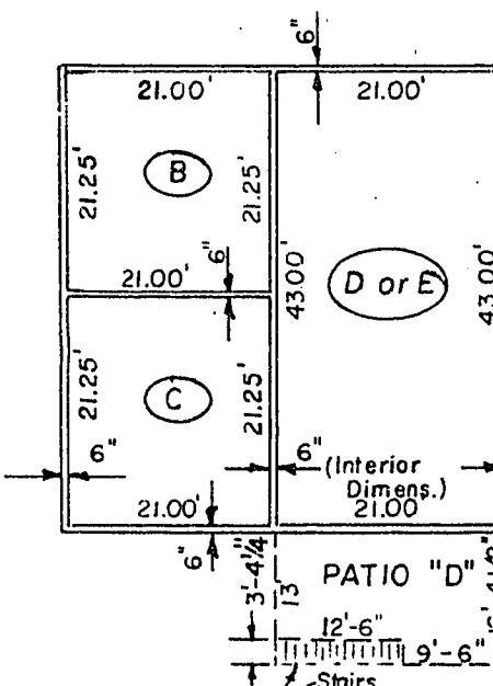
2ND FLOOR PLAN (REVERSED UNITS)
