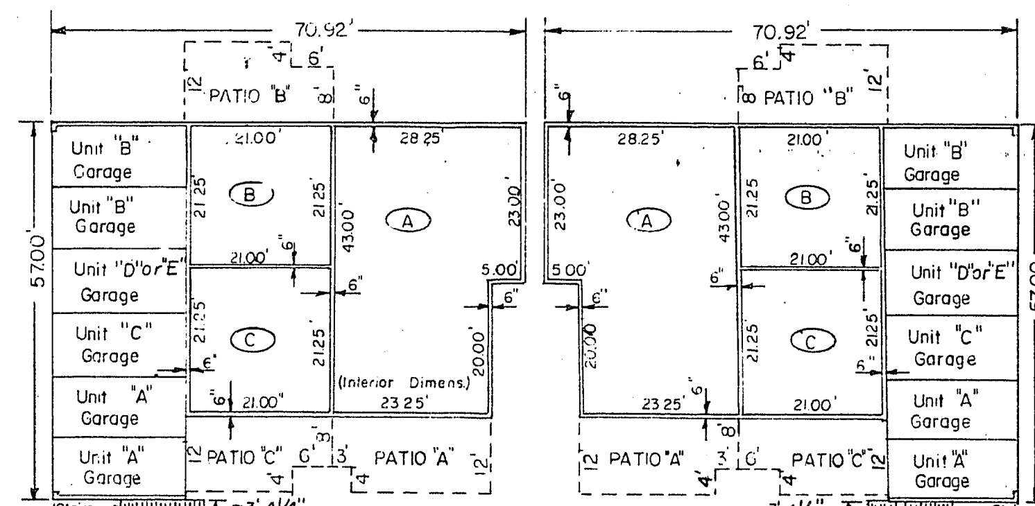
FIRST FLOOR PLAN (REGULAR UNITS)
