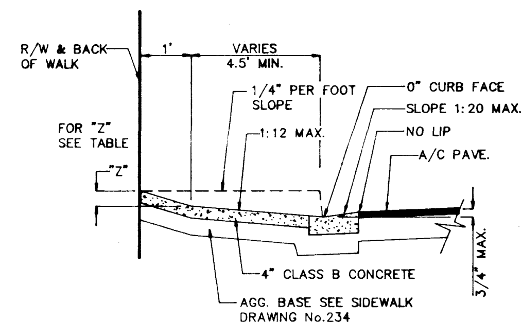
SECTION
