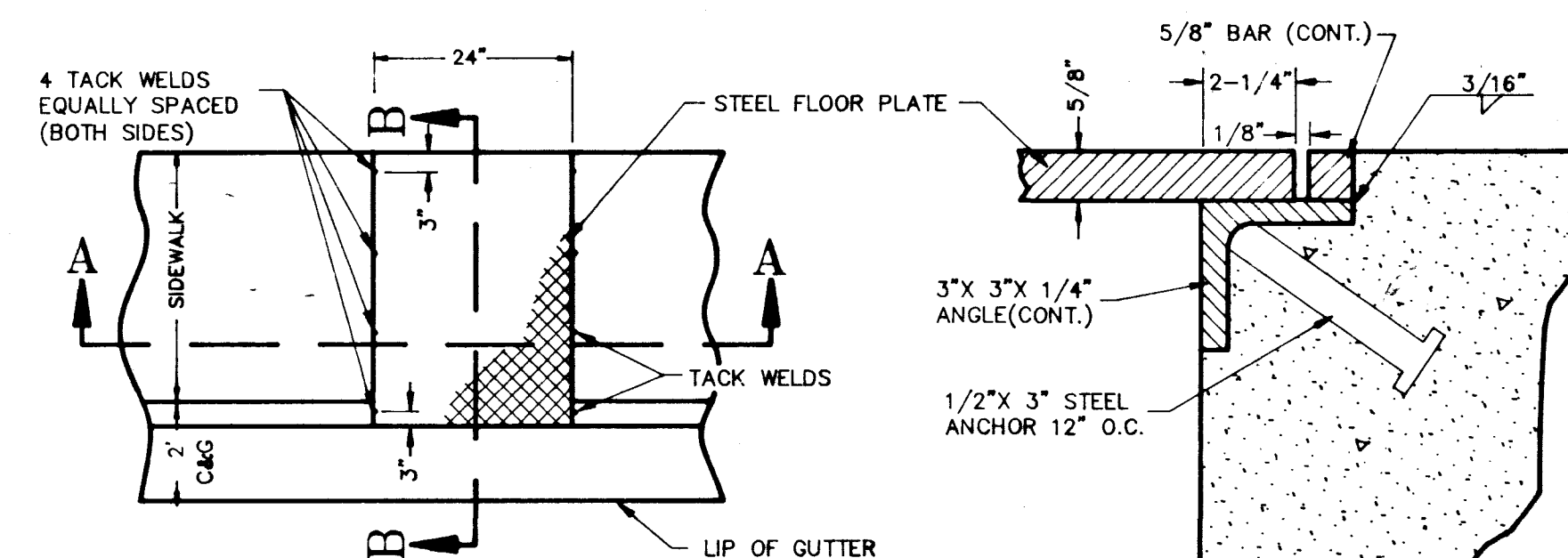
PLAN
