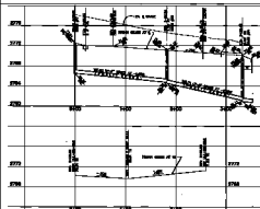
PROFILE 'A' - CUL-DE-SAC
