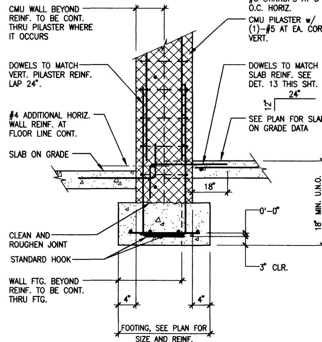
MASONRY PILASTER
