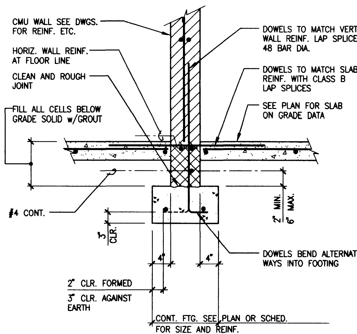
INTERIOR CMU WALL FOOTING
