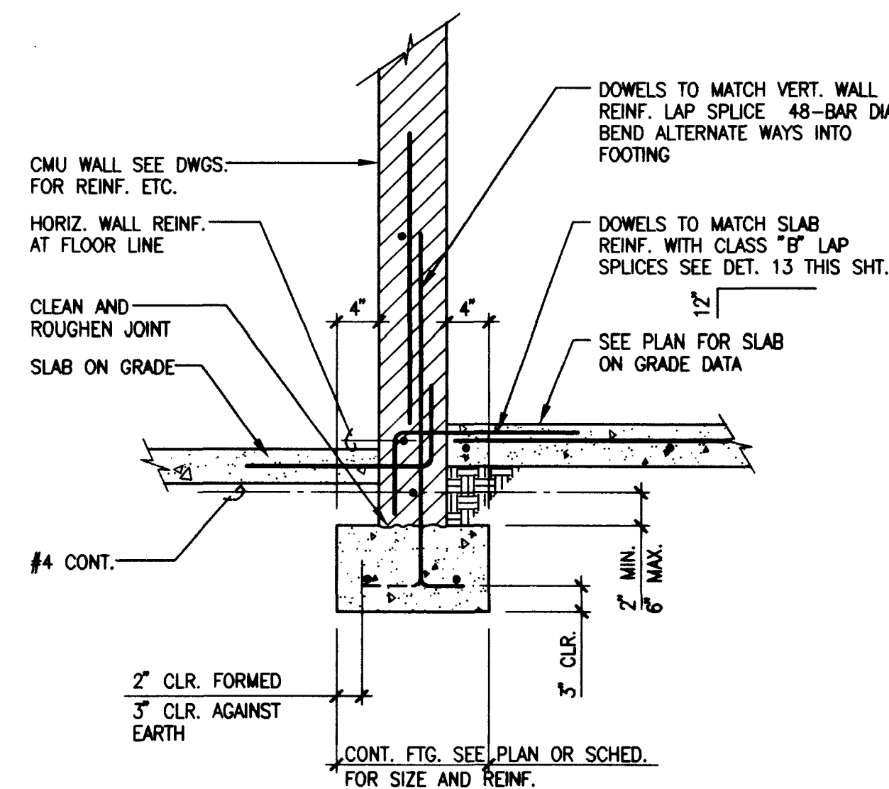
EXTERIOR WALL FOOTING
