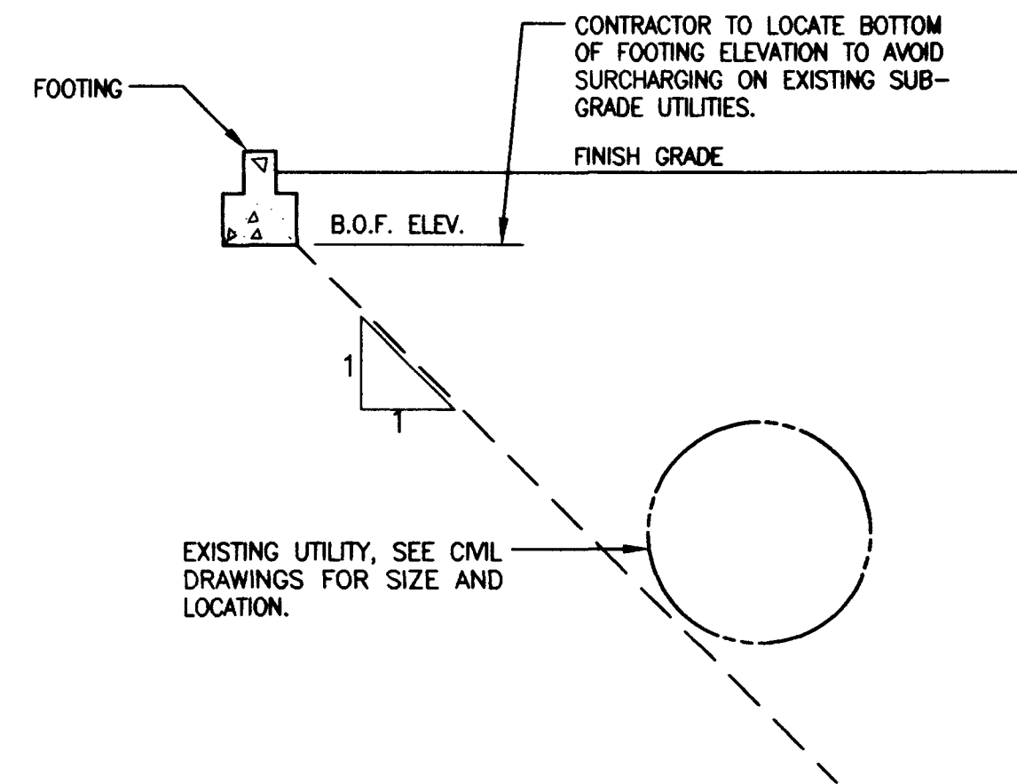
FOOTING PARALLEL TO EXISTING UTILITY
