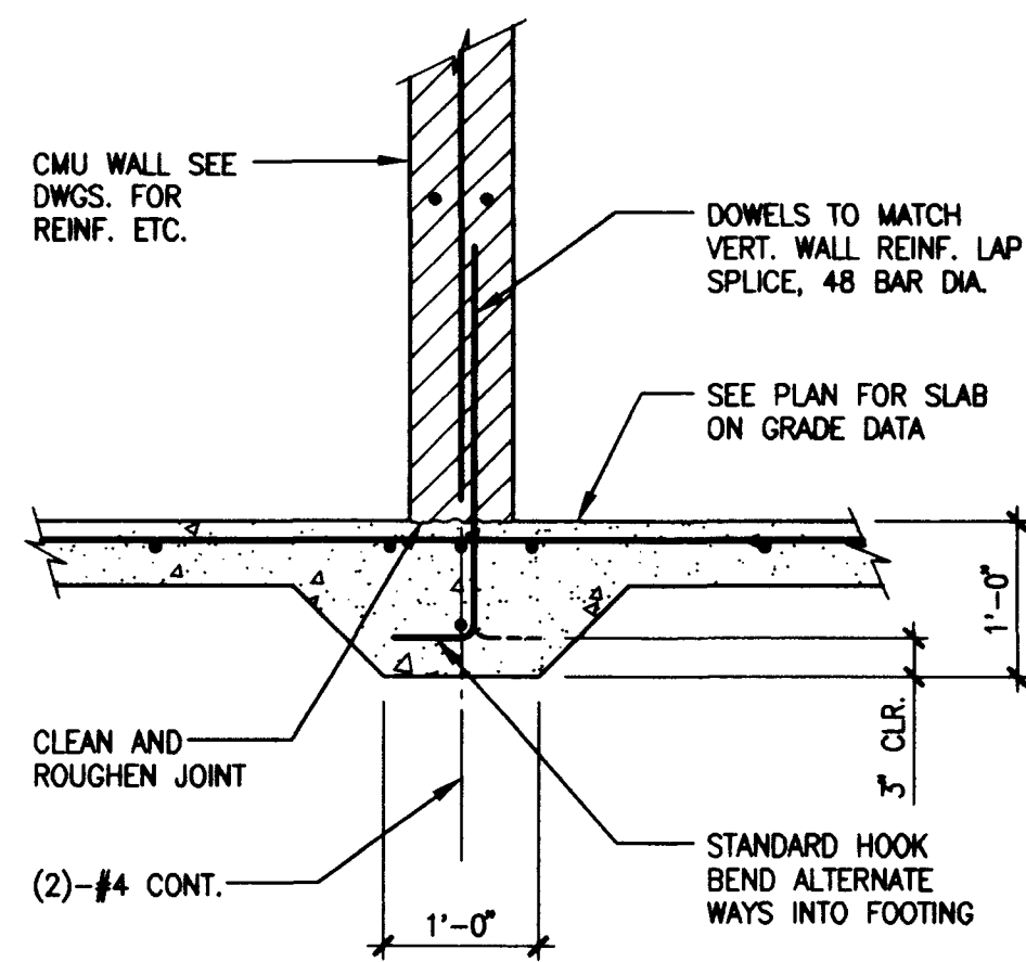
THICKENED SLAB AT NON-BEARING MASONRY WALL
