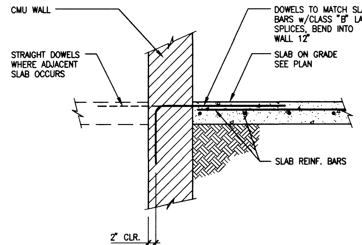
DOWELS TO SLAB
