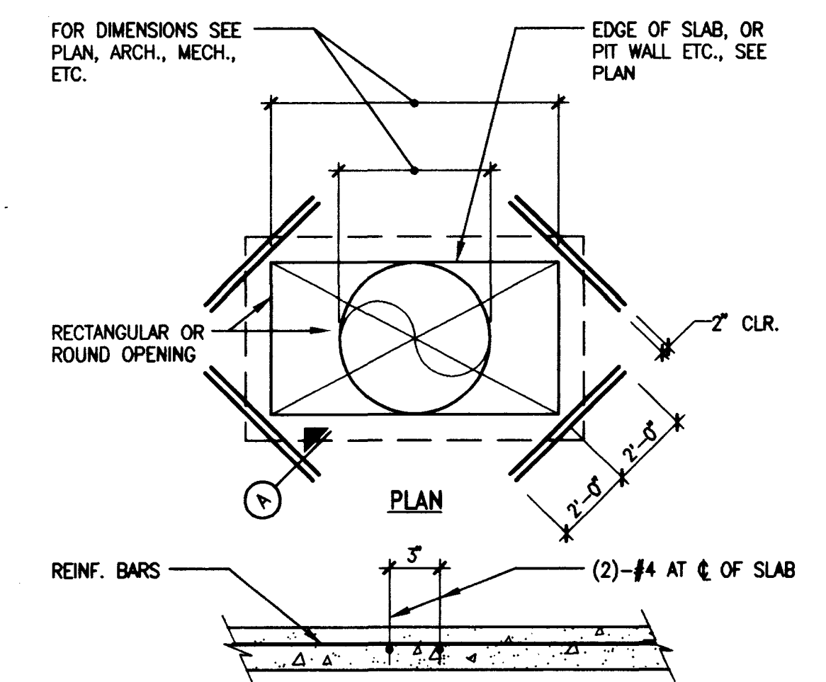
DETAIL 13
