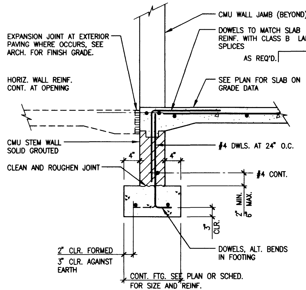
FOOTING AT WALL OPENING
