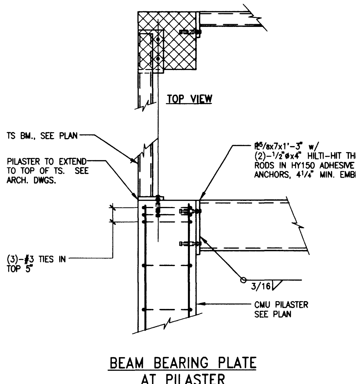
DETAIL 12
