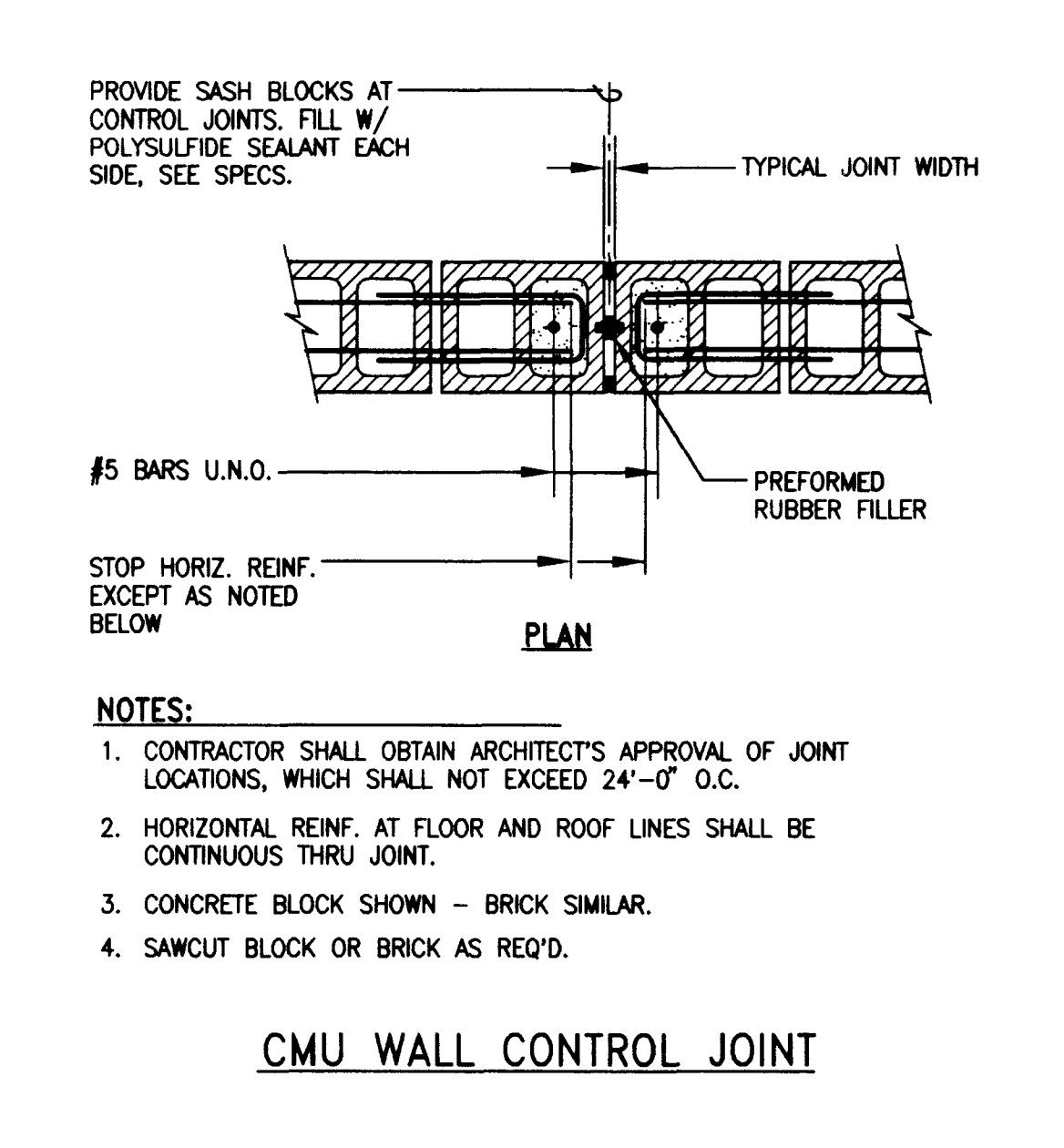
DETAIL 6
