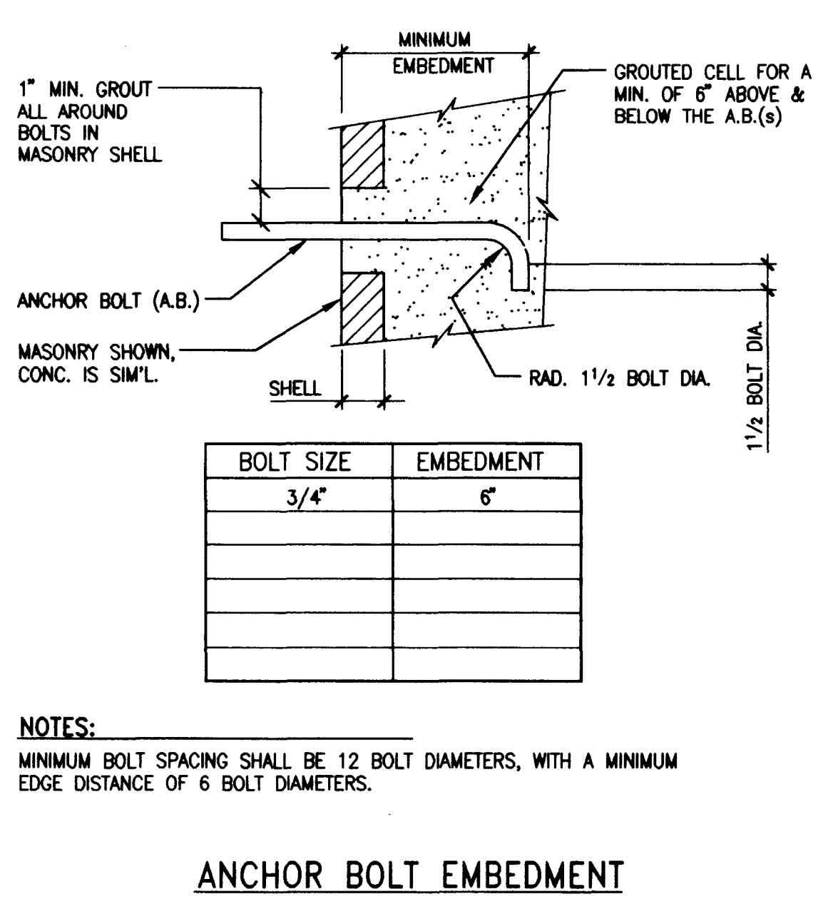
DETAIL 1
