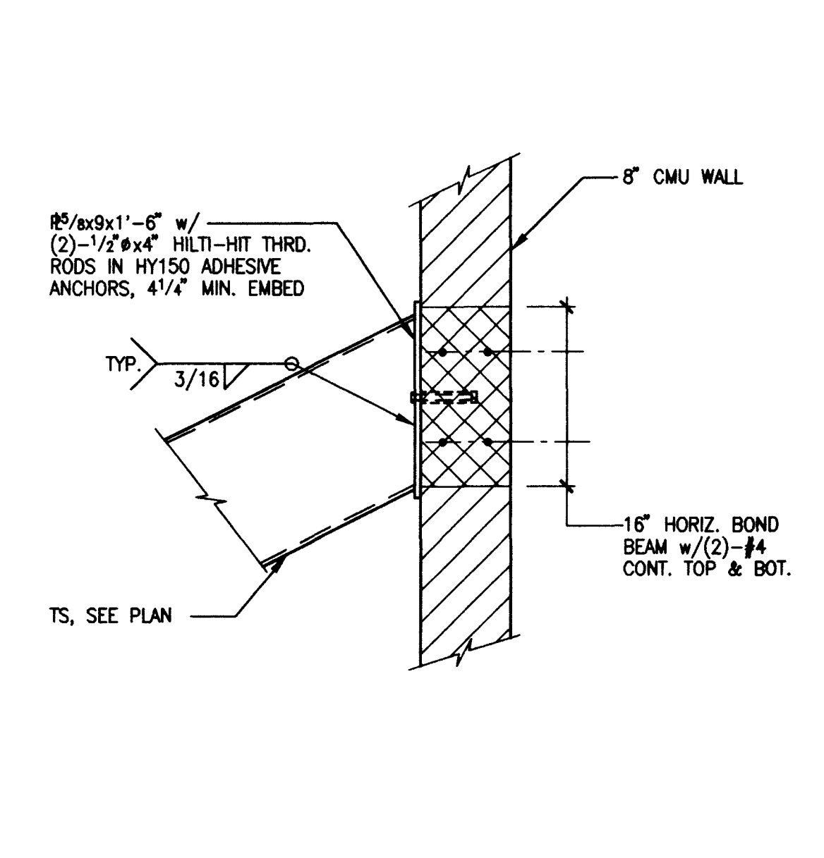
DETAIL 13
