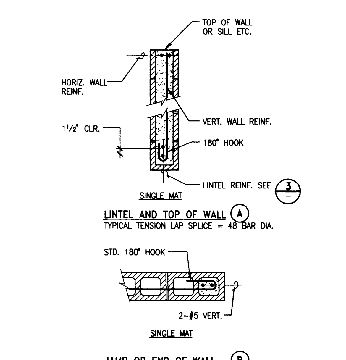
DETAIL 4
