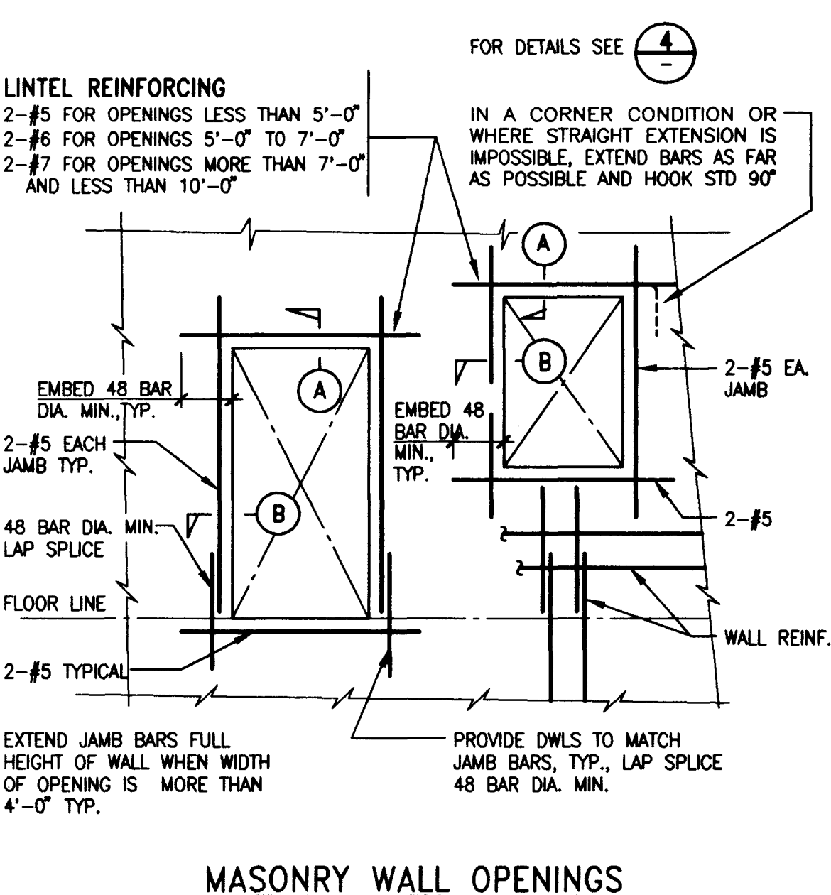
DETAIL 3
