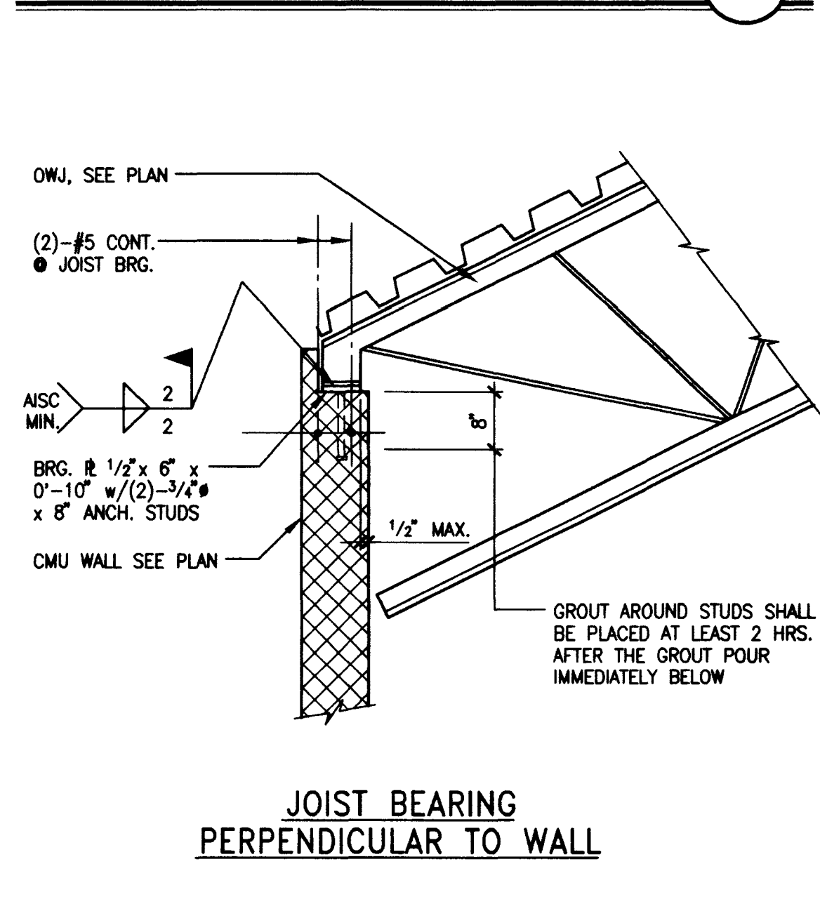
DETAIL 11
