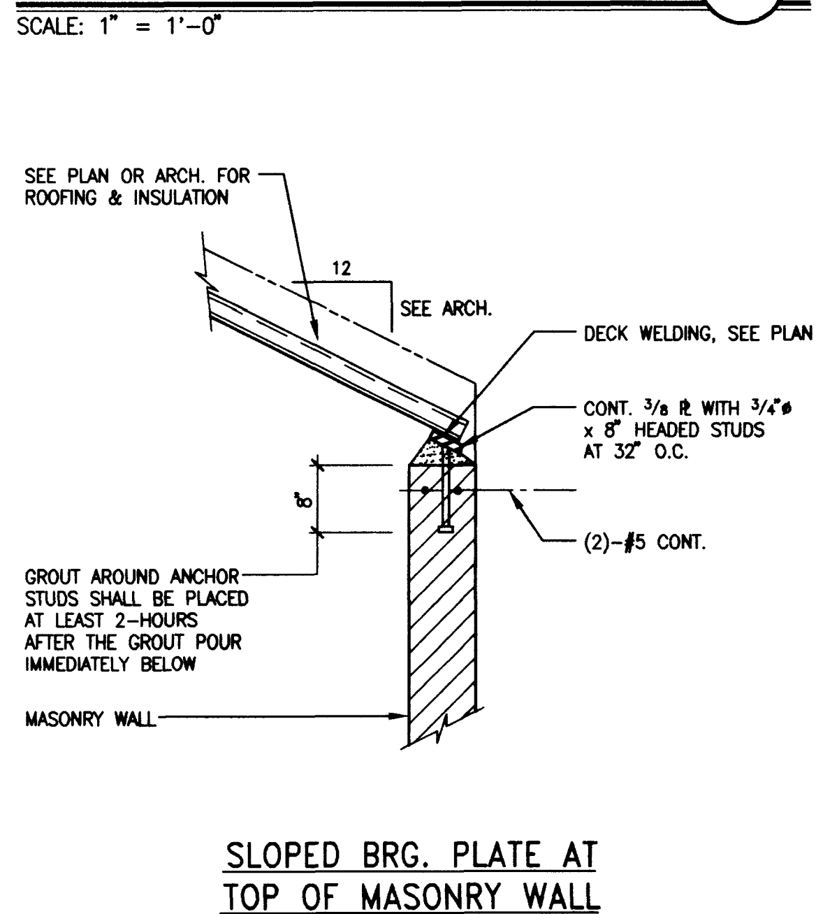
DETAIL 14
