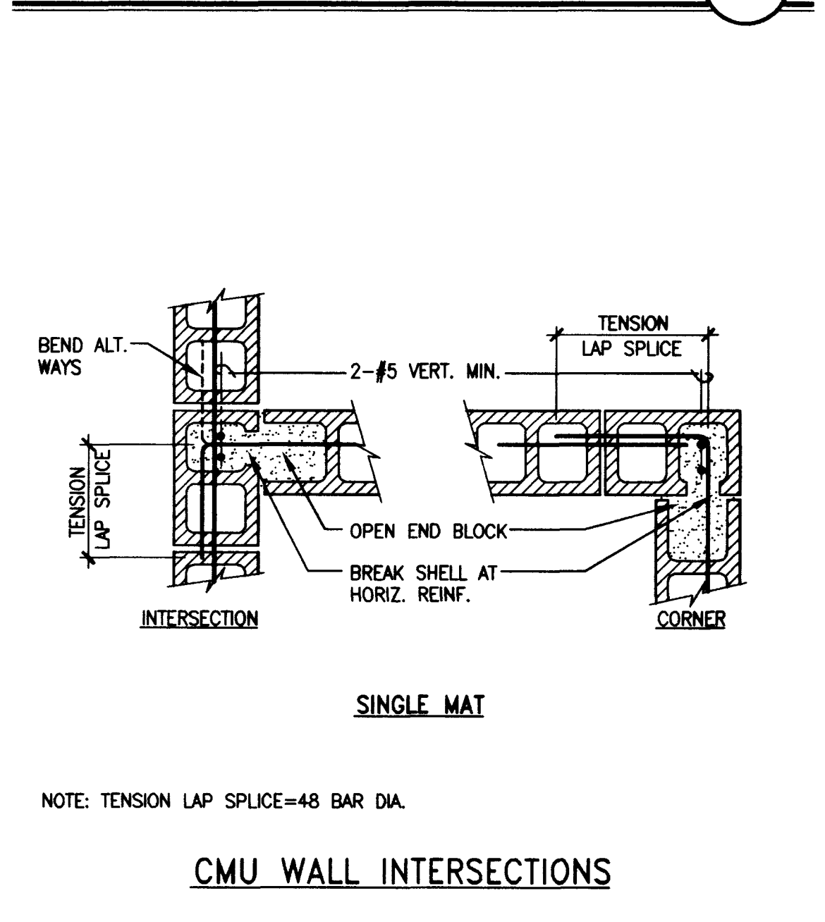
DETAIL 5
