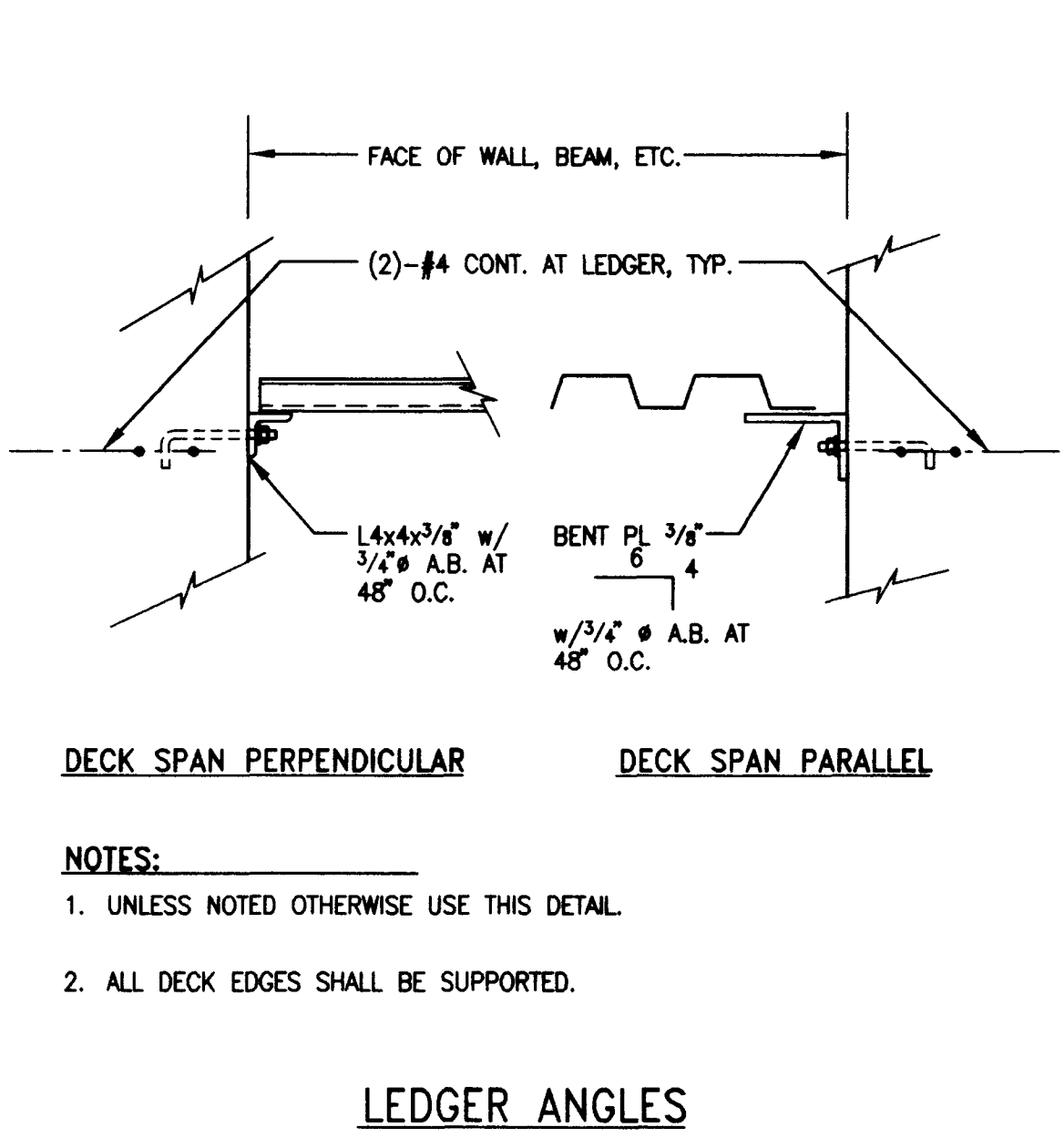
DETAIL 9
