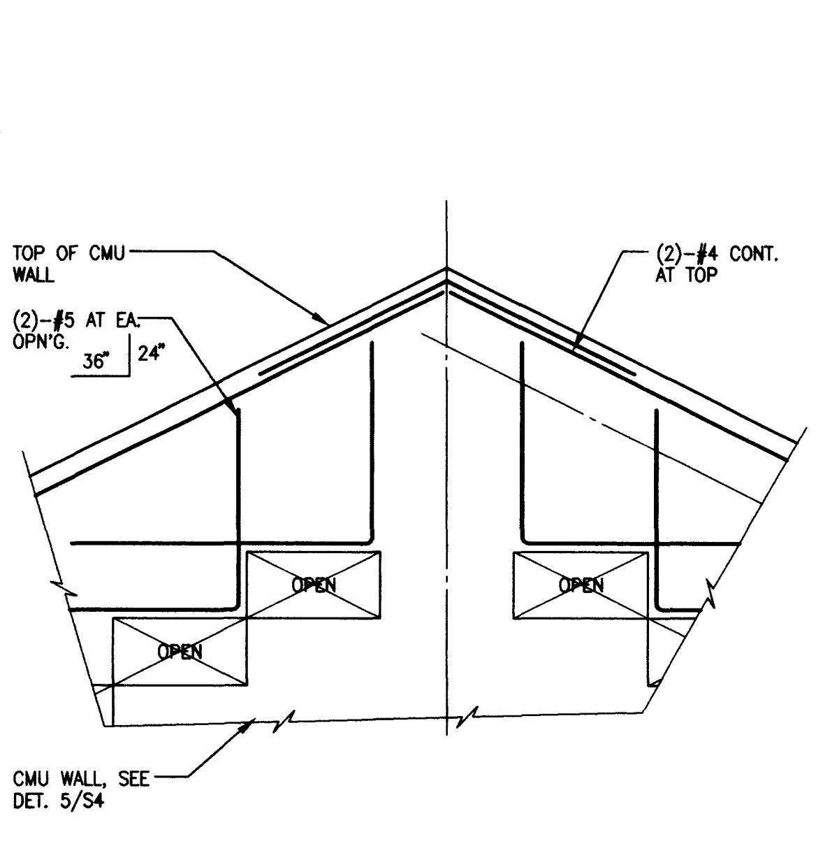
DETAIL 7
