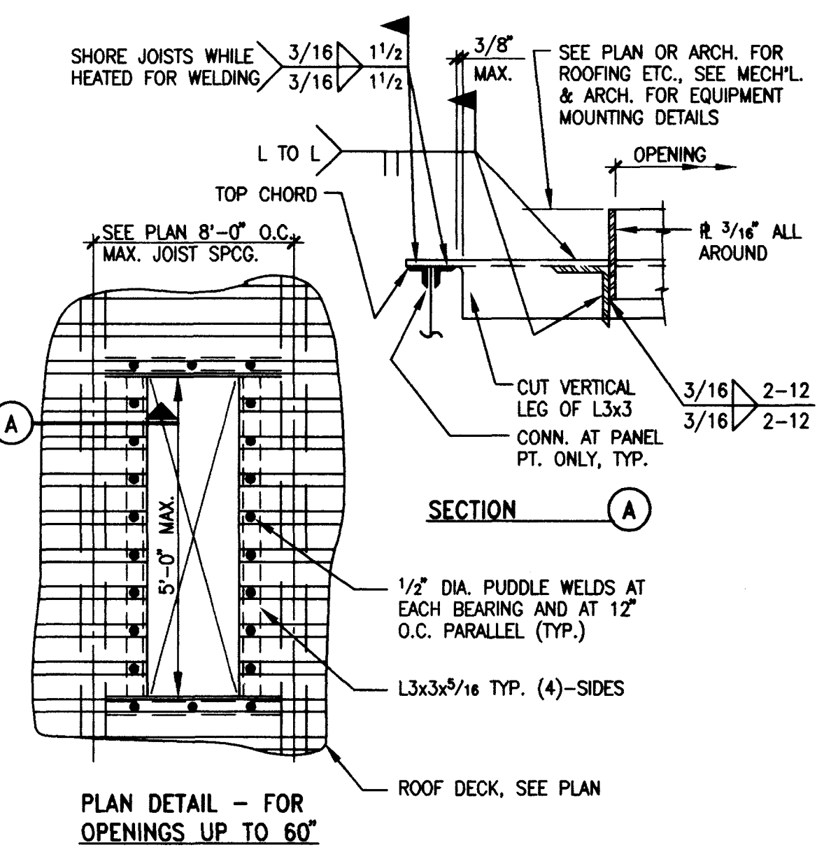
DETAIL 10
