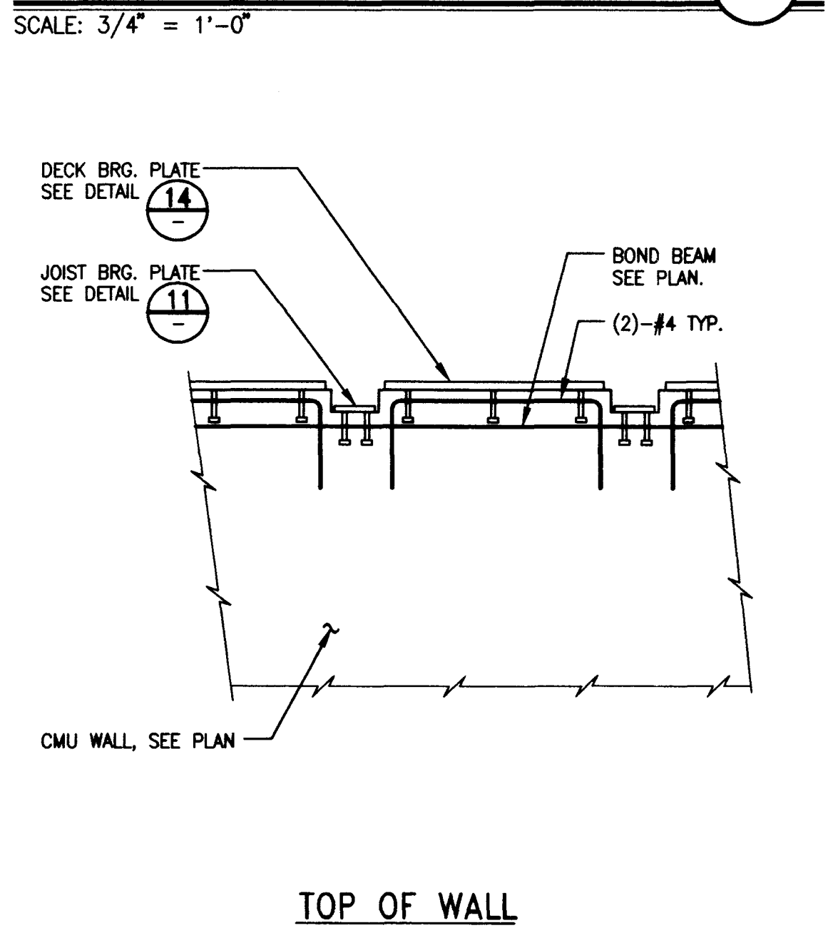
DETAIL 8
