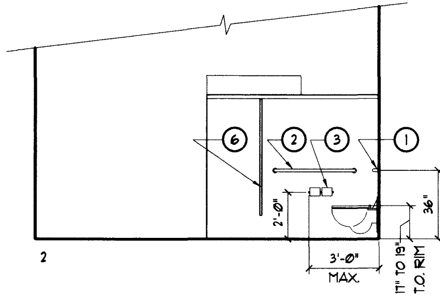
MENS RM. 103 OPPOSITE HAND OF WOMENS RM. 101 - SIM.
