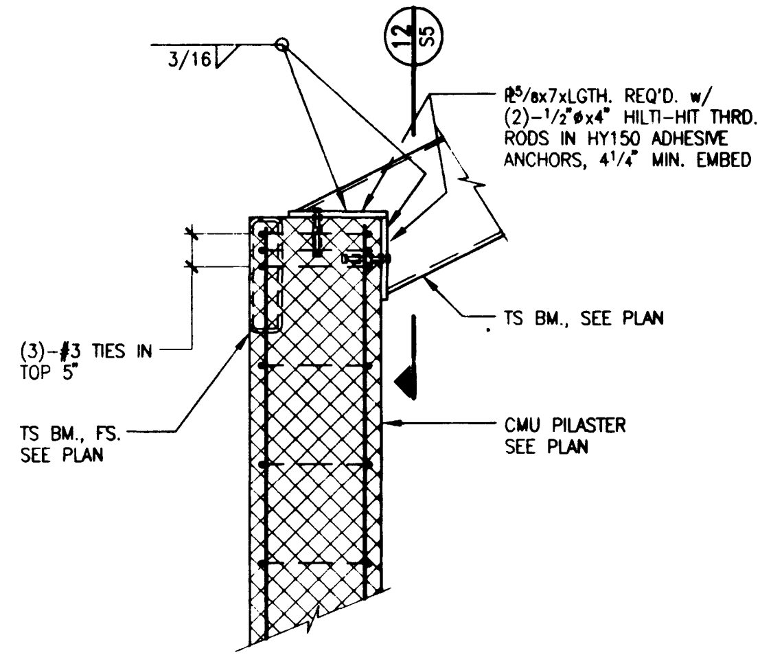
BEAM BEARING PLATE AT PILASTER
