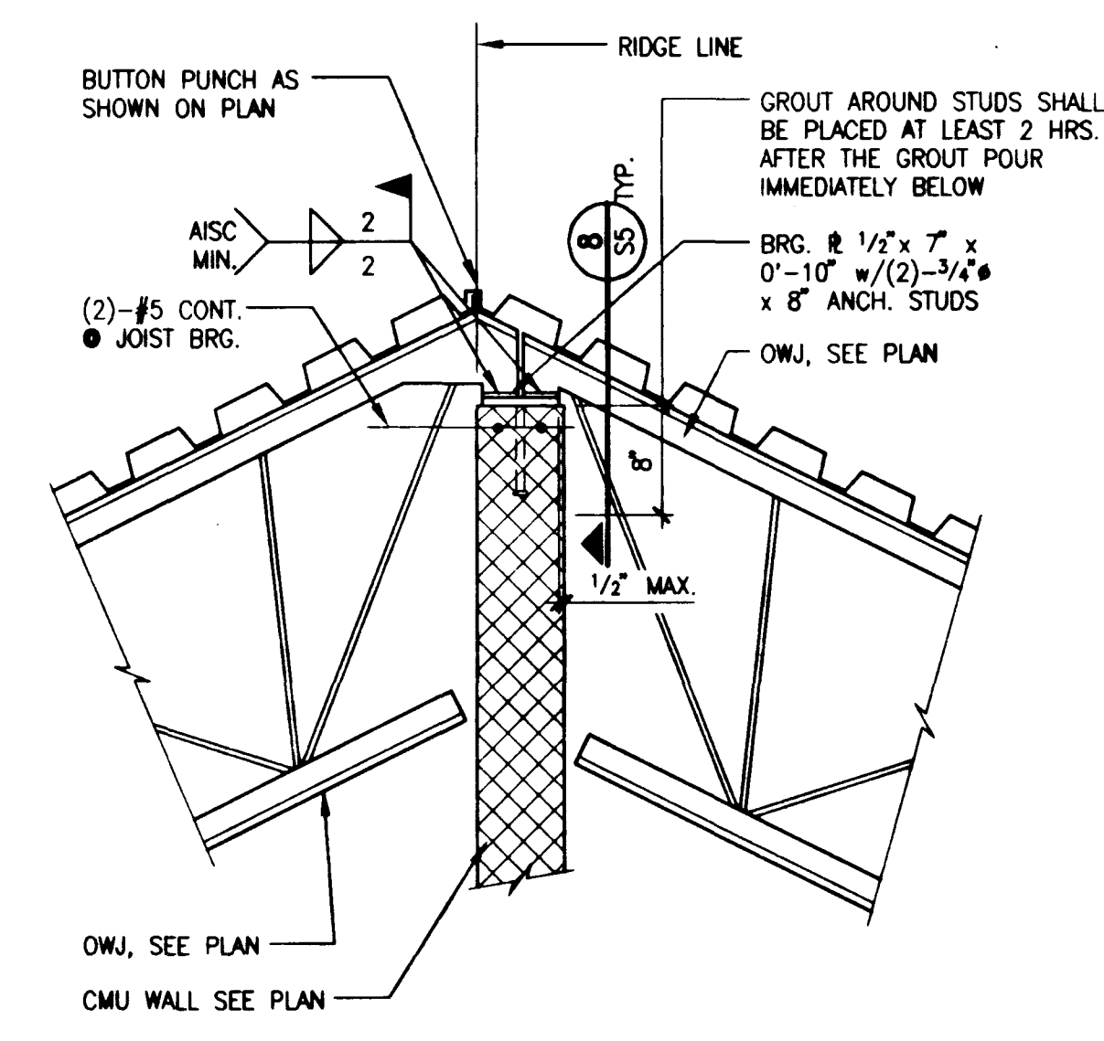
JOIST BEARING ON WALL AT RIDGE LINE
