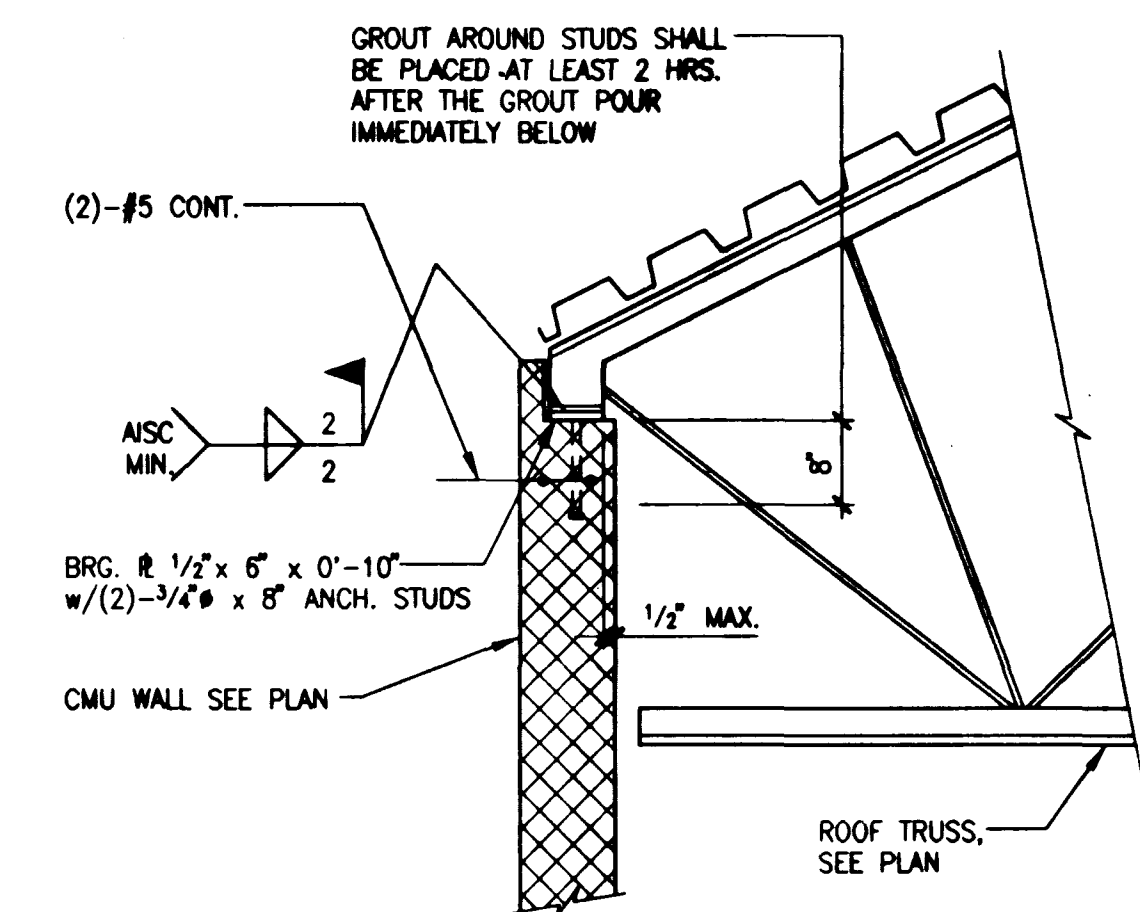
JOIST BEARING PERPENDICULAR TO WALL
