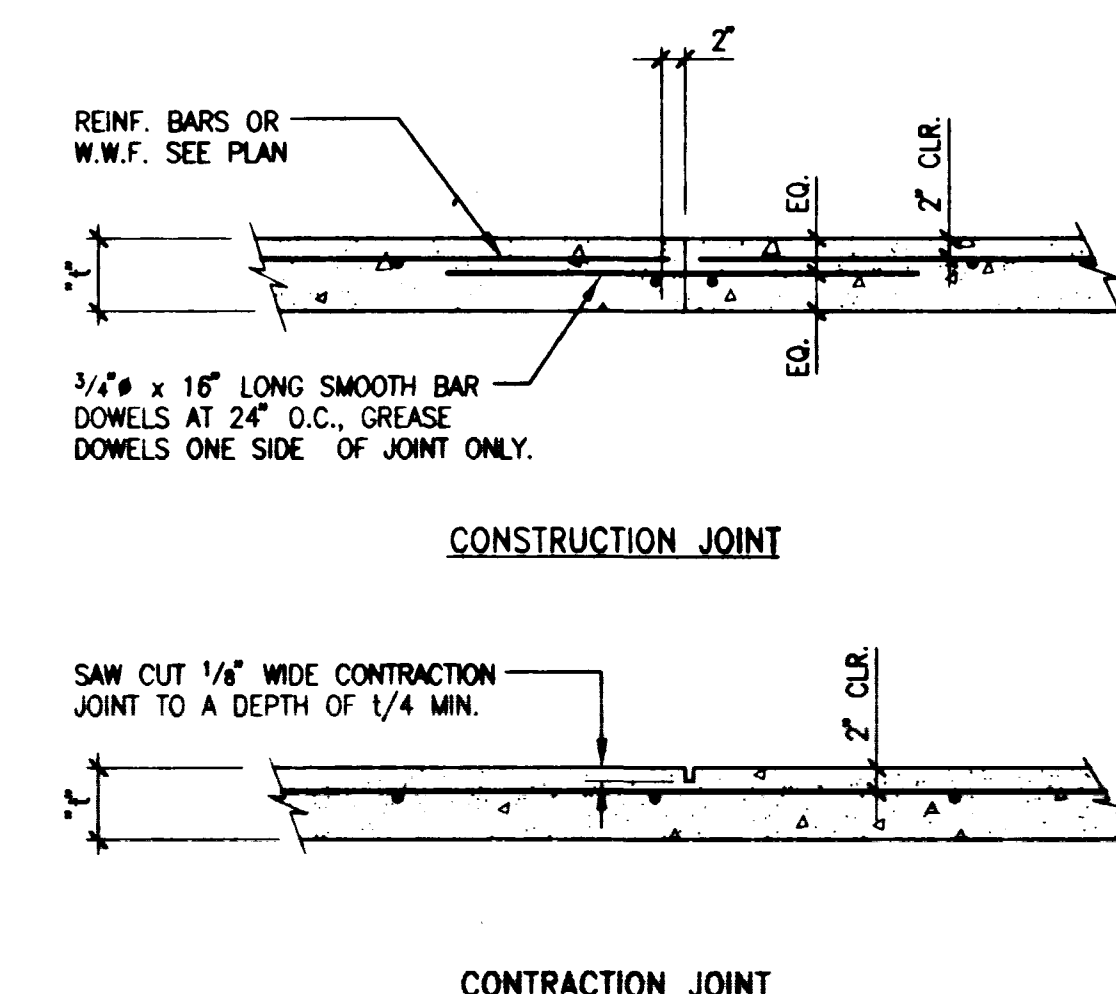
JOINTS IN SLAB ON GRADE
