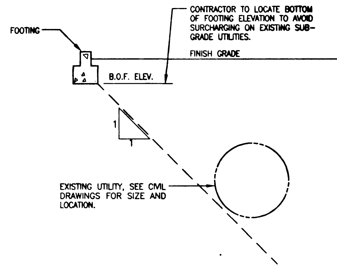
FOOTING PARALLEL TO EXISTING UTILITY
