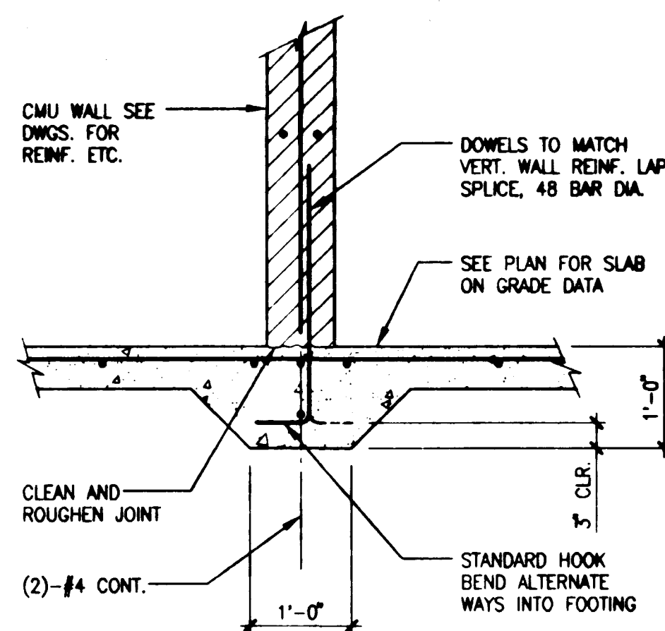
THICKENED SLAB AT NON-BEARING MASONRY WALL
