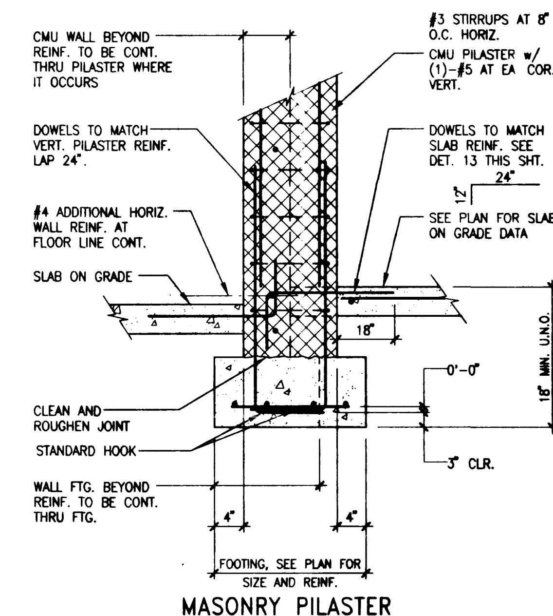
MASONRY PILASTER
