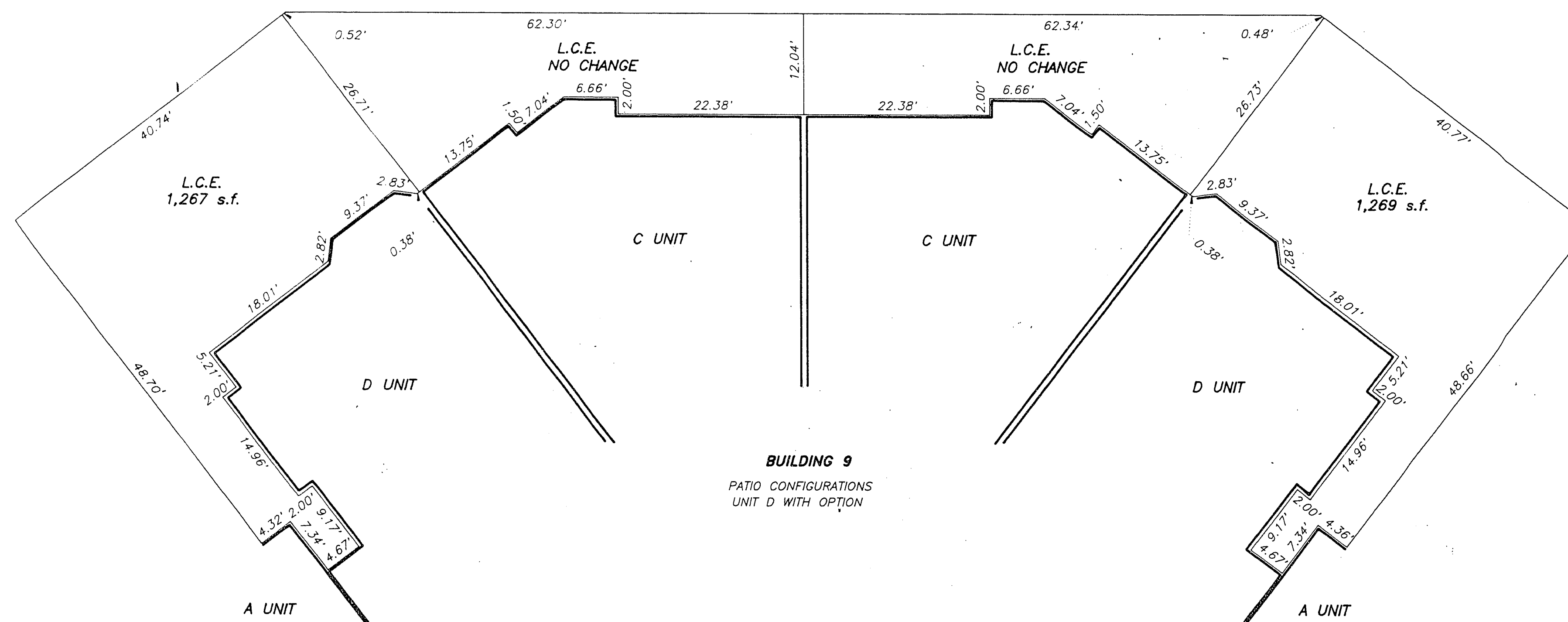
PATIO CONFIGURATIONS 8 UNIT BUILDING
