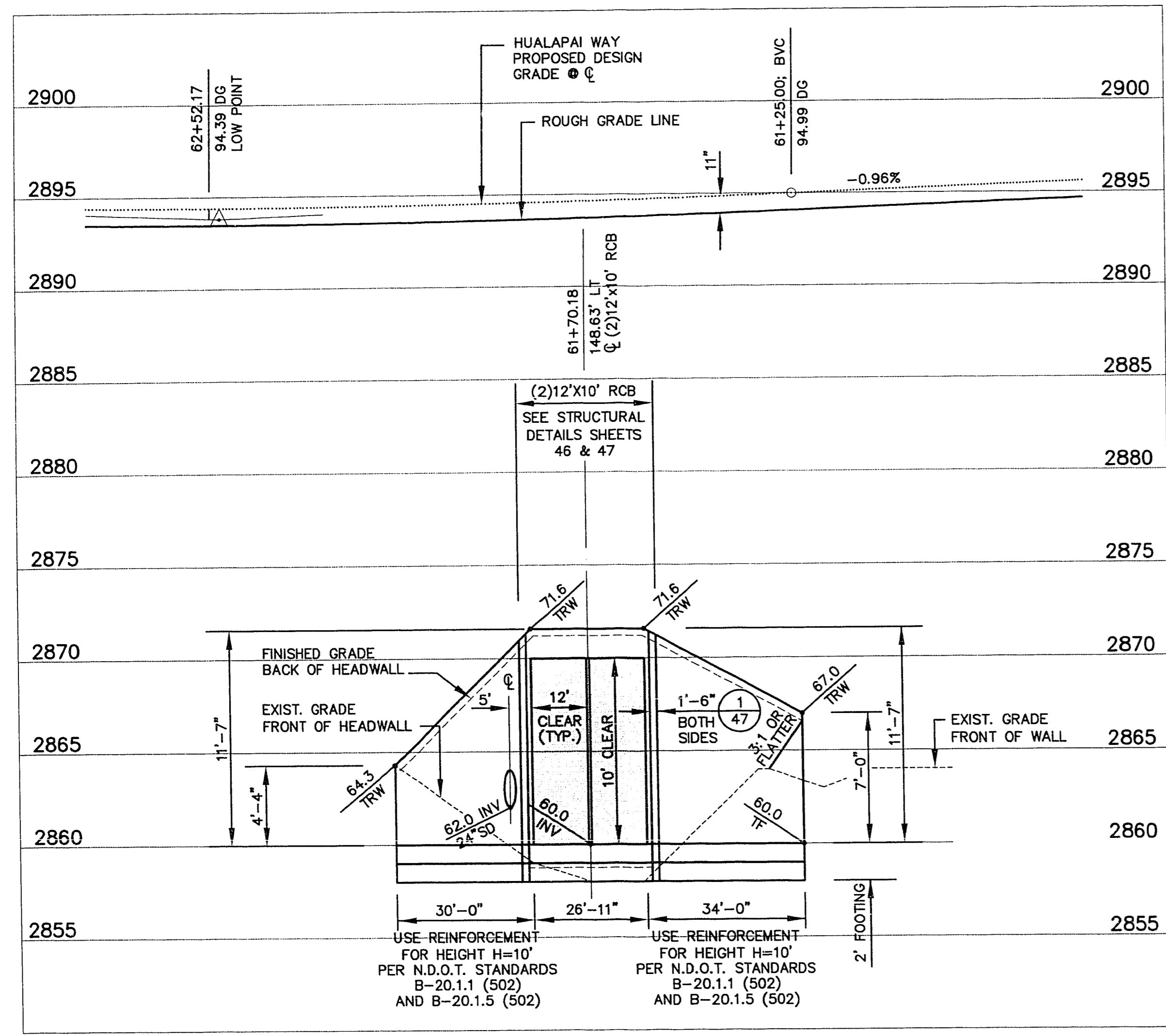
IMPROVED INLET DRAINAGE CROSSING HUALAPAI WAY HEADWALL ELEVATION - DOWN-STREAM
