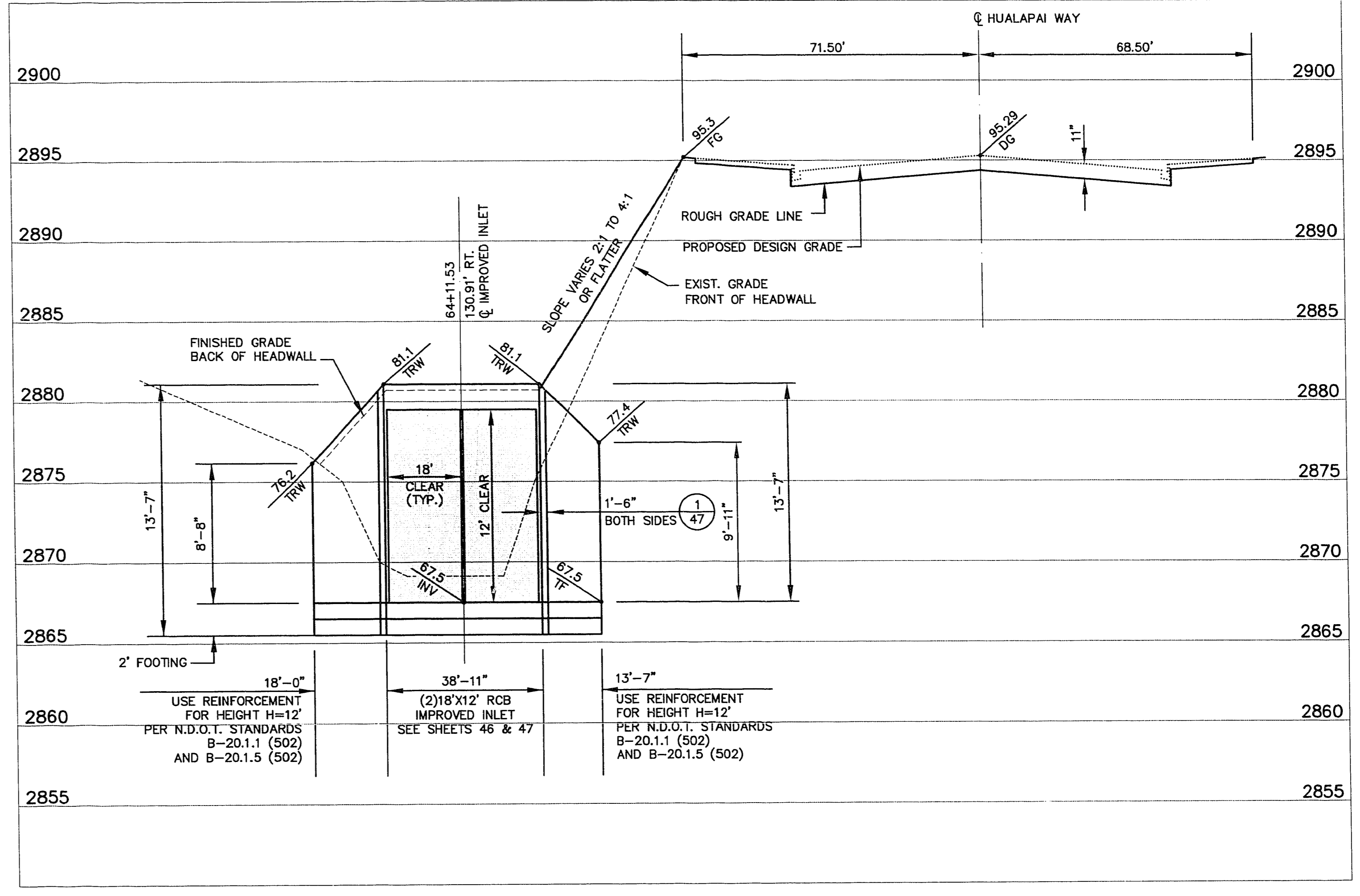
IMPROVED INLET DRAINAGE CROSSING HUALAPAI WAY HEADWALL ELEVATION - UP-STREAM
