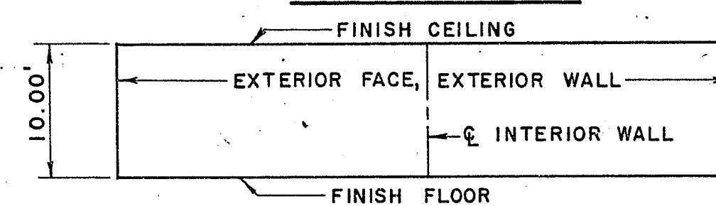
SECTION E-E
