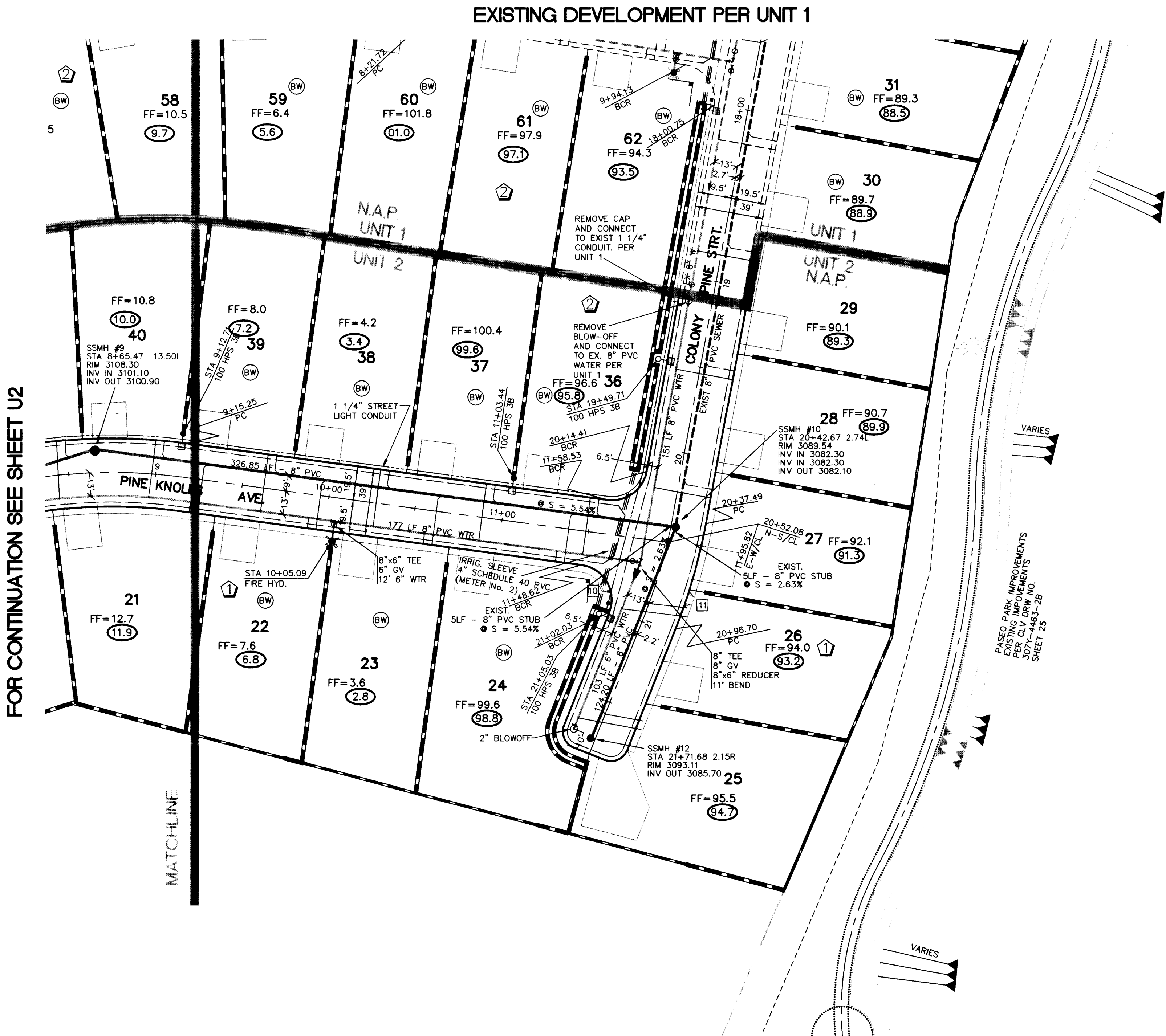
EX. SEWER CONTINUATION THROUGH VILLAGE 8
