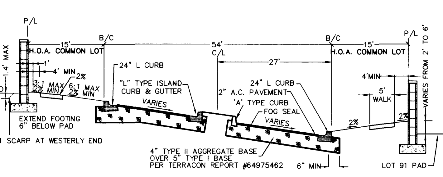
SECTION B - PARCEL ENTRY
