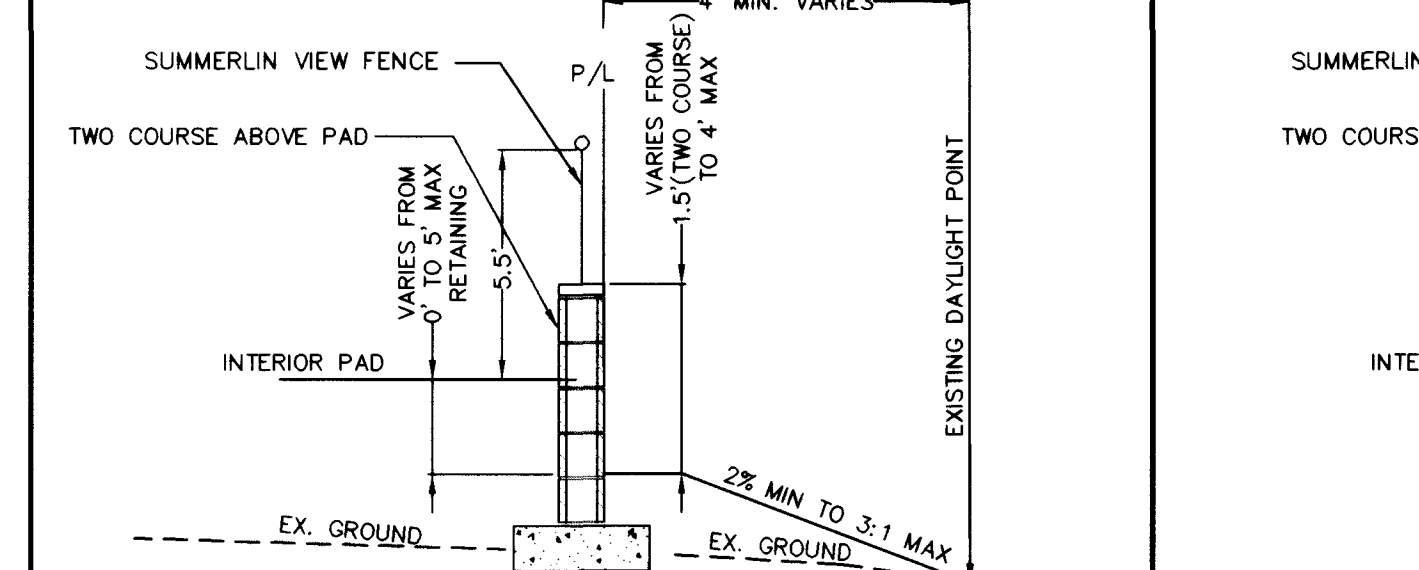
SECTION D - PASEO PARK
