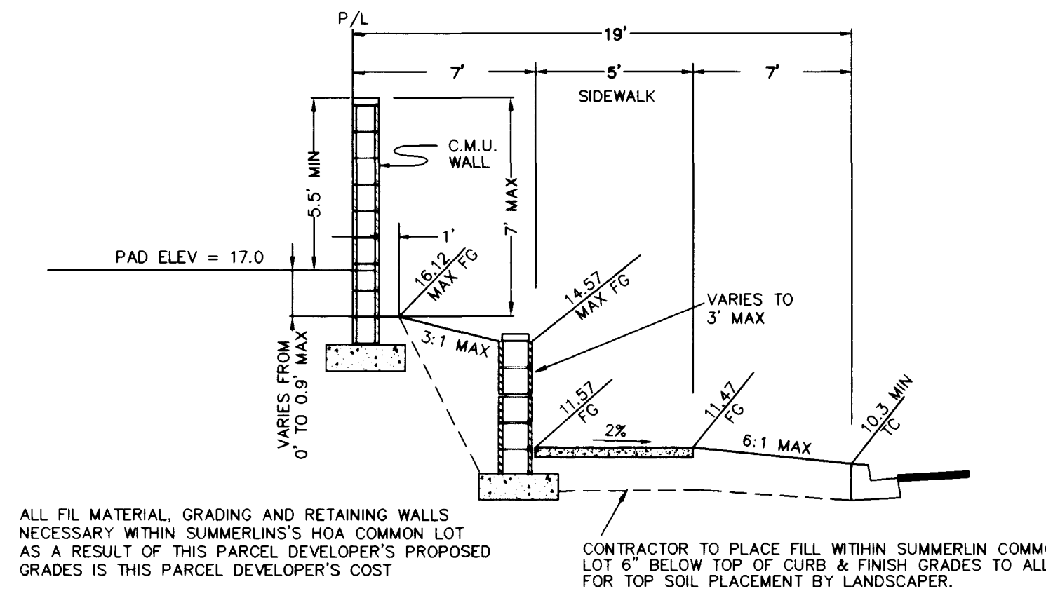
SECTION A3 - SAGEBERRY DRIVE
