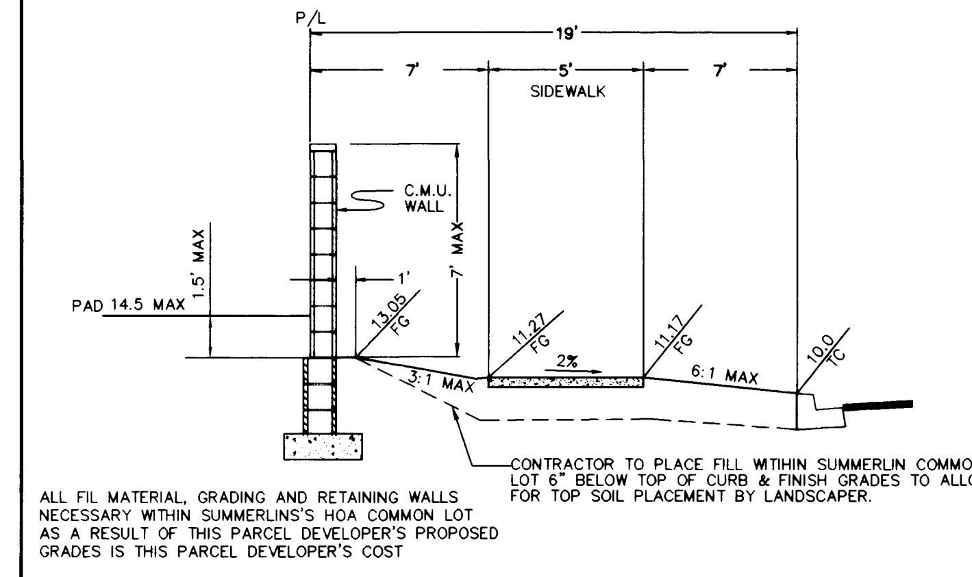
SECTION A2 - SAGEBERRY DRIVE
