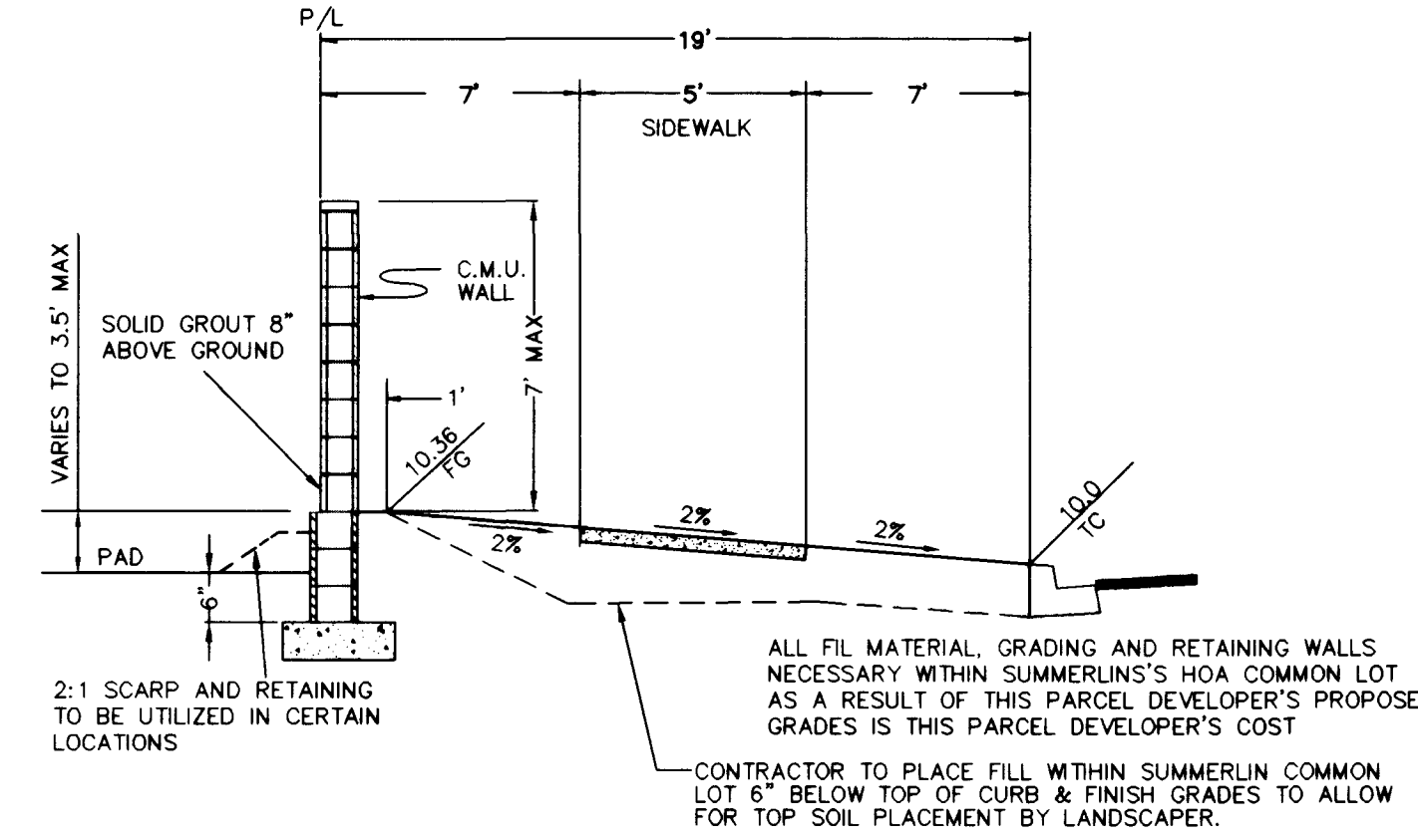
SECTION A1 - SAGEBERRY DRIVE
