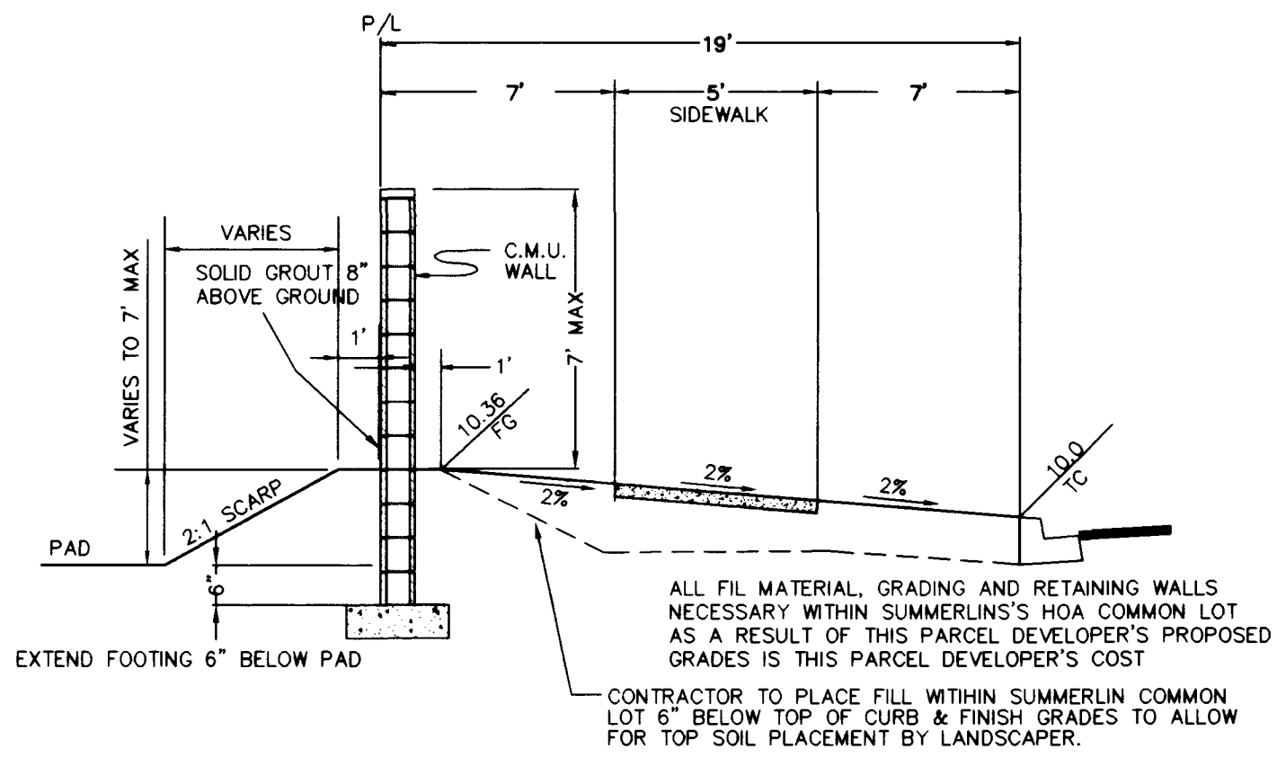
SECTION A - SAGEBERRY DRIVE
