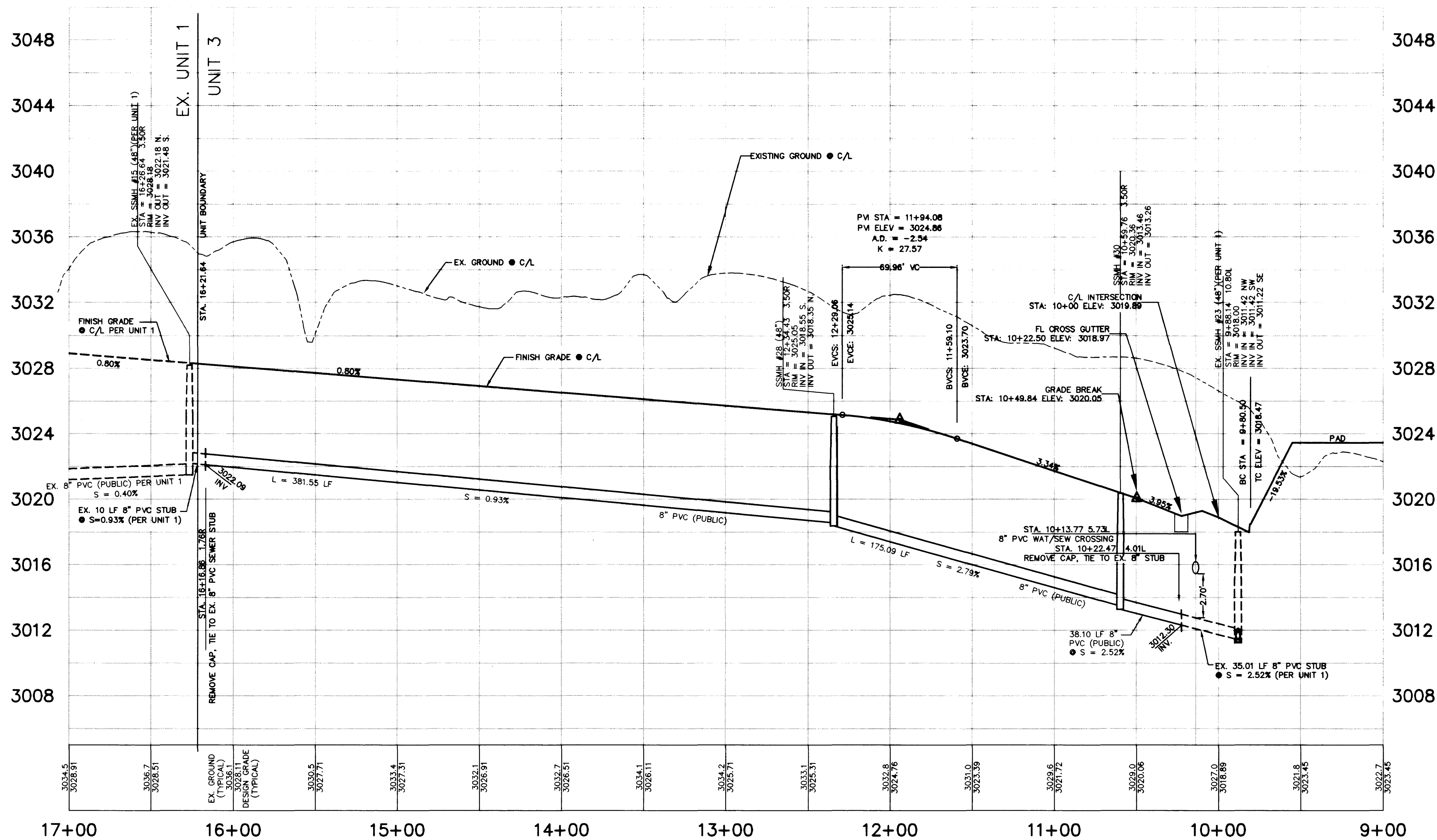
REISLING COURT PROFILE (PUBLIC SEWER & PRIVATE DRIVE)
