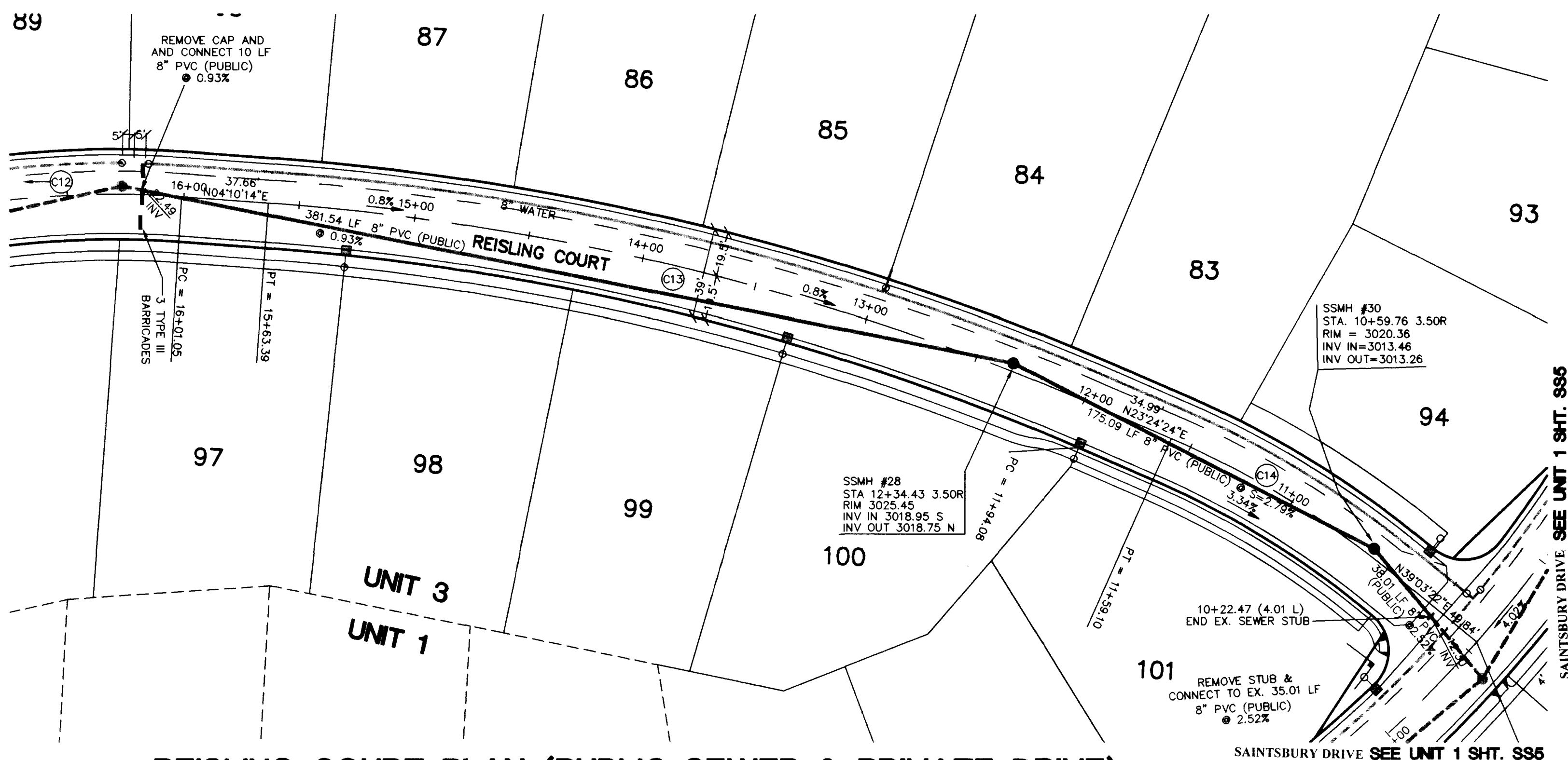
REISLING COURT PLAN (PUBLIC SEWER & PRIVATE DRIVE)
