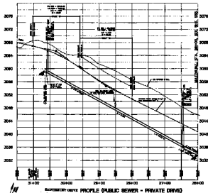
BANTERSBY DRIVE PROFILE (PUBLIC SEWER - PRIVATE DRIVE)
