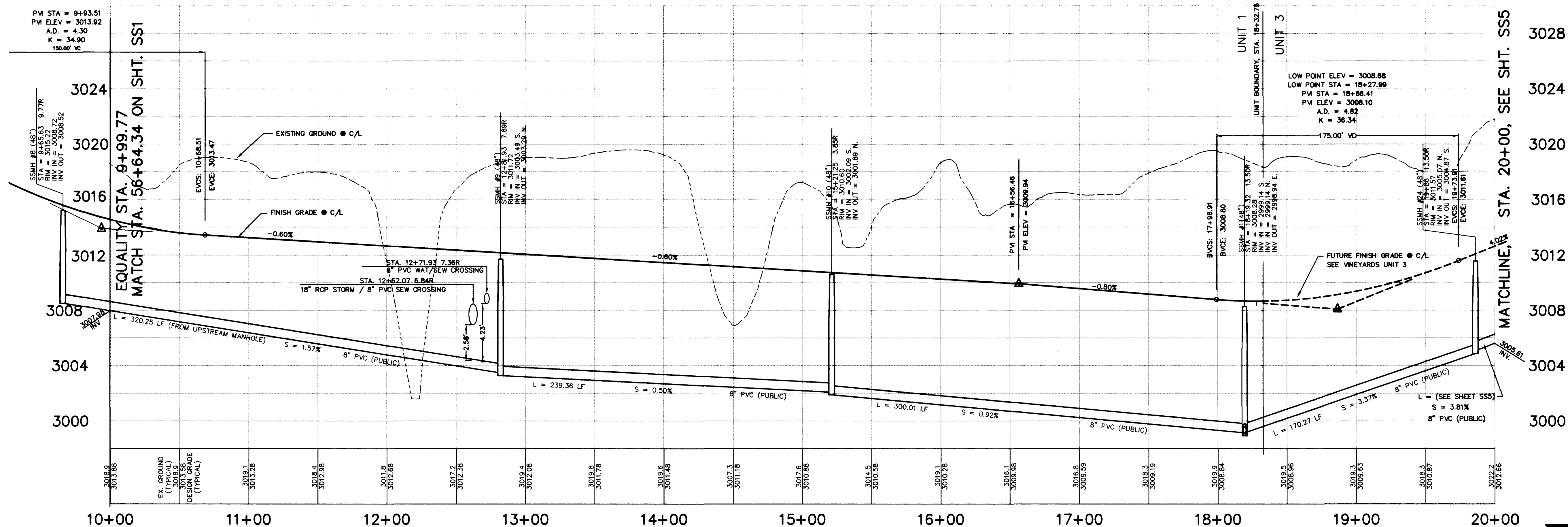
SAINTSBURY DRIVE PROFILE (PUBLIC SEWER & PRIVATE DRIVE)
