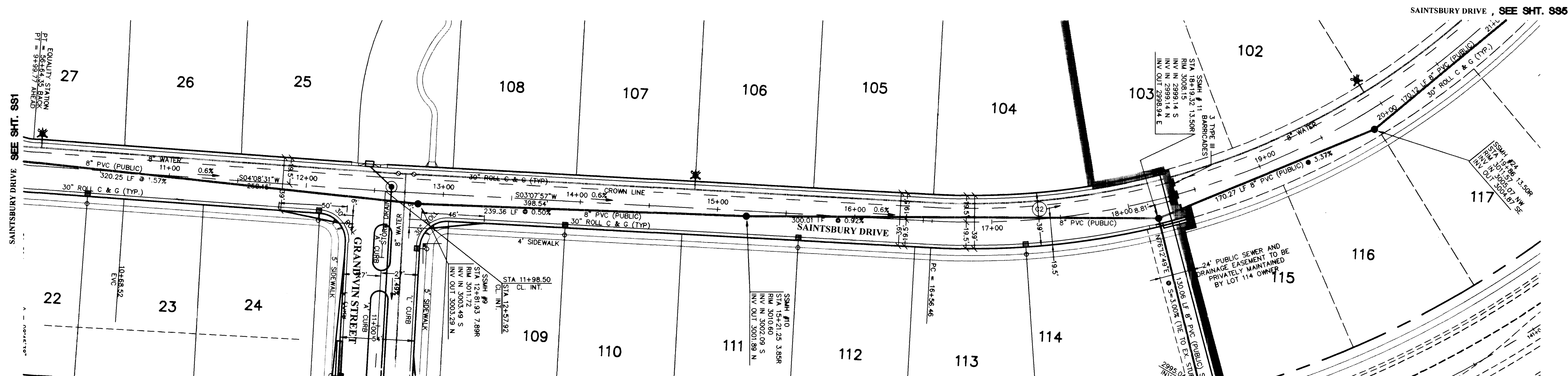
SAINTSBURY DRIVE PLAN (PUBLIC SEWER & PRIVATE DRIVE)
