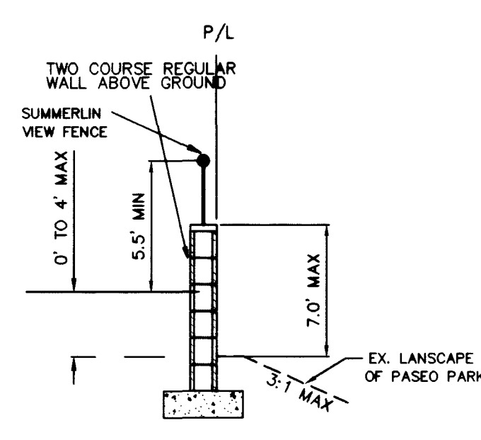
SECTION N PASEO PARK
