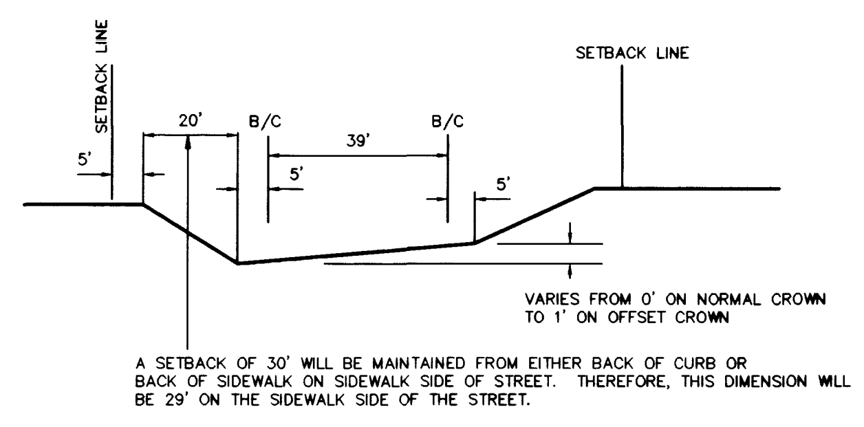
SECTION A - FAR HILLS
