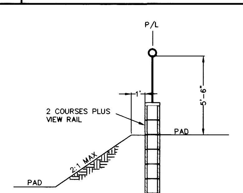
SECTION Q - FIRE DEPT. ACCESS
