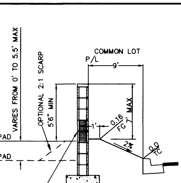
SECTION Q - FIRE DEPT. ACCESS
