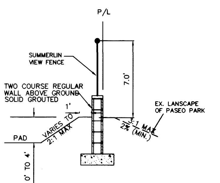
SECTION M PASEO PARK
