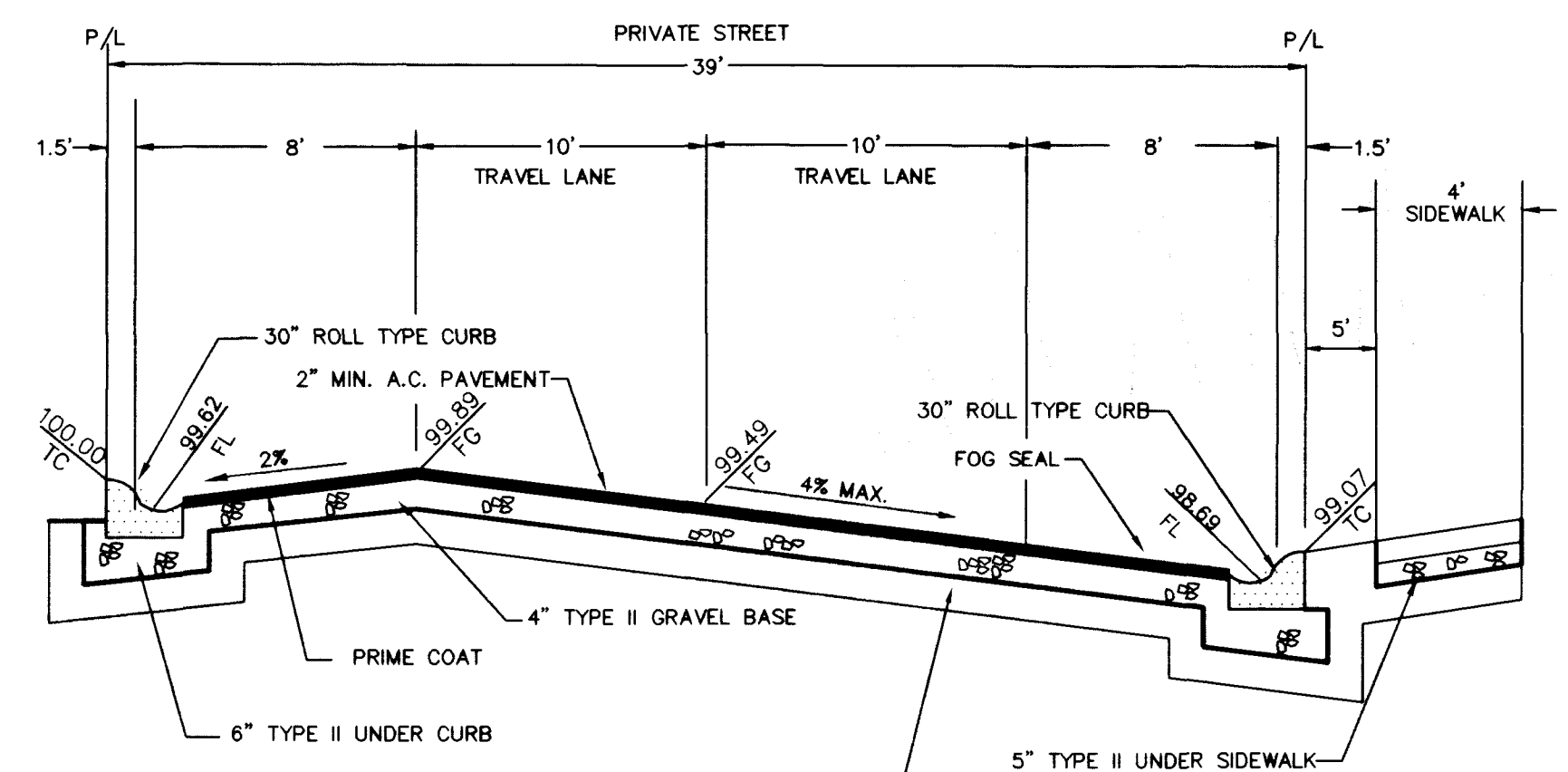
SECTION M PASEO PARK
