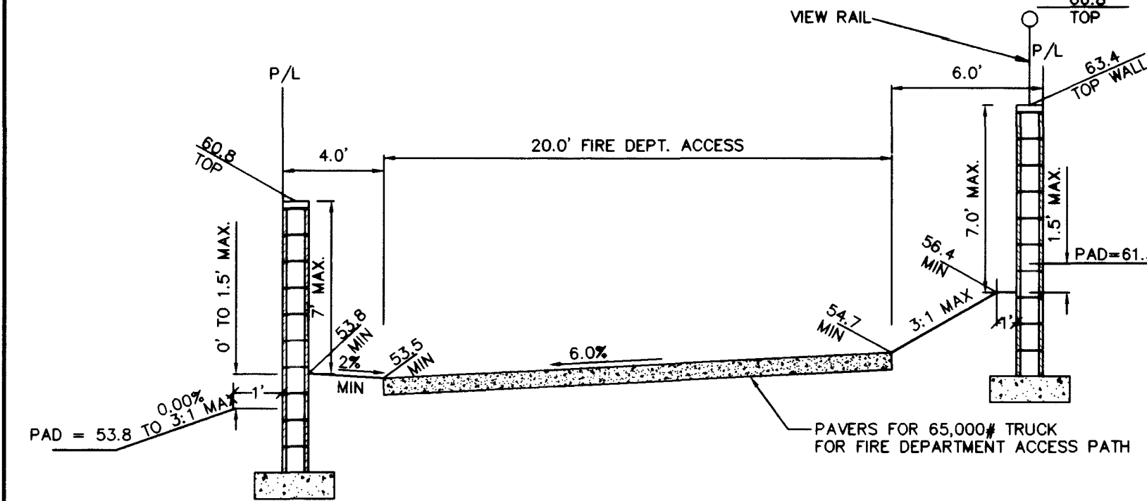
SECTION F - PED / FIRE DEPT. ACCESS
