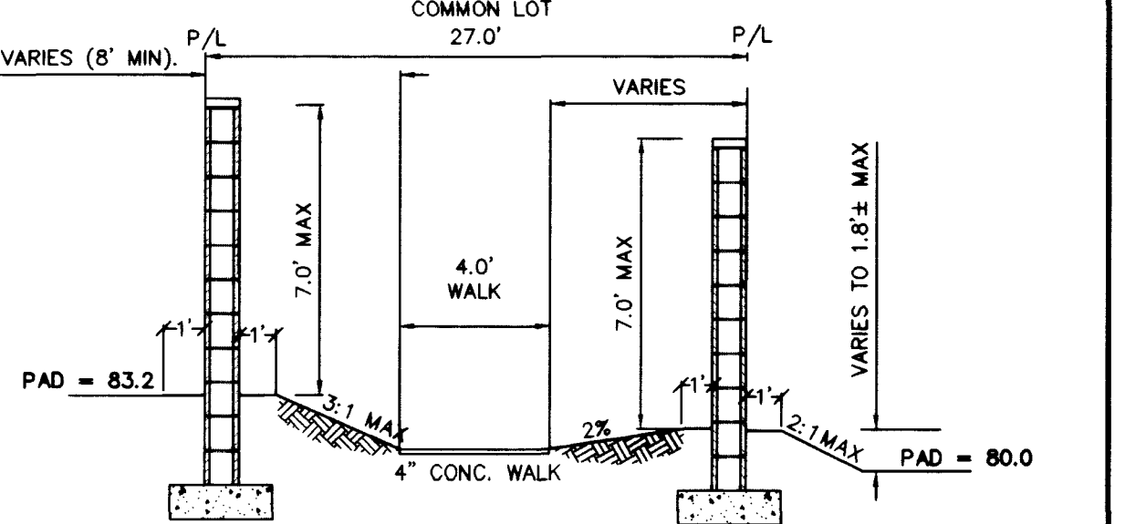
SECTION K - PED ACCESS
