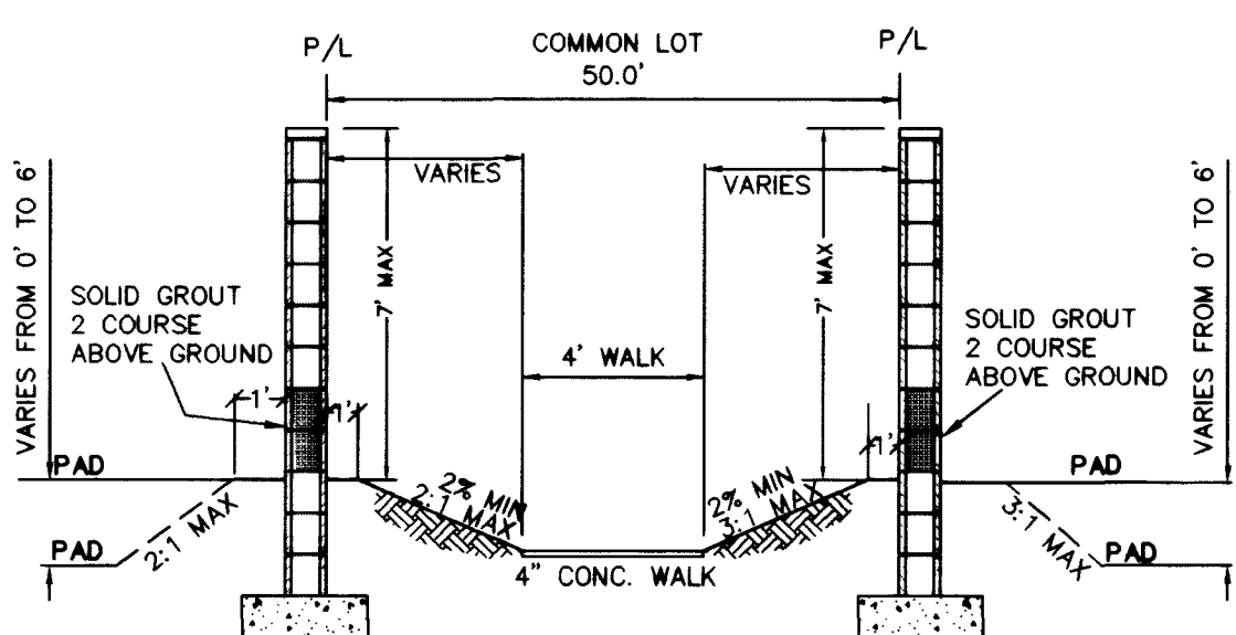
SECTION L - FINGER PARK
