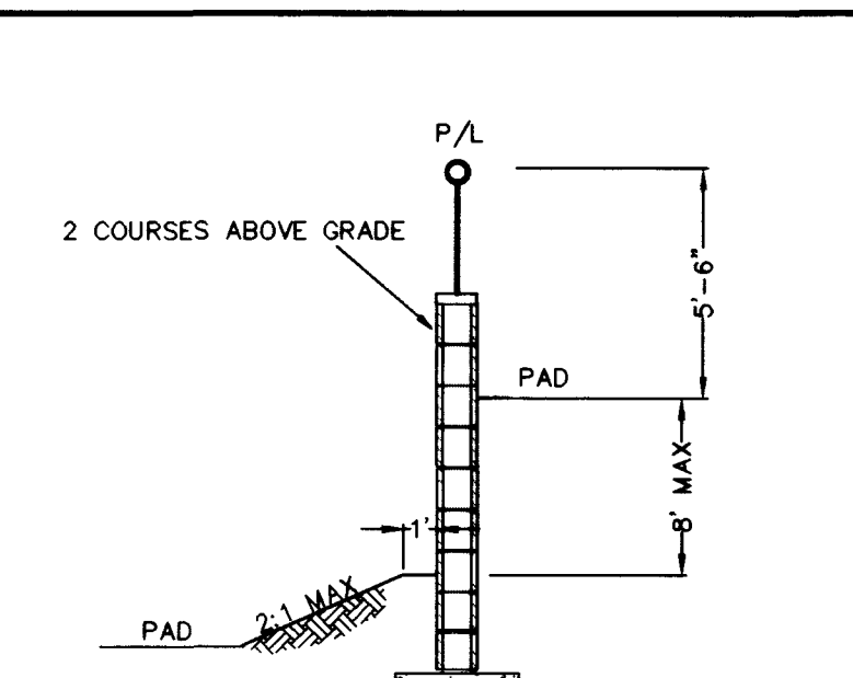
SECTION L - FINGER PARK
