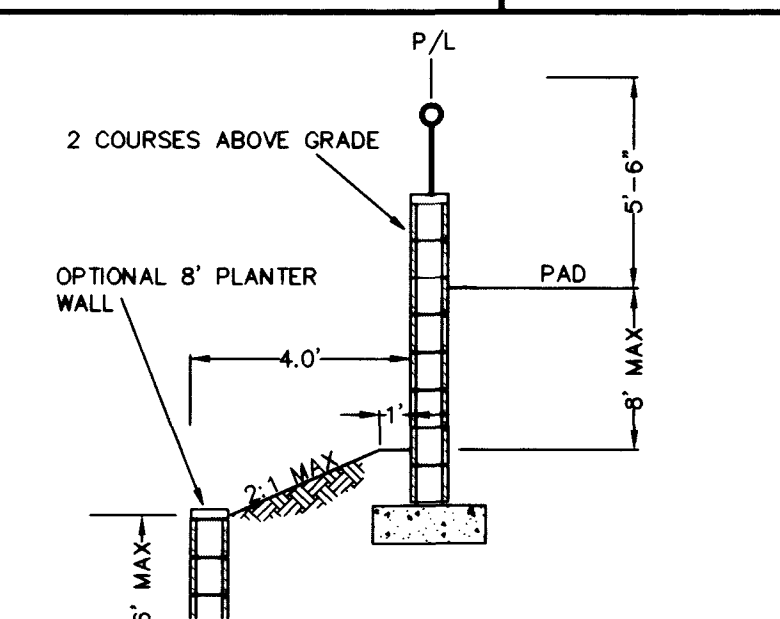
SECTION K - PED ACCESS
