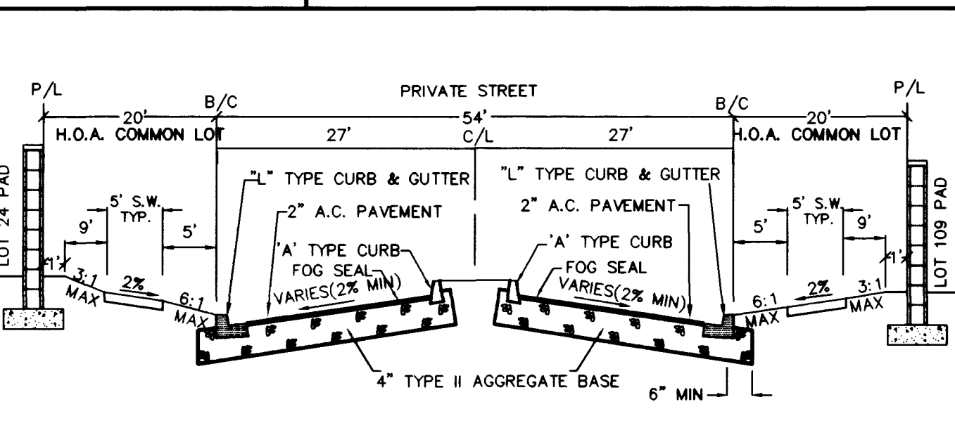
SECTION R - PARCEL ENTRY
