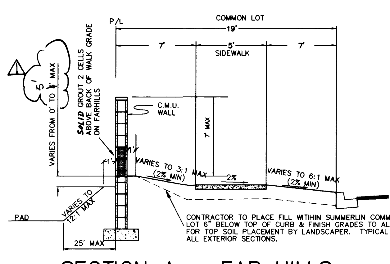
SECTION A - FAR HILLS
