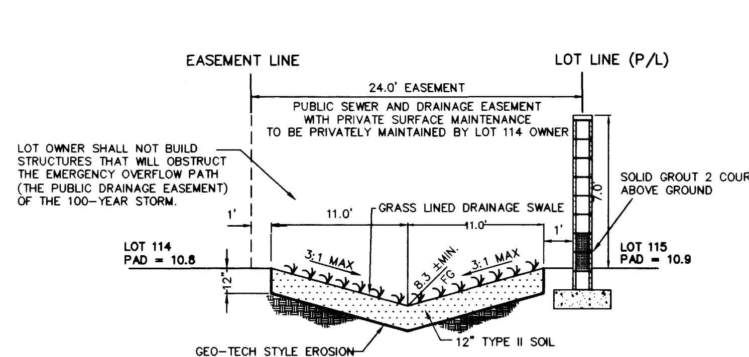
SECTION G-24' SEWER/STORM EASEMENT
