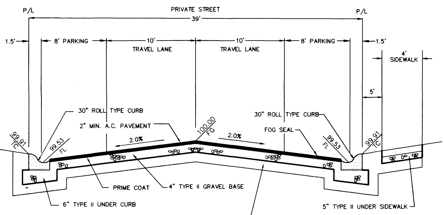
SECTION O - INTERIOR STREET (TYP.) - PRIVATE
