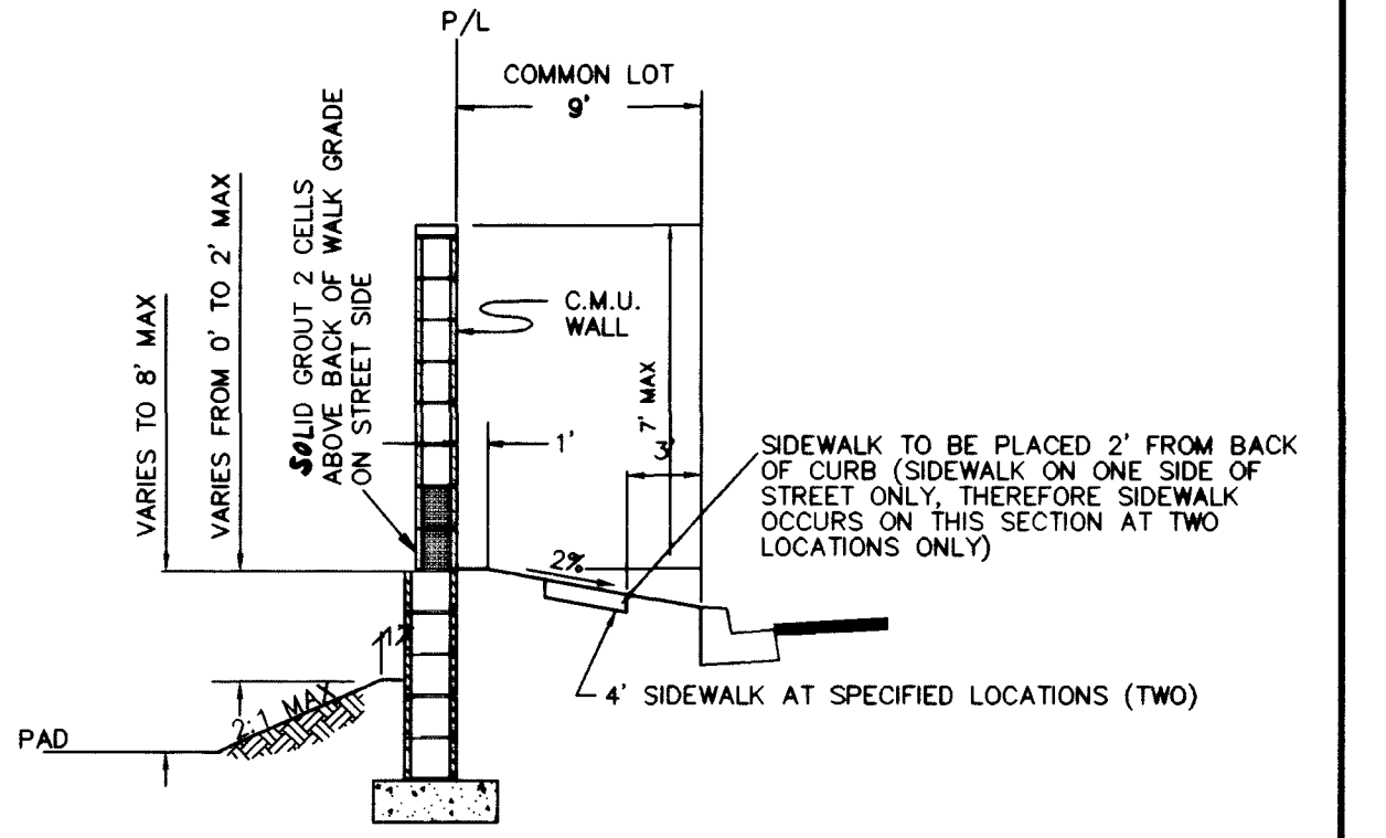
SECTION H - INTERIOR STREET
