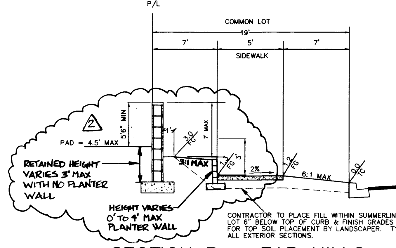
SECTION B - FAR HILLS
