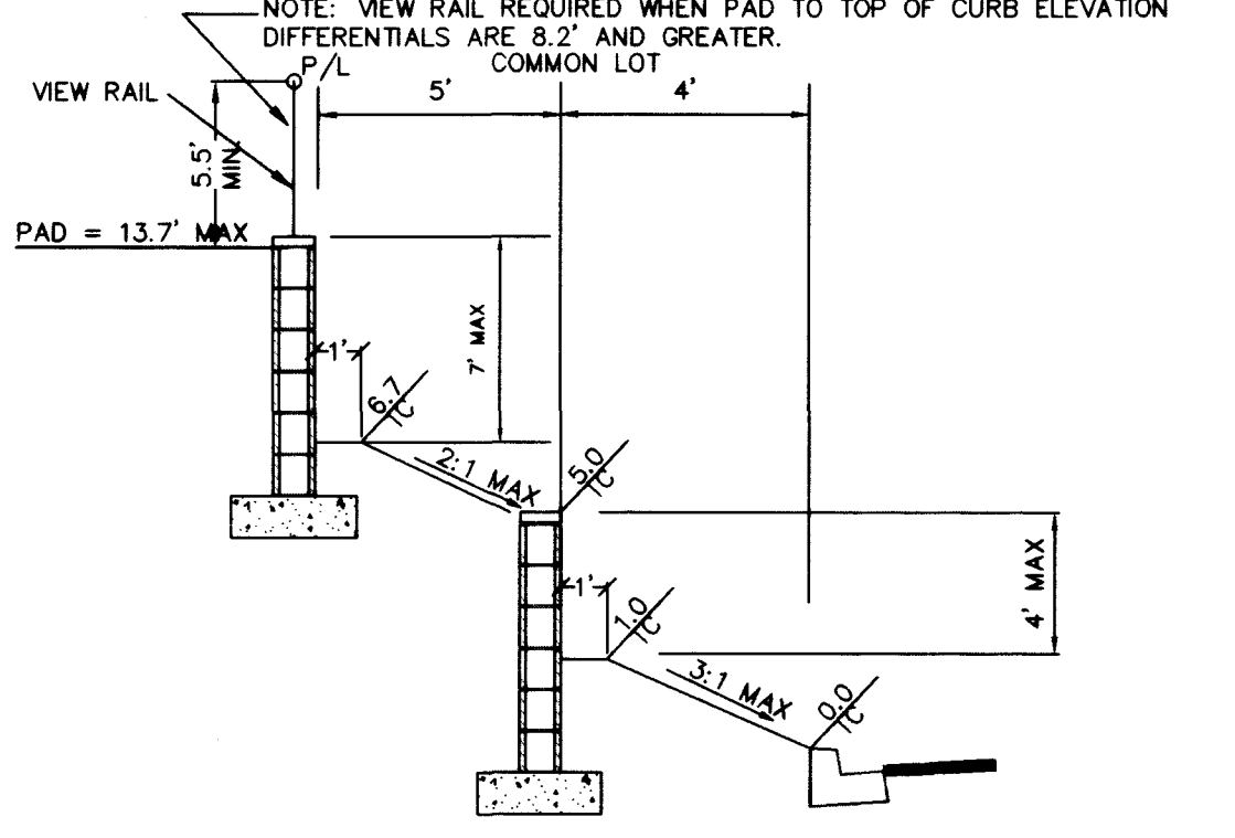
SECTION I - INTERIOR STREET
