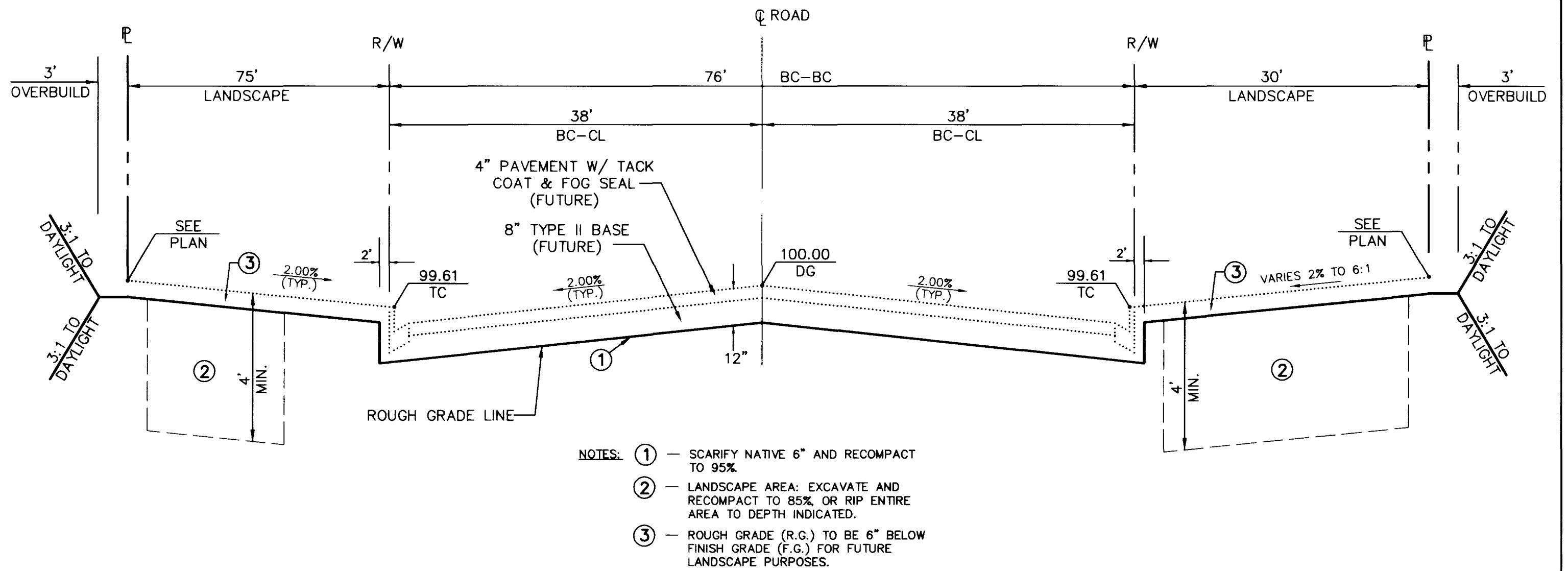
ALTA DRIVE - TYPICAL SECTION
