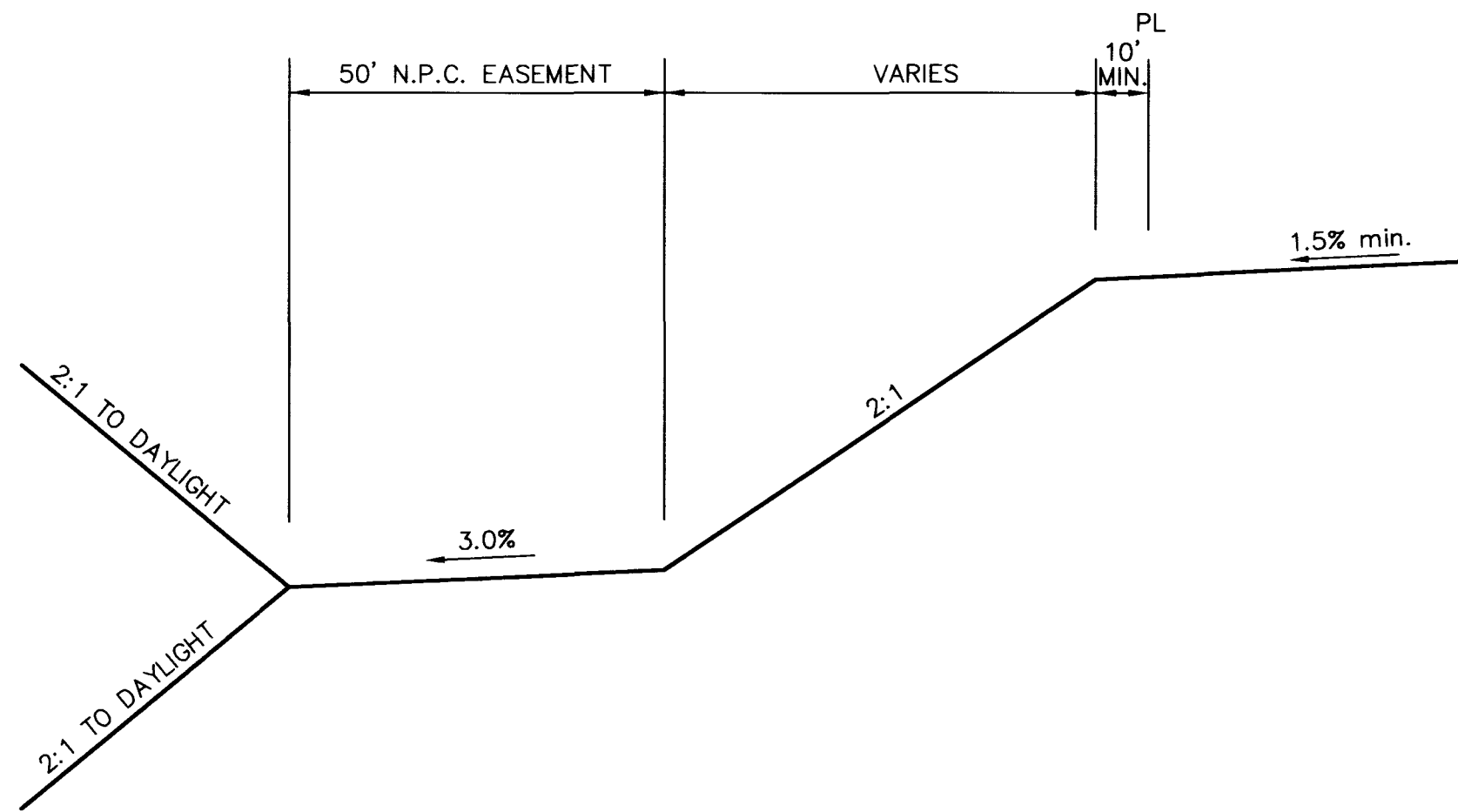
W. B. UTILITY CORIDOR AND CHANNEL - TYPICAL SECTION
