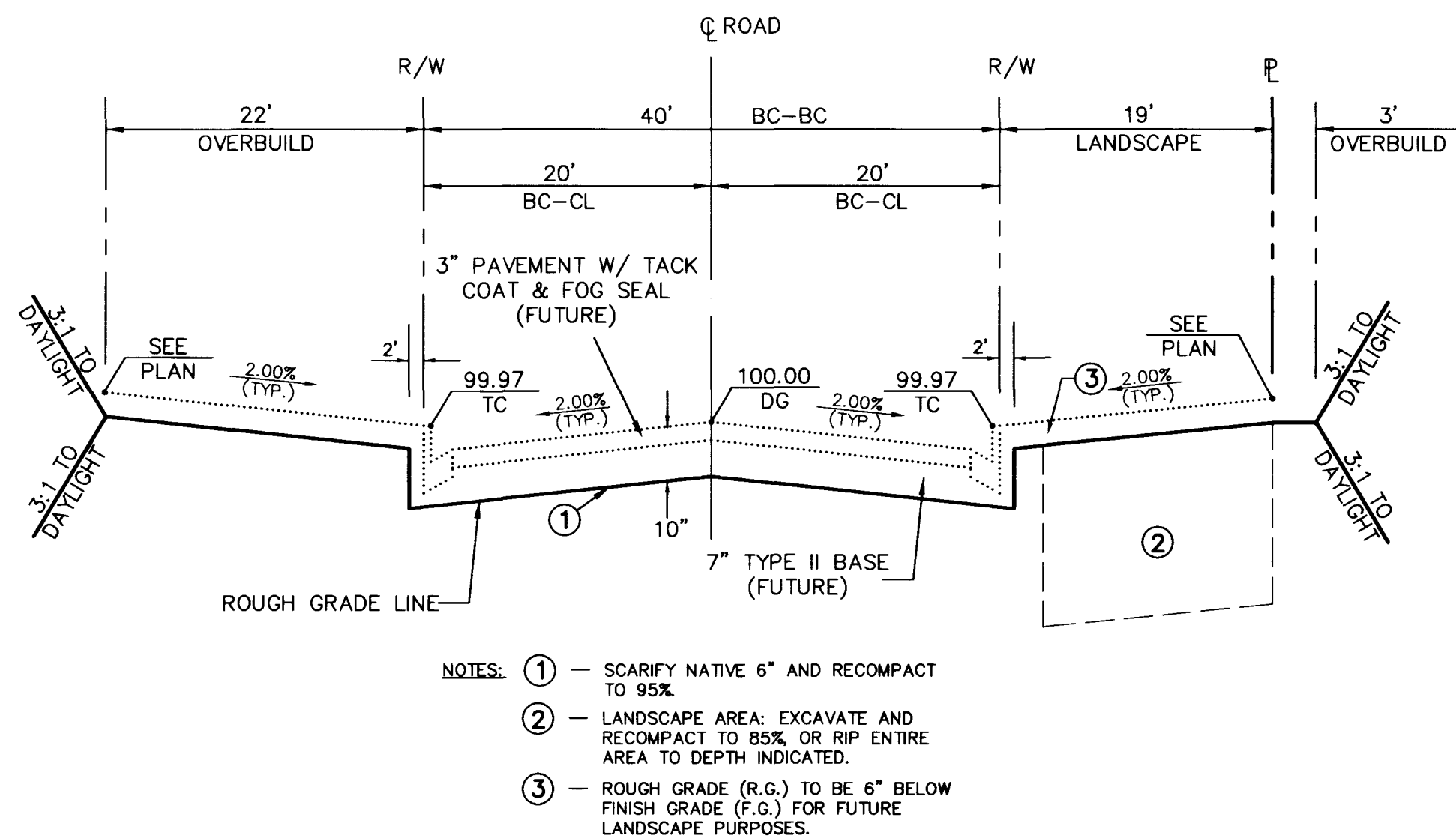
STREETS I AND J - TYPICAL SECTION
