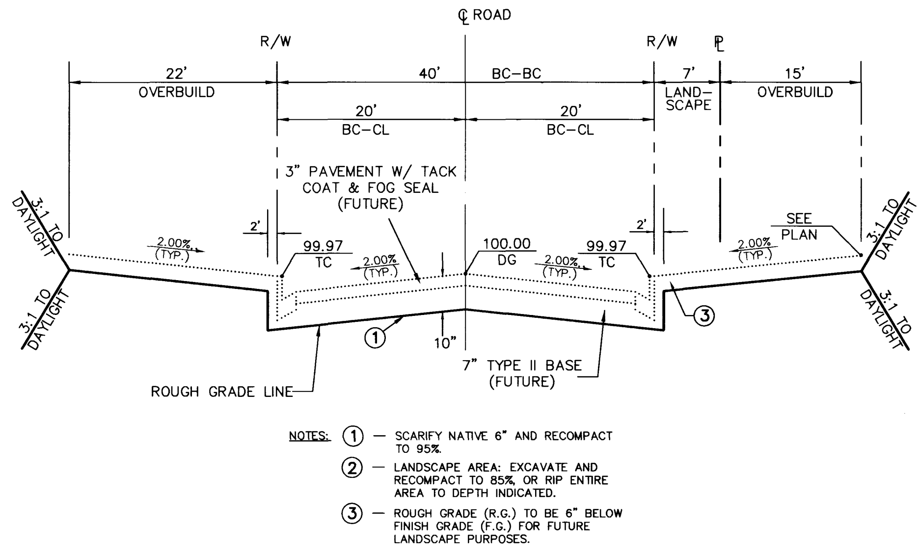
STREET K - TYPICAL SECTION
