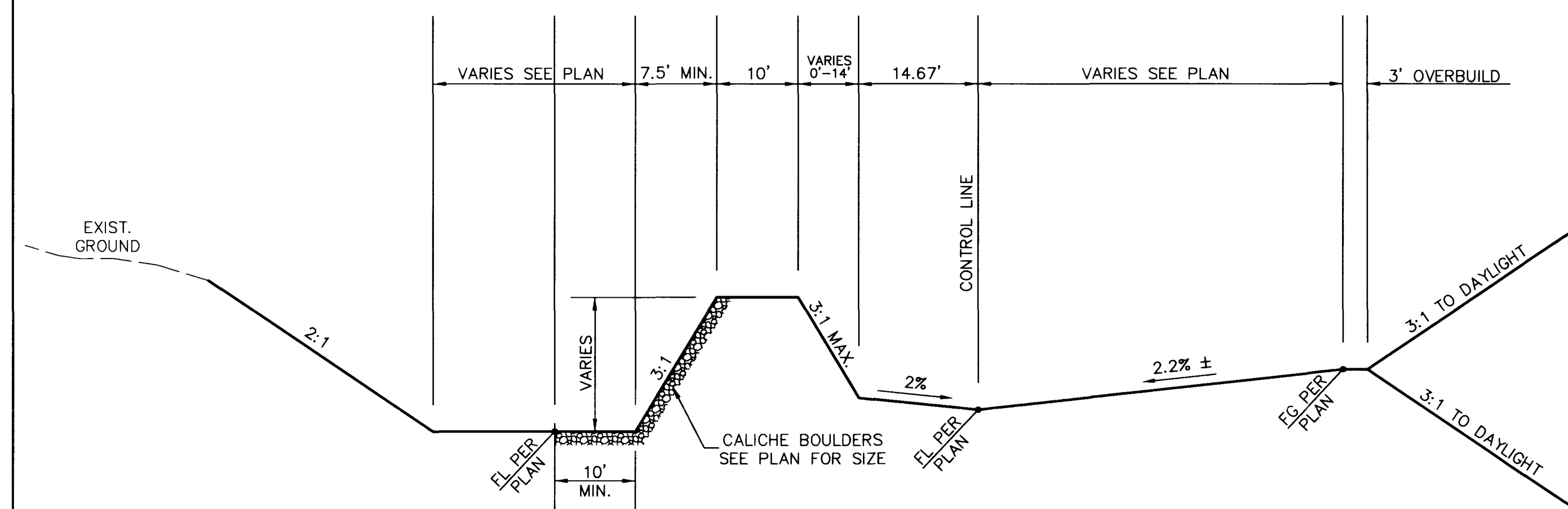
FOOTHILLS PKWY. INTERIM CHANNEL - TYPICAL SECTION
