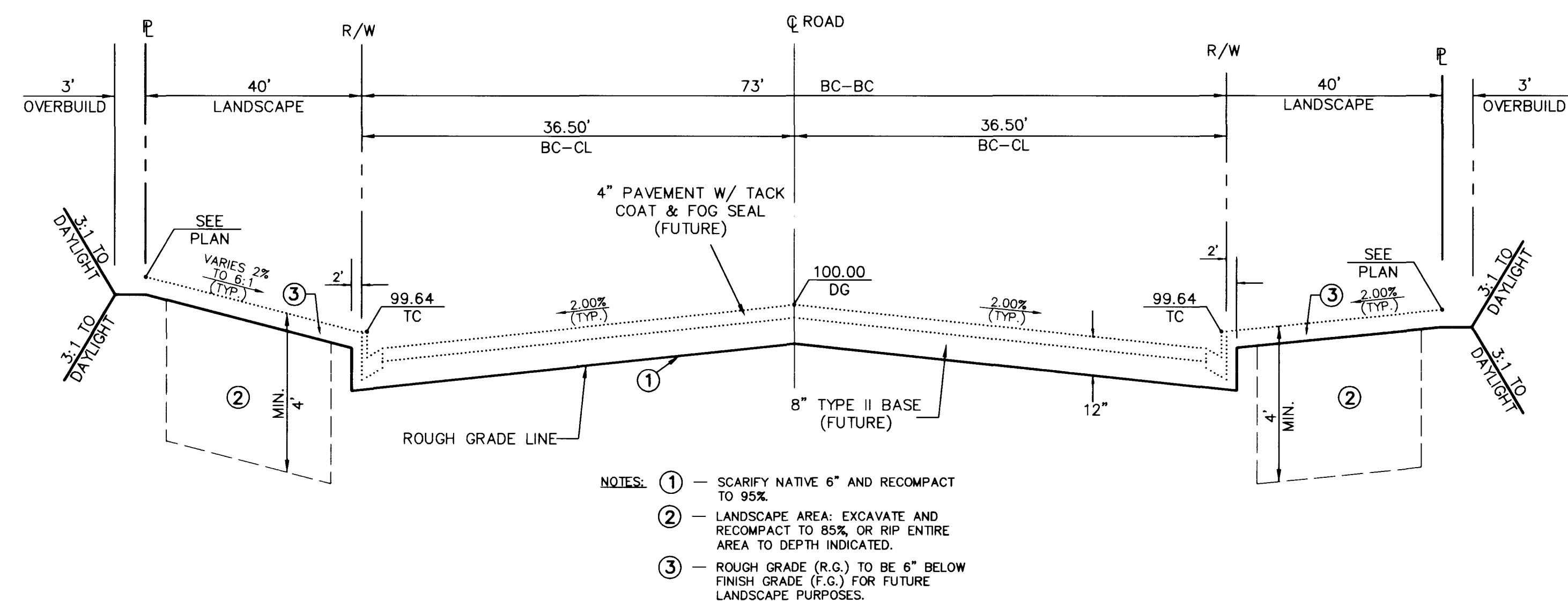
STREET F - TYPICAL SECTION
