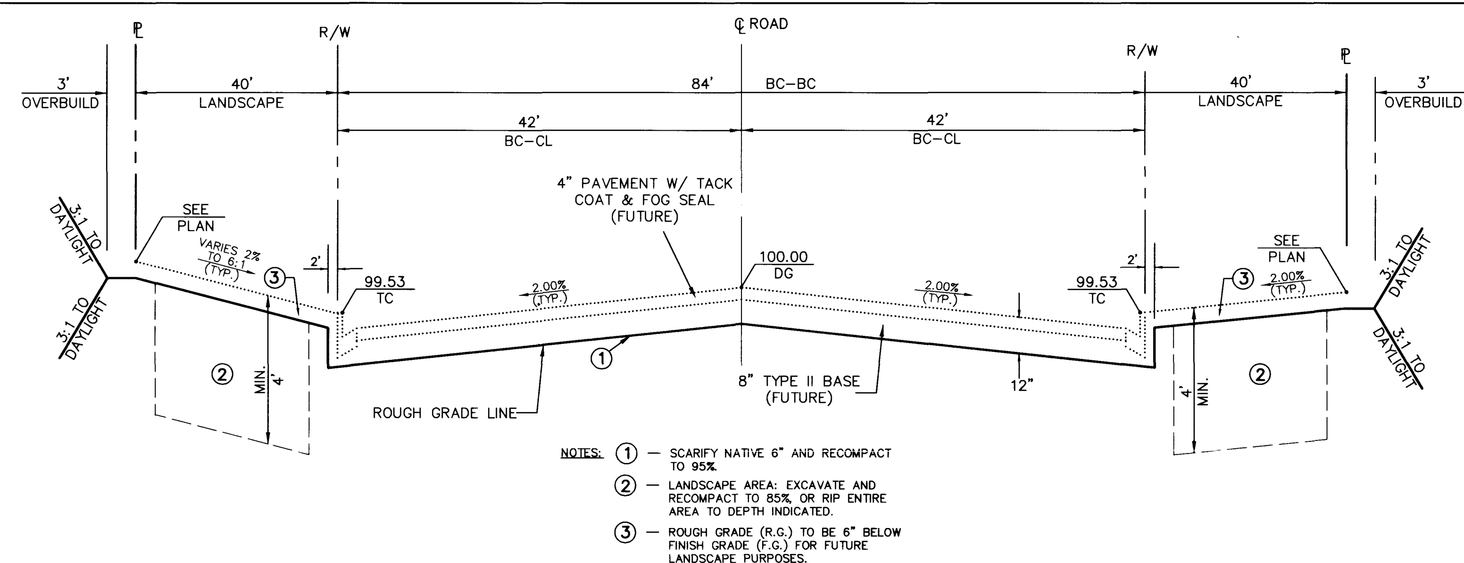
STREET D - TYPICAL SECTION
