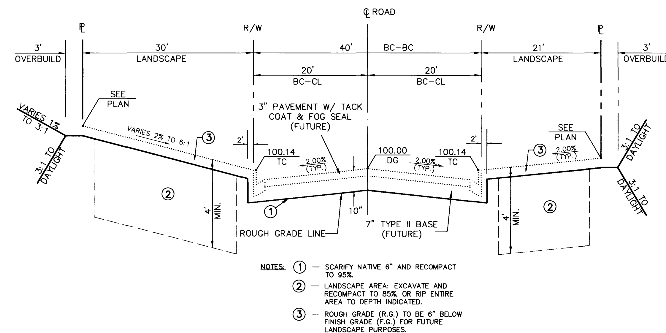
STREETS 'A/E' AND 'B/G' - TYPICAL SECTION
