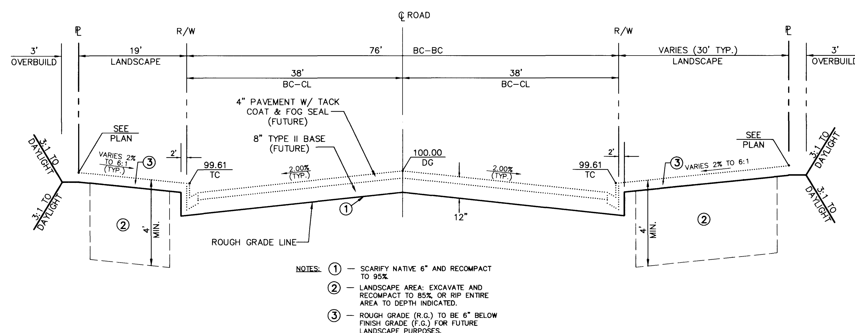
FAR HILLS AVENUE - TYPICAL SECTION
