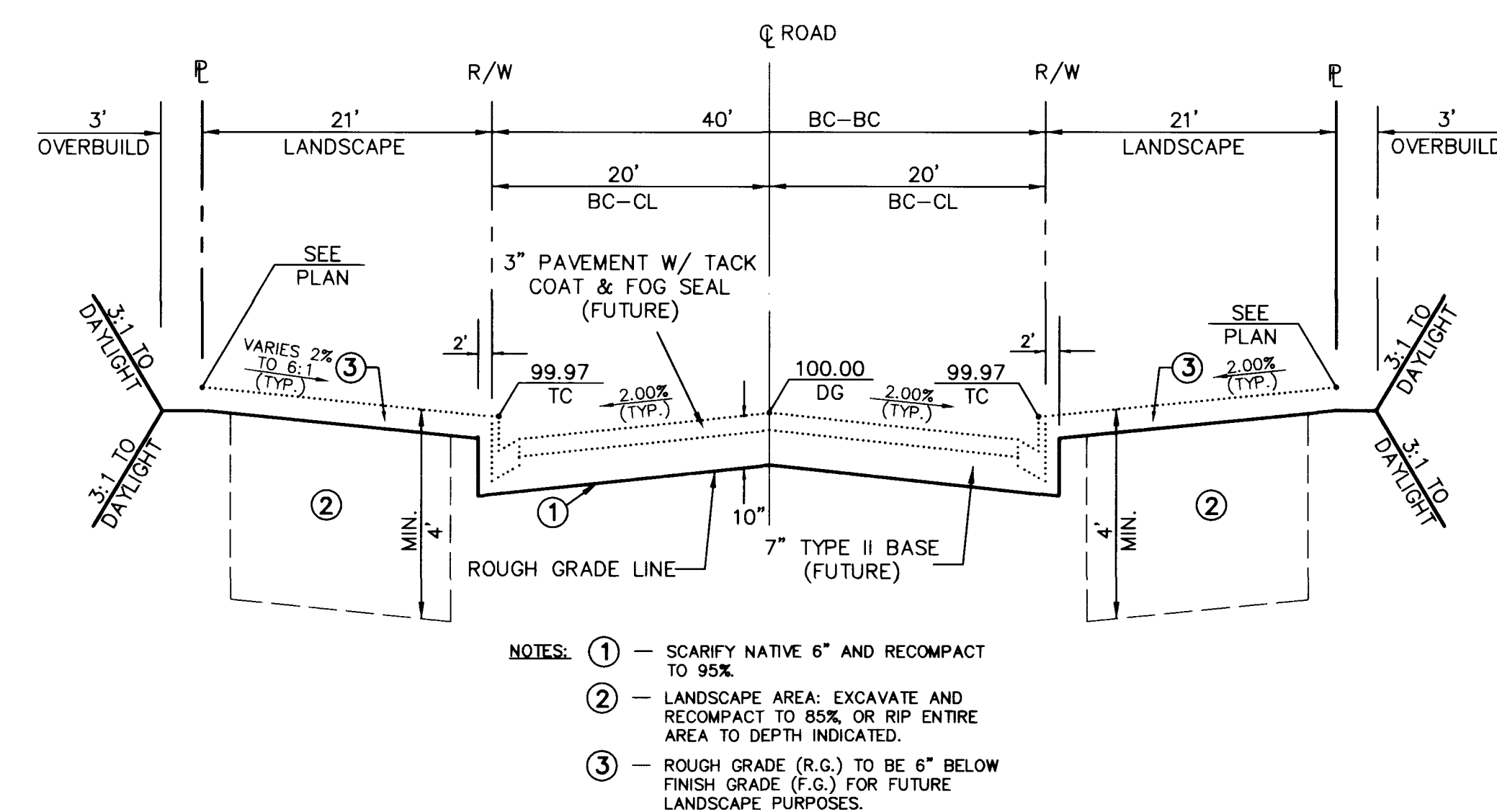
STREETS C AND H - TYPICAL SECTION
