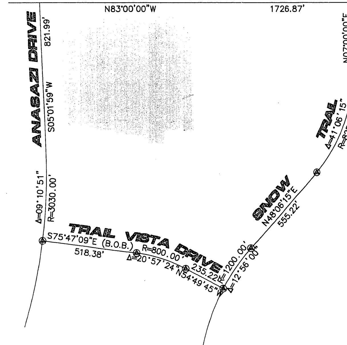
SURVEY ANALYSIS SCALE: 1"=200'
