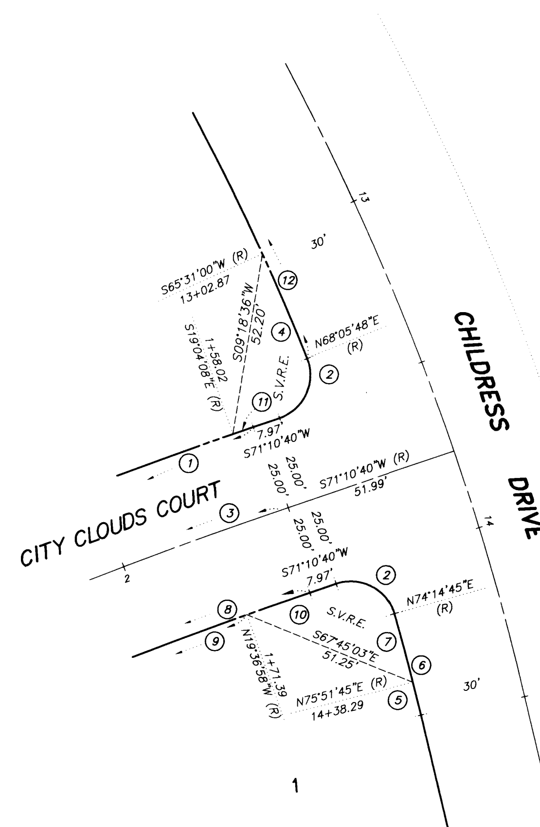
S.V.R.E. DETAIL NOT TO SCALE
