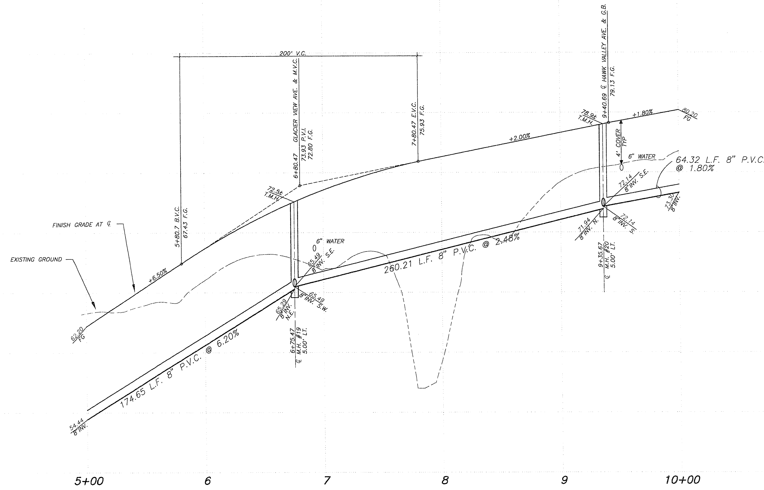
PROFILE SCALE: HORIZ. 1" = 40' VERT. 1" = 4'
