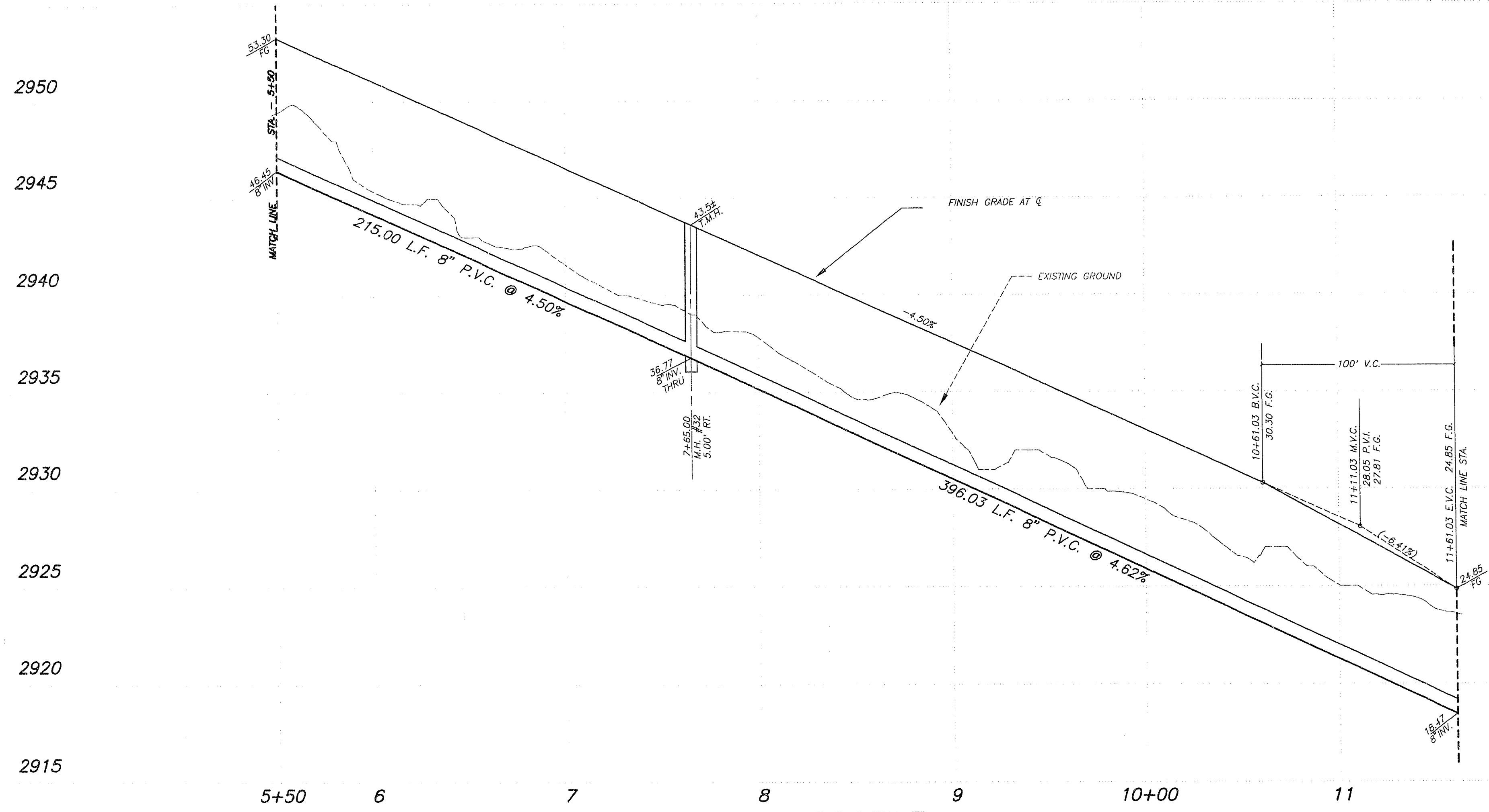
PROFILE SCALE: HORIZ. 1" = 40' VERT. 1" = 4'
