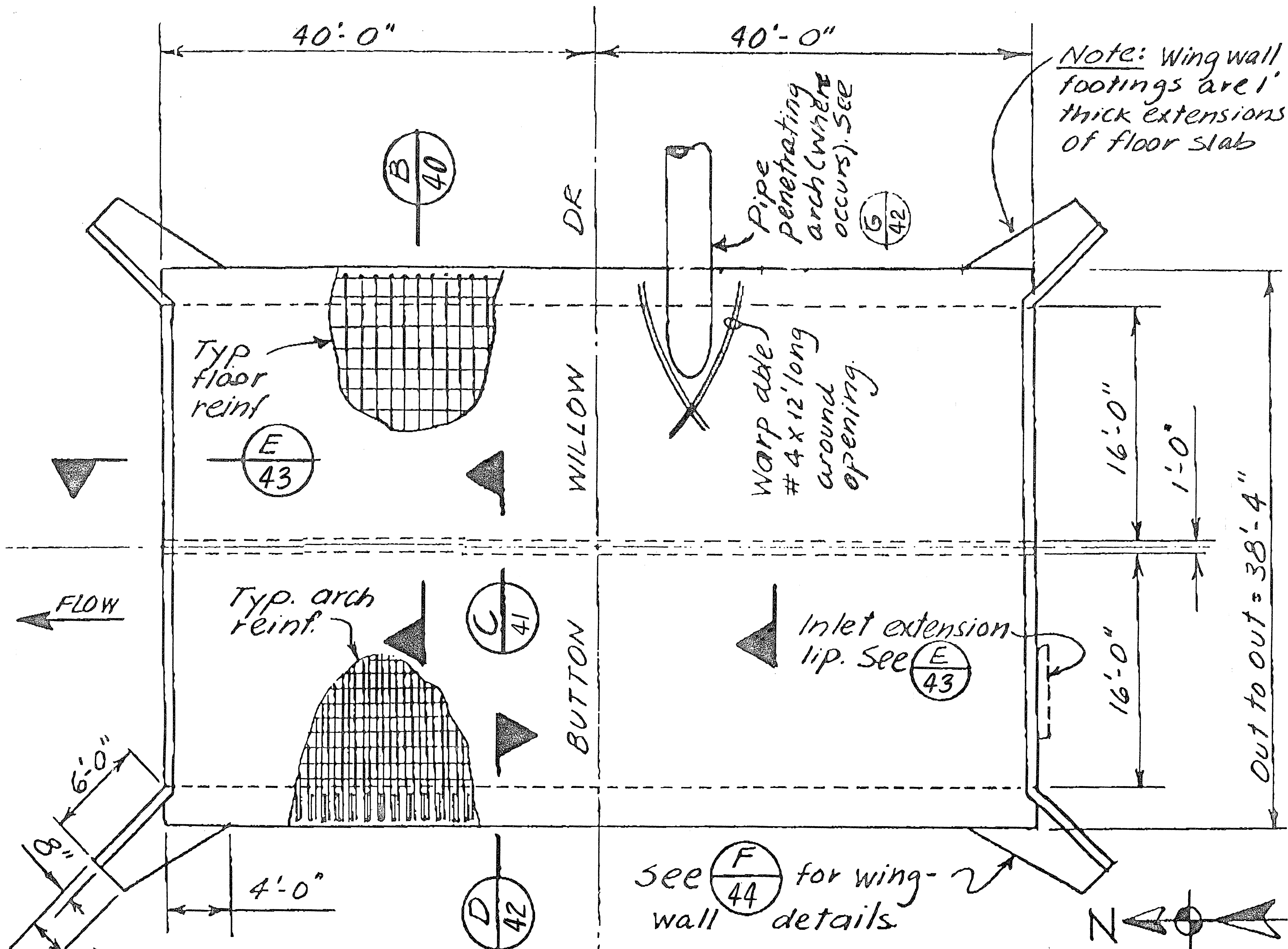
PLAN - ARCH CULVERT @ STA. 48+10.00 BUTTON WILLOW DRIVE Scale 1"=10'
