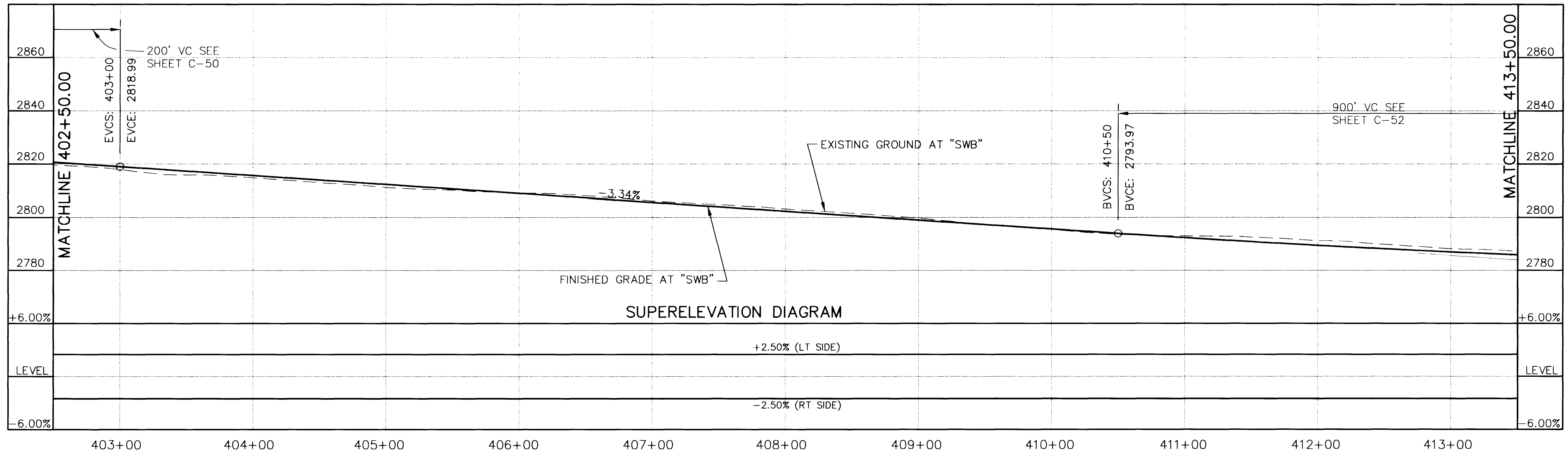
SUMMERLIN PARKWAY "SWB" PROFILE
