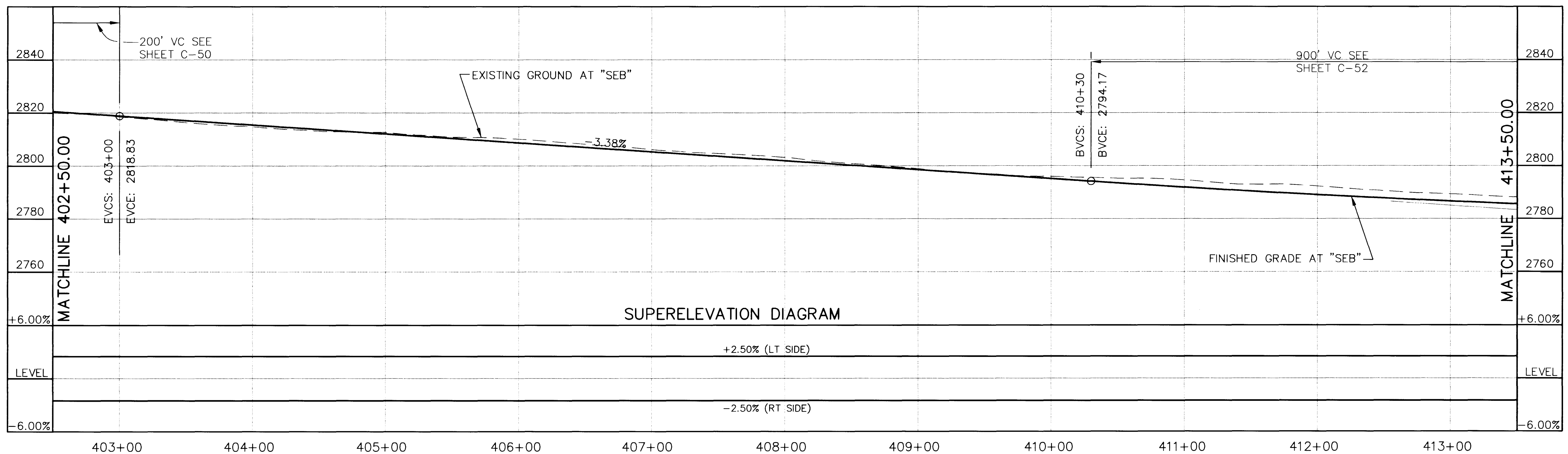
SUMMERLIN PARKWAY "SEB" PROFILE
