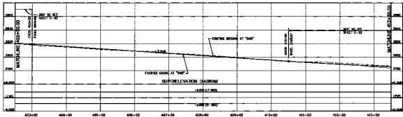
SUMMERLIN PARKWAY "SWB" PROFILE
