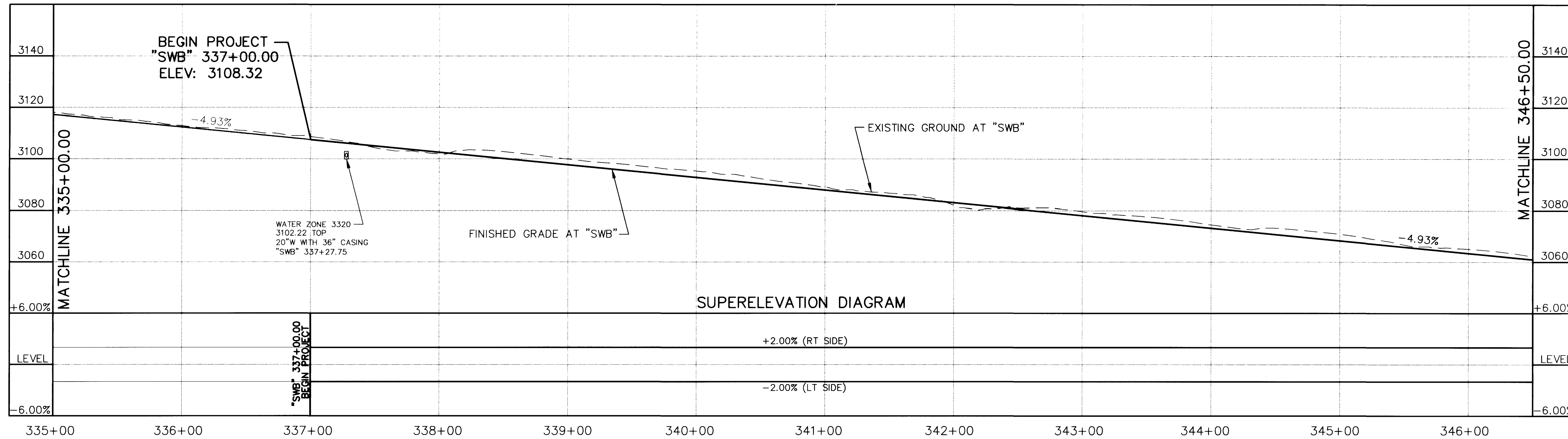
SUMMERLIN PARKWAY "SWB" PROFILE
