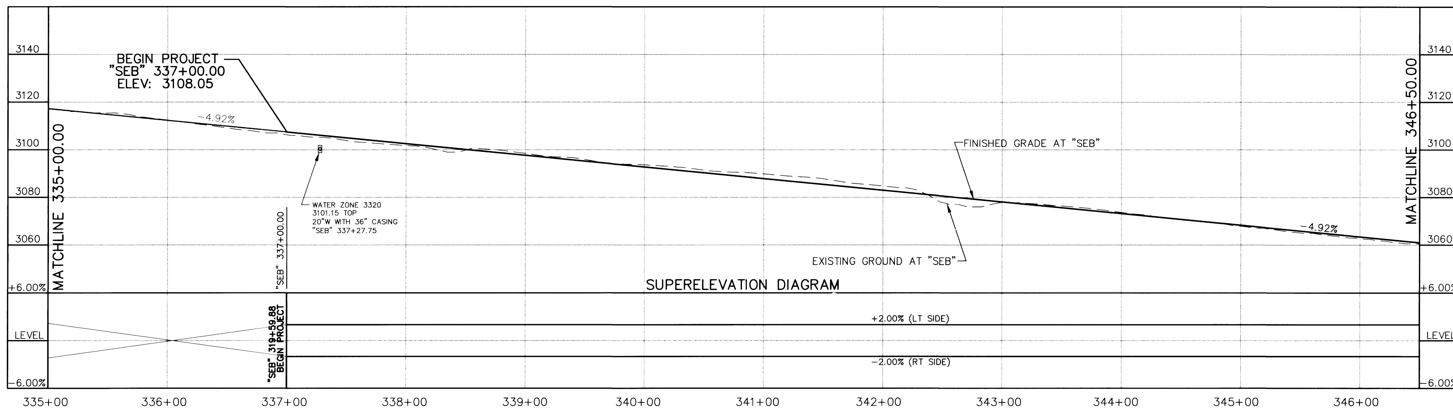
SUMMERLIN PARKWAY "SEB" PROFILE
