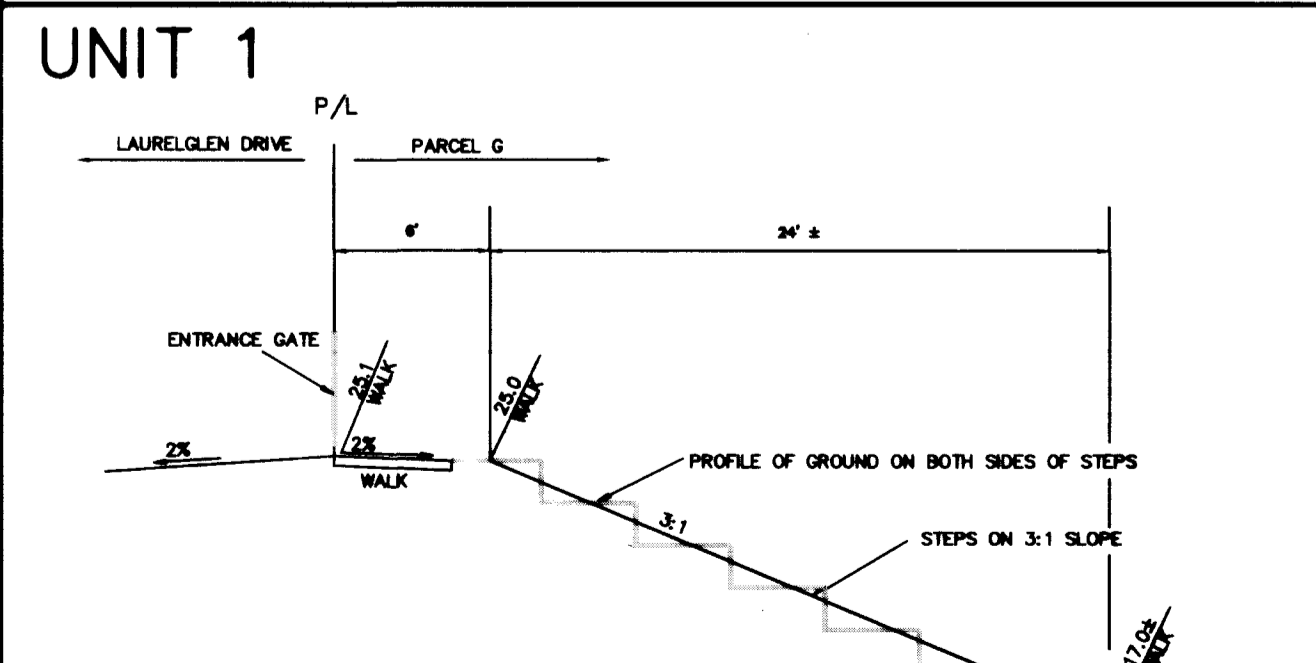
SECTION O
