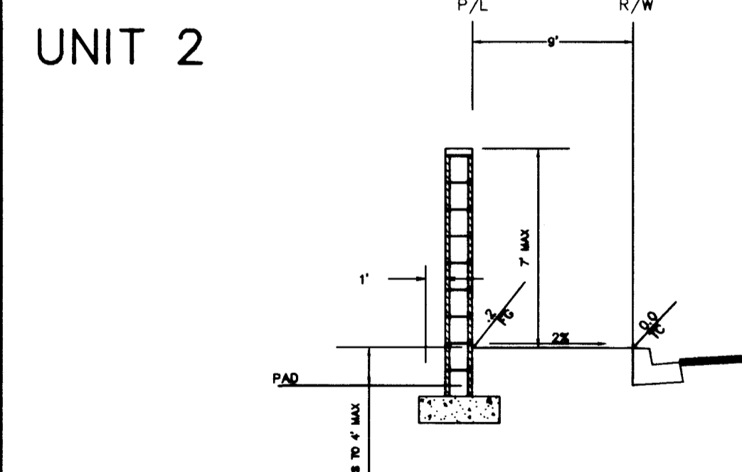
SECTION K
