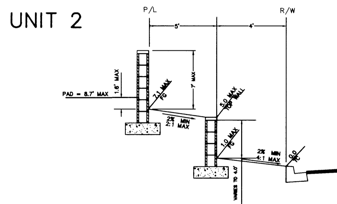
SECTION I
