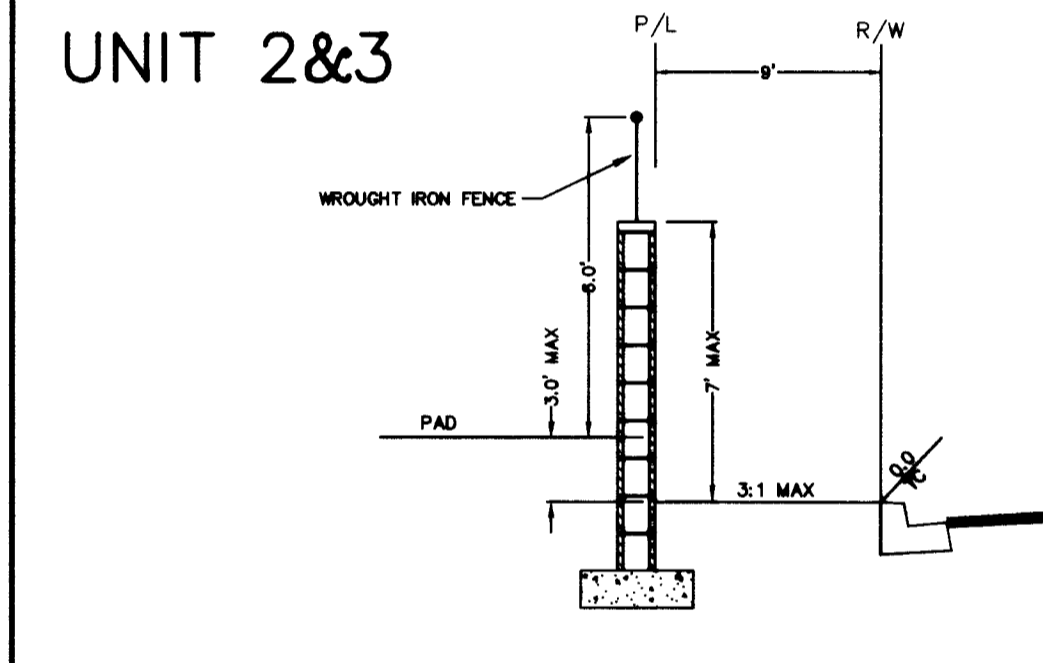
SECTION L
