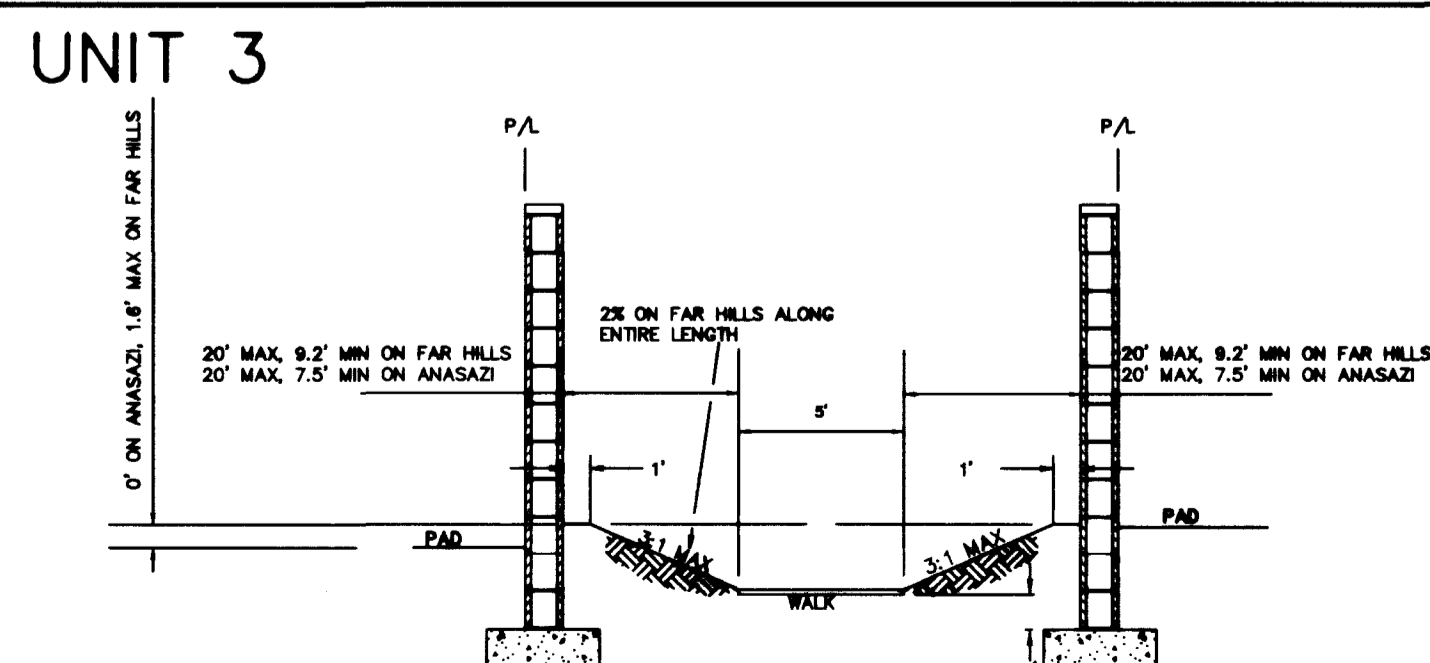
SECTION M
