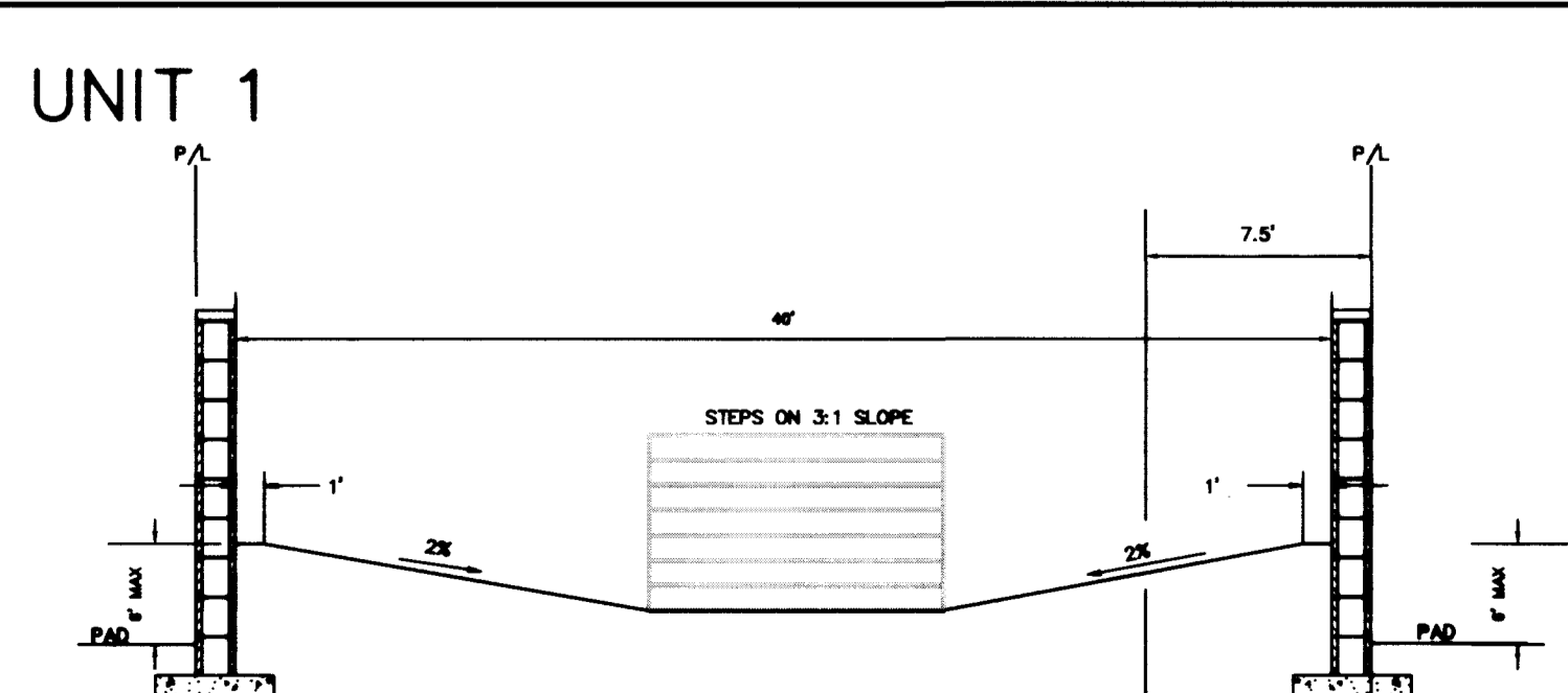
SECTION N
