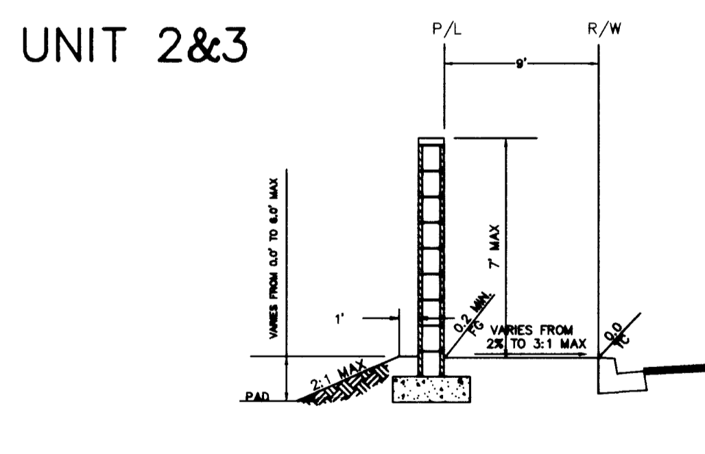
SECTION J
