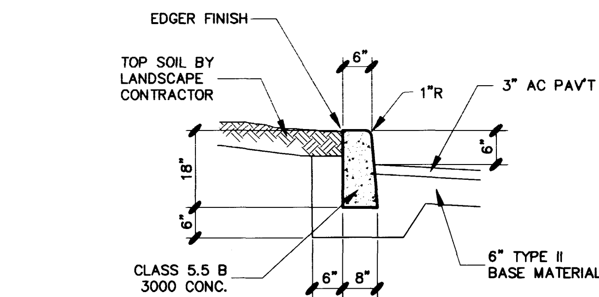
'A' TYPE CURBING
