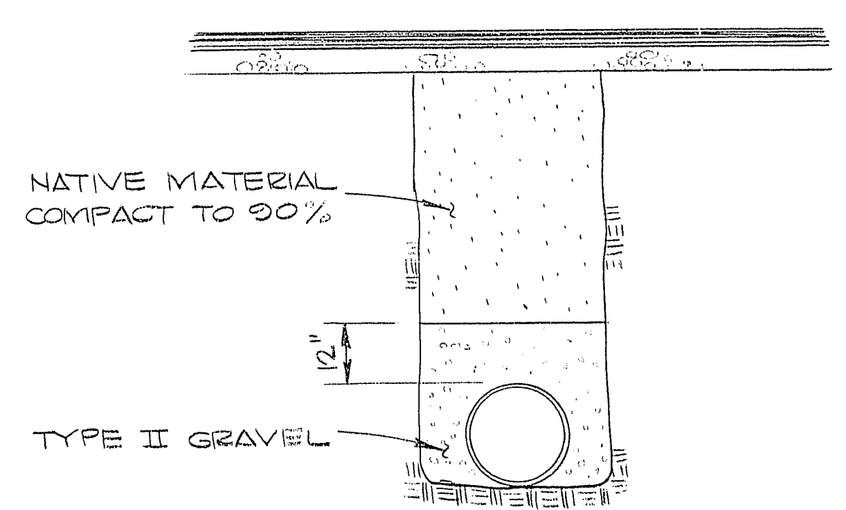
TYP. TRENCH SECTION FOR SEWER ONLY
