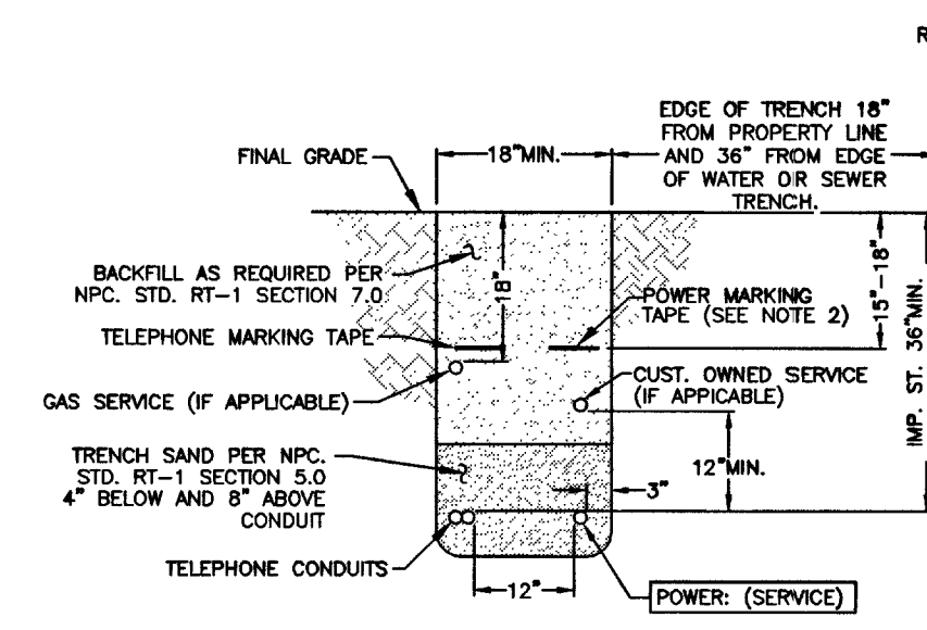
TRENCH DETAIL NPC U.G. STD. RT-8 (REV. 4/8/02) (RESIDENTIAL SERVICES)
