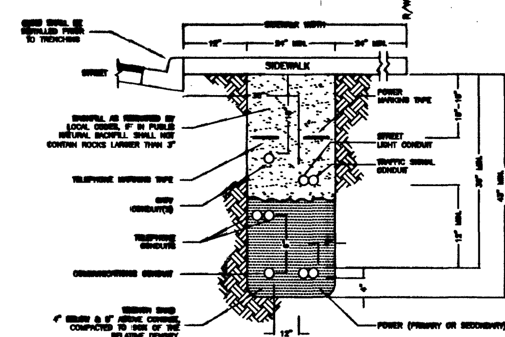
SIDEWALK TRENCH DETAIL PRIVATE & PROJECT INTERIOR TRENCH (NOT TO SCALE)
