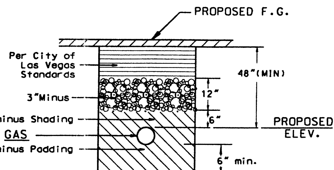
TRENCH DETAIL FOR UNIMPROVED AREAS ONLY CLV
