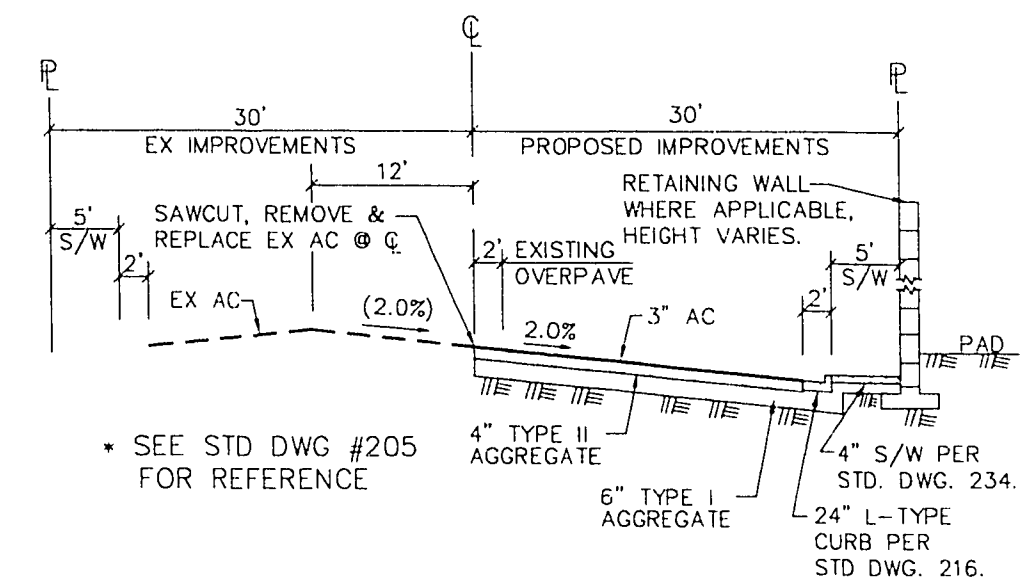
TYP. 60' HALF-STREET SECTION N.T.S.
