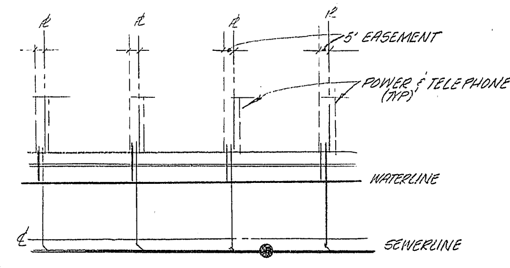
TYPICAL UTILITY DETAIL
