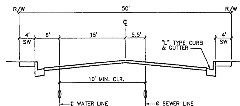
TYPICAL UTILITY LOCATION (NOT TO SCALE)
