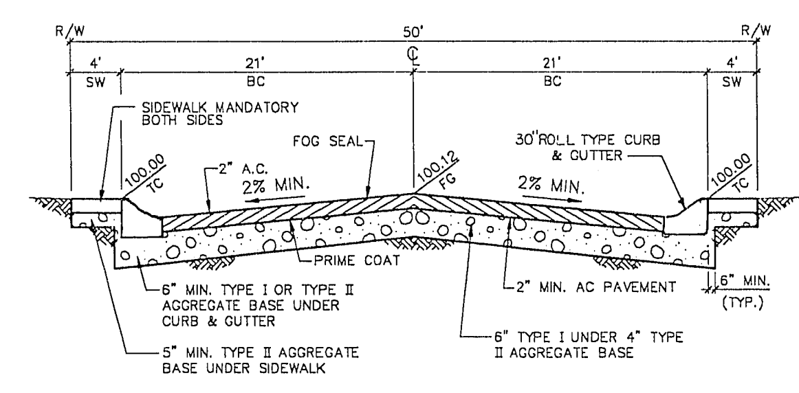
TYPICAL 50' STREET SECTION SUMMERLIN STD. DWG. NO. S-8 (8/88) (NOT TO SCALE)
