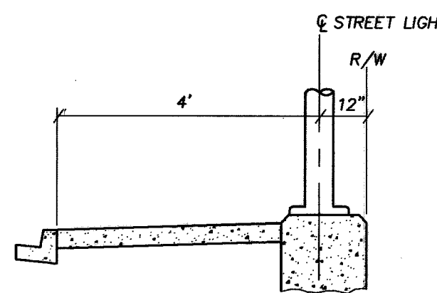
TYPICAL STREET LIGHT LOCATION WITH ATTACHED SIDEWALK ON-SITE NOT TO SCALE
