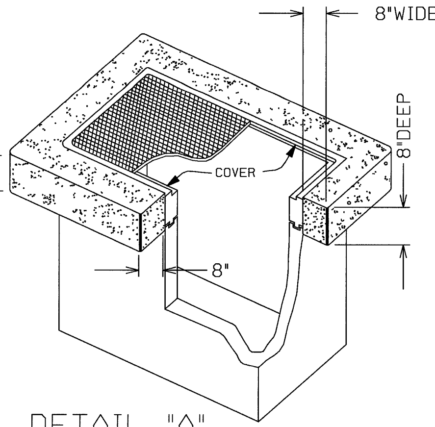
DETAIL "A"
