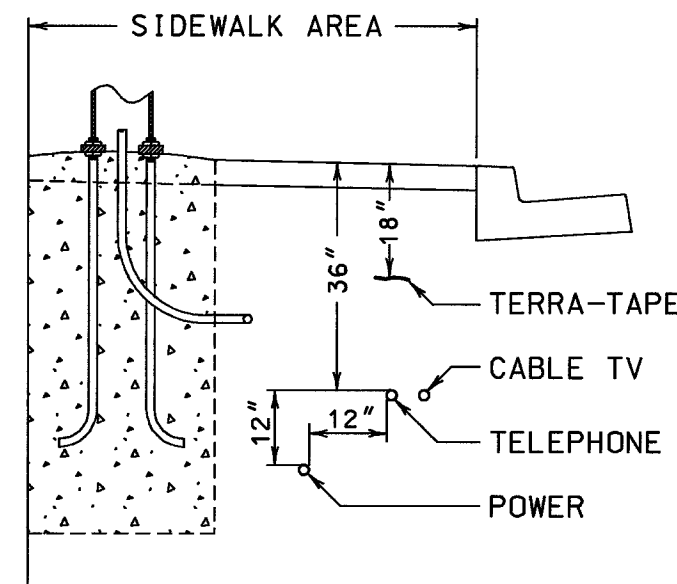
OFFSITE TRENCH DETAIL WITH SIDEWALK
