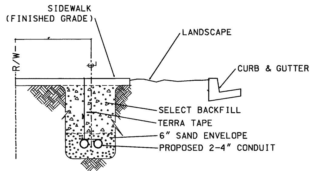
TRENCH DETAIL WITH SIDEWALK
