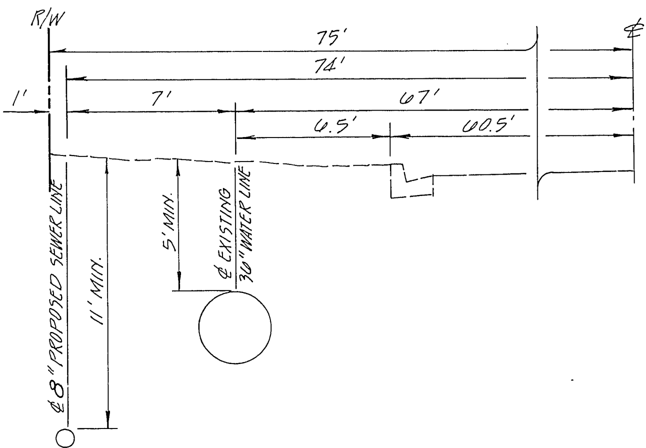
SEWER & WATER SEPARATION DETAIL N.T.S.
