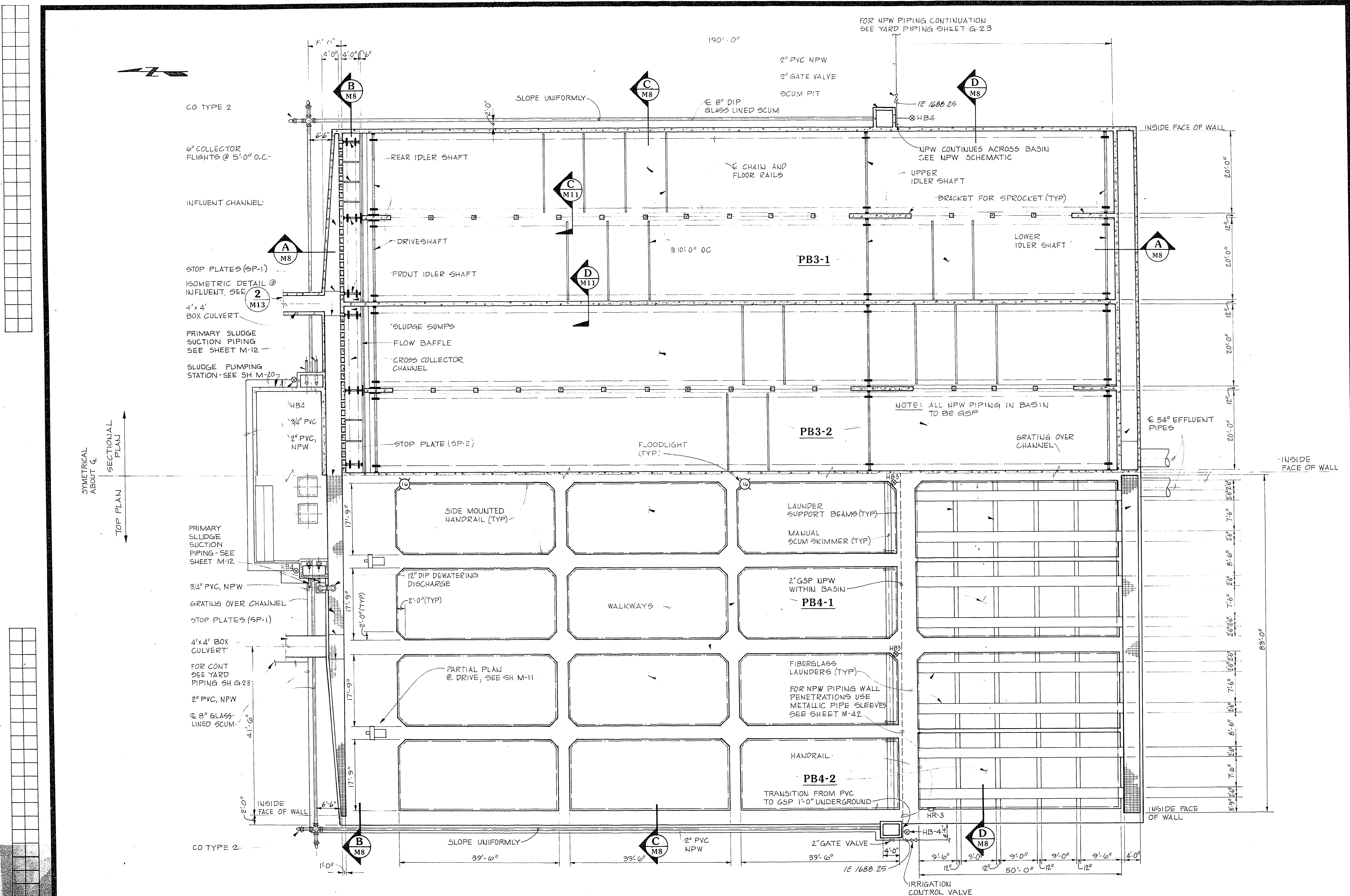
PLAN 1" = 10'-0"
