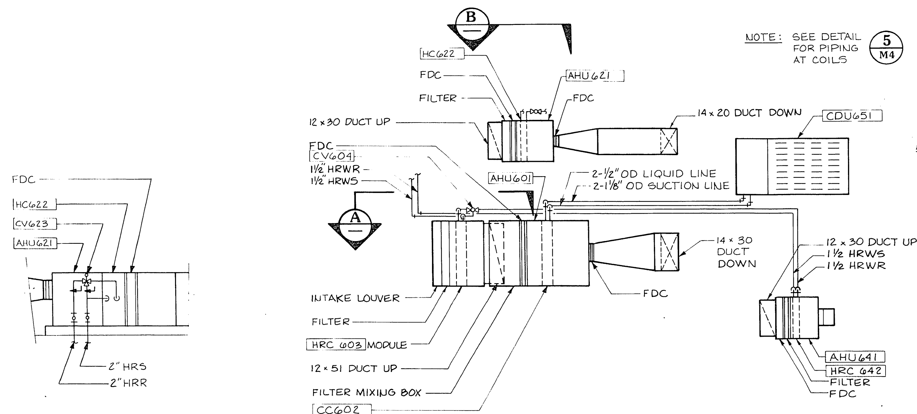
PARTIAL ROOF PLAN 1/4" = 1'-0"
