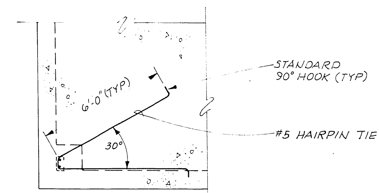
SECTIONAL PLAN AT CORNER POST
