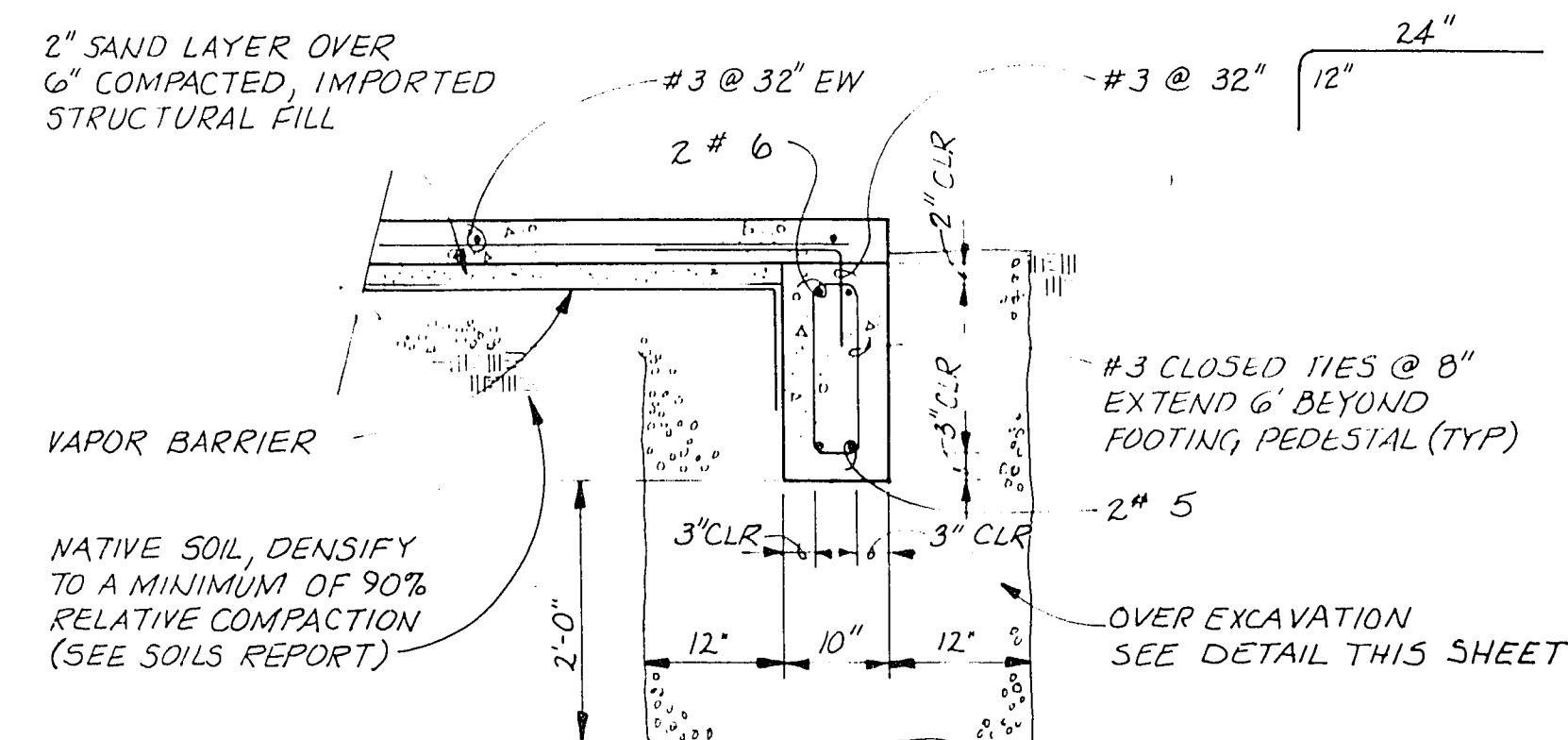
SECTION A 3/4" = 1'-0"
