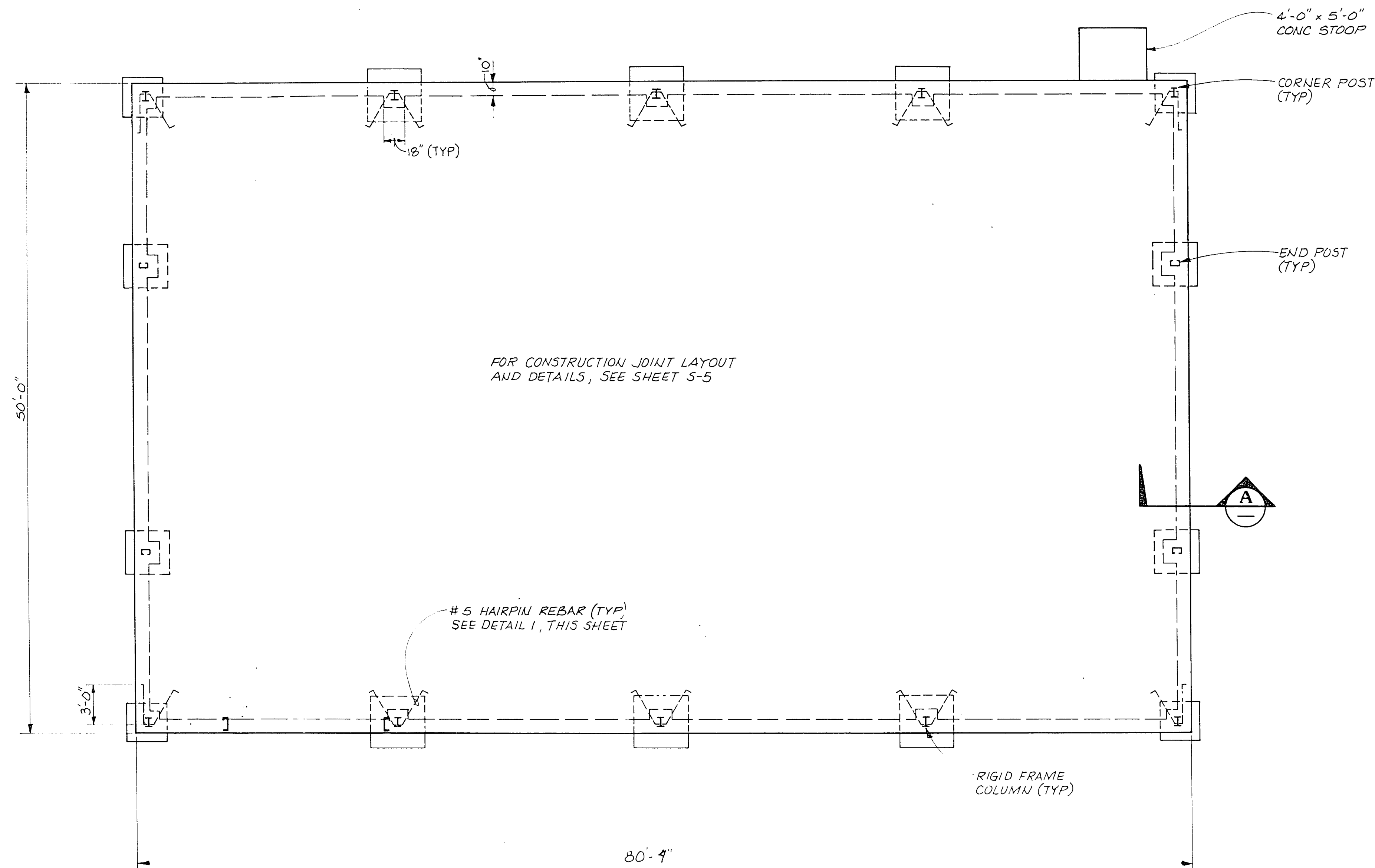
FOUNDATION PLAN 3/16" = 1'-0"
