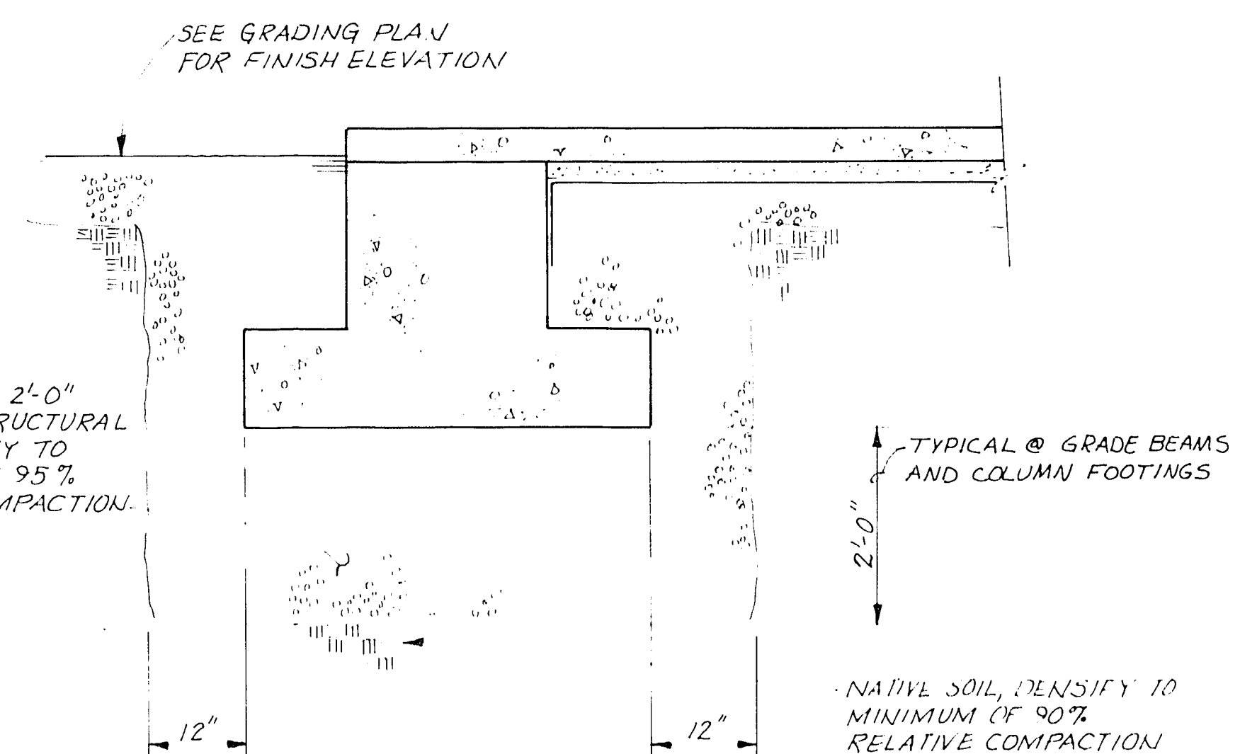
TYPICAL OVER-EXCAVATION DETAIL FOR FOOTINGS 3/4" = 1'-0"
