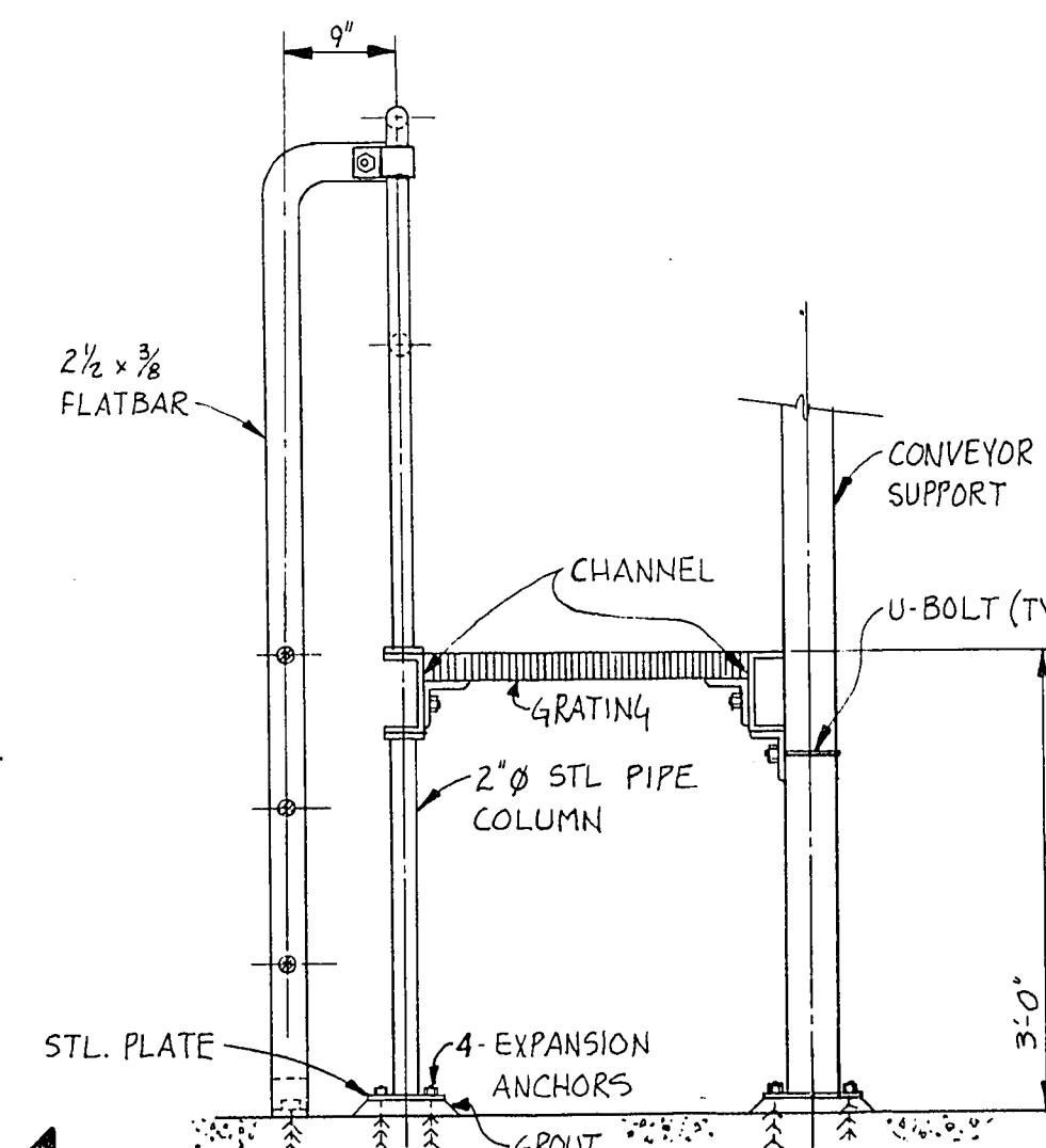
SECTION A
