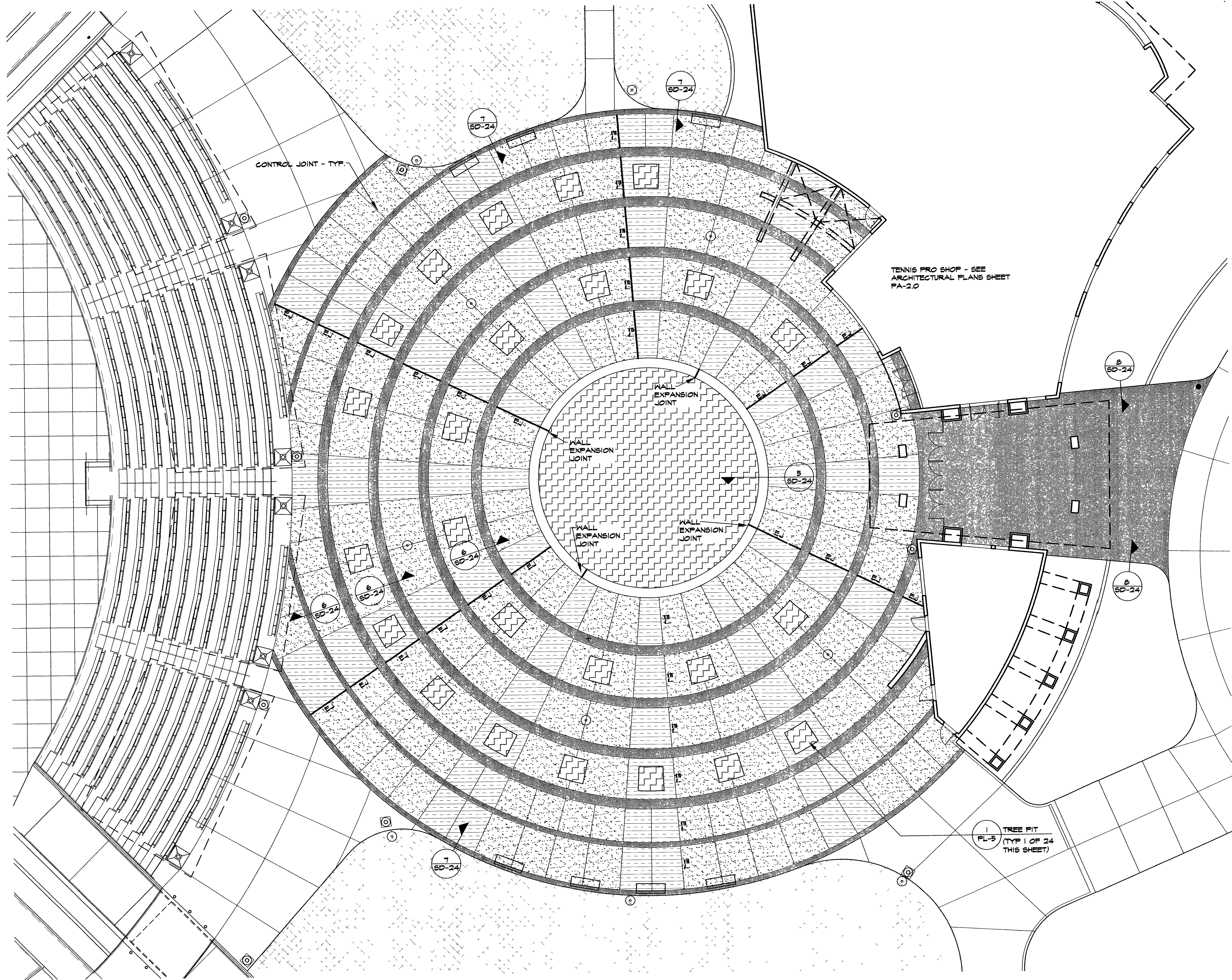
1 PLAZA LAYOUT
