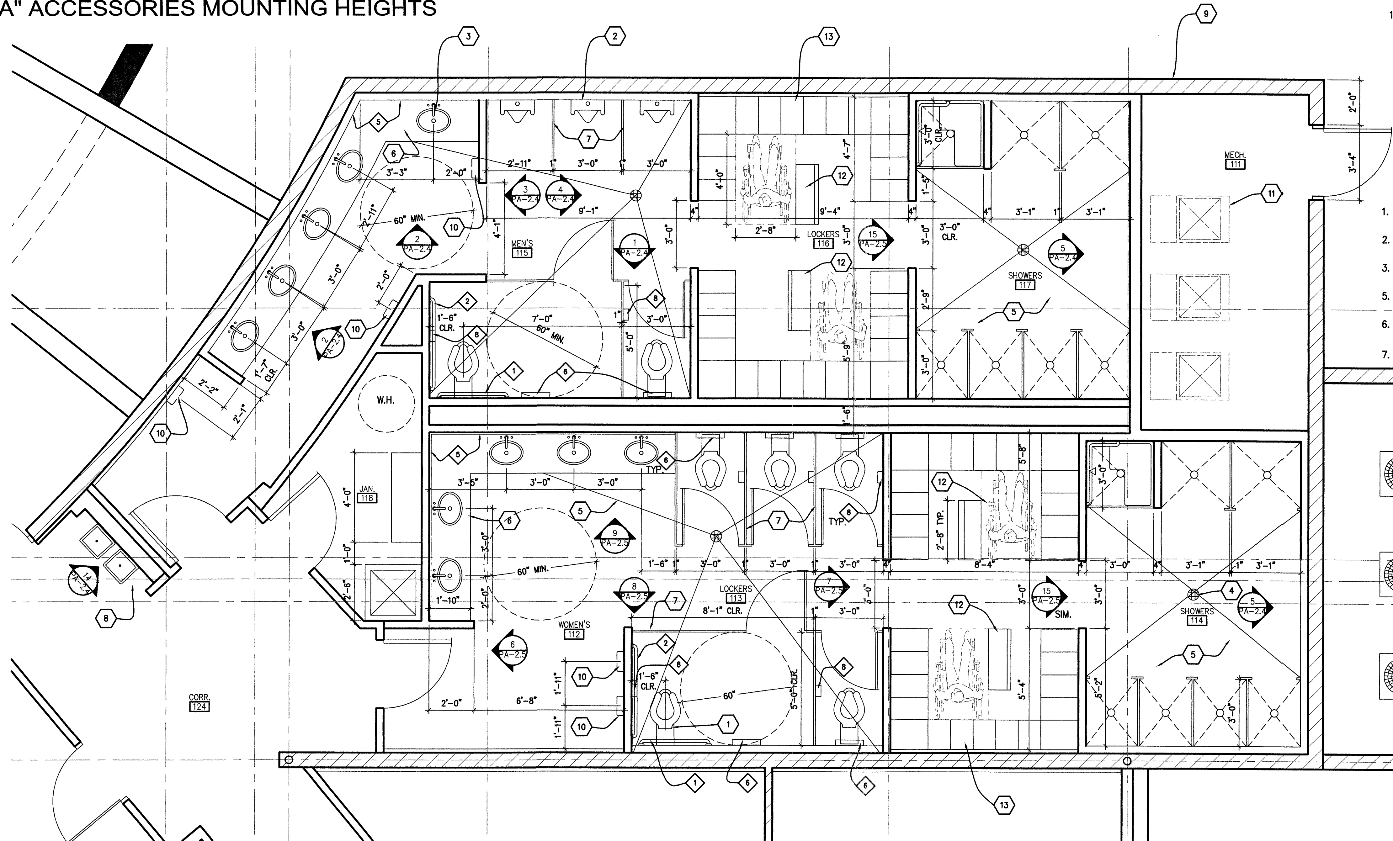
1 PRO-SHOP ENLARGED TOILET PLANS SCALE: 3/8"=1'-0"
