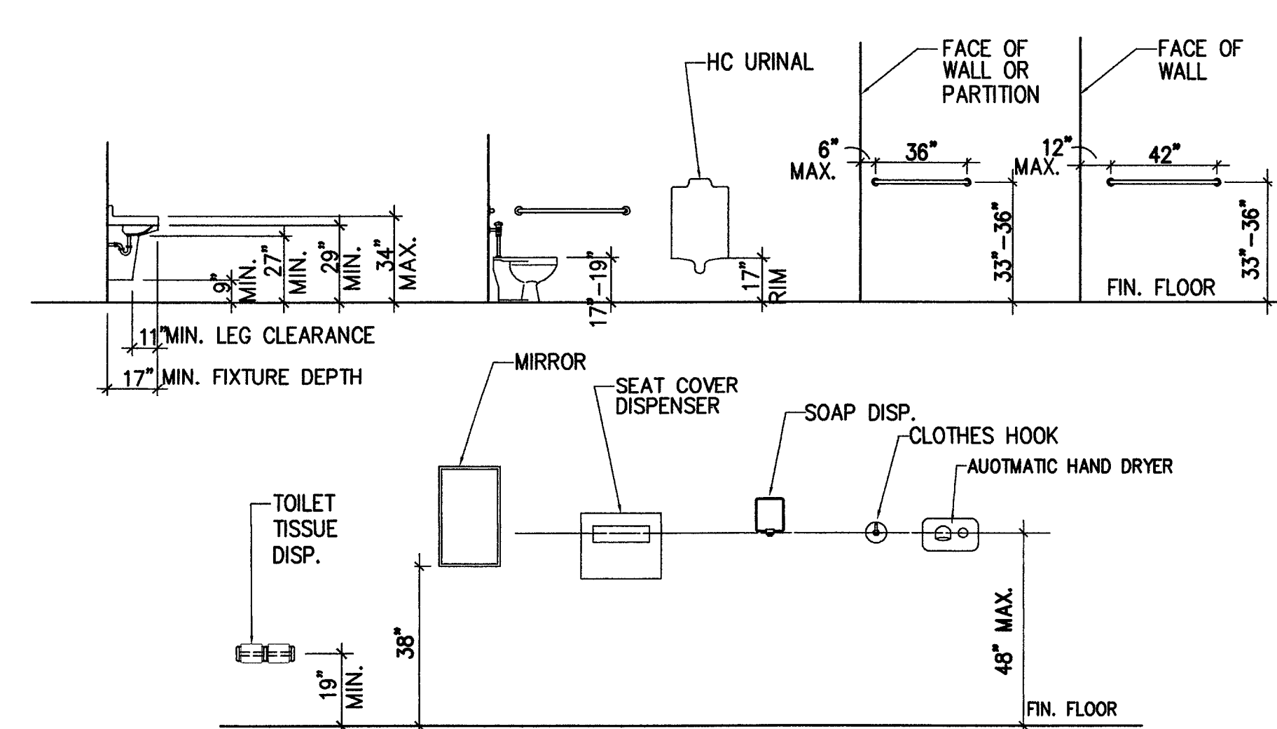
"ADA" ACCESSORIES MOUNTING HEIGHTS
