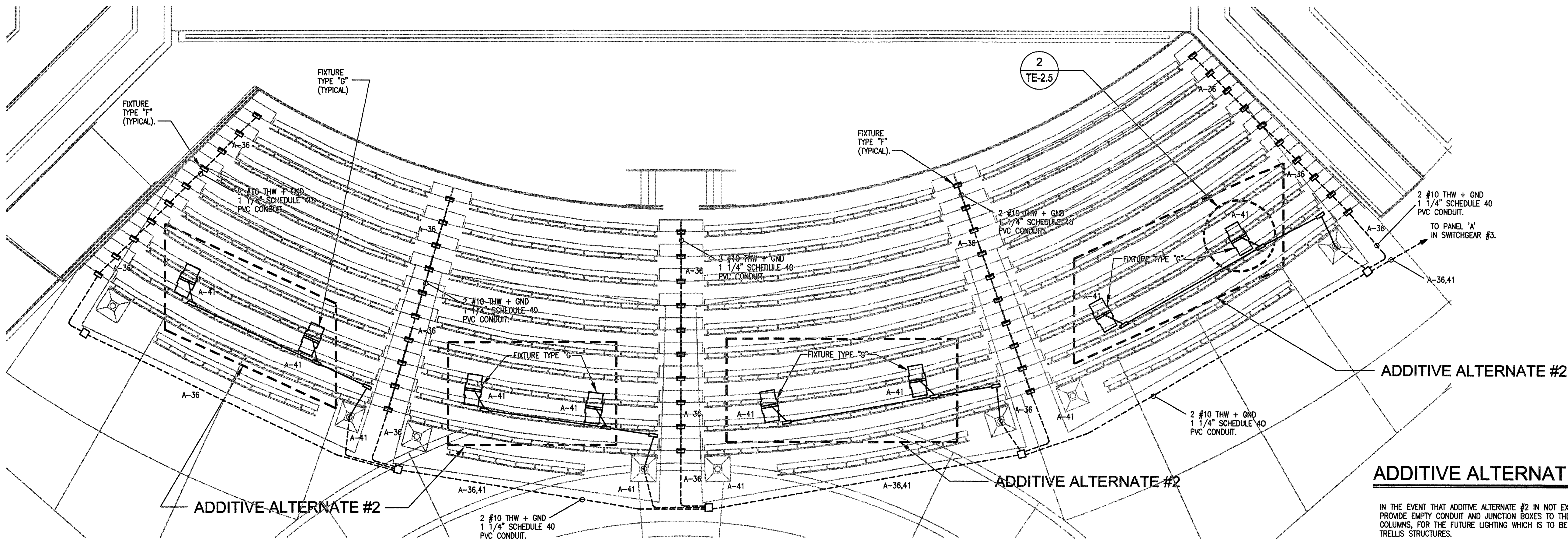
3 TE-2.4 1/8" = 1'-0"
