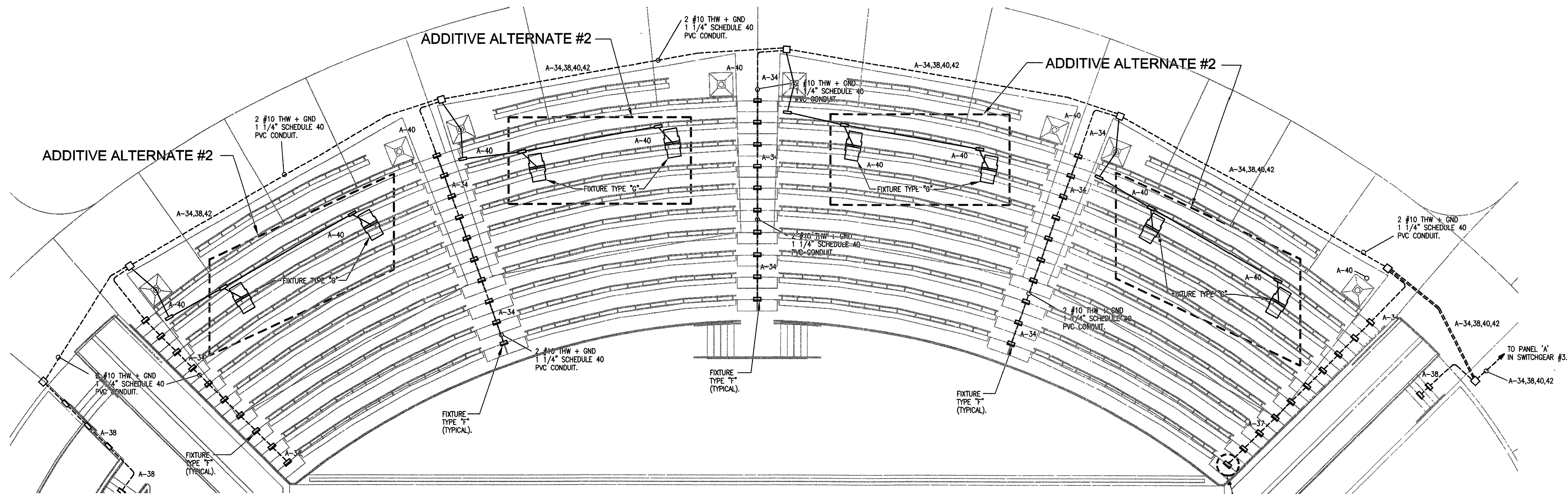
2 TE-2.4 1/8" = 1'-0"
