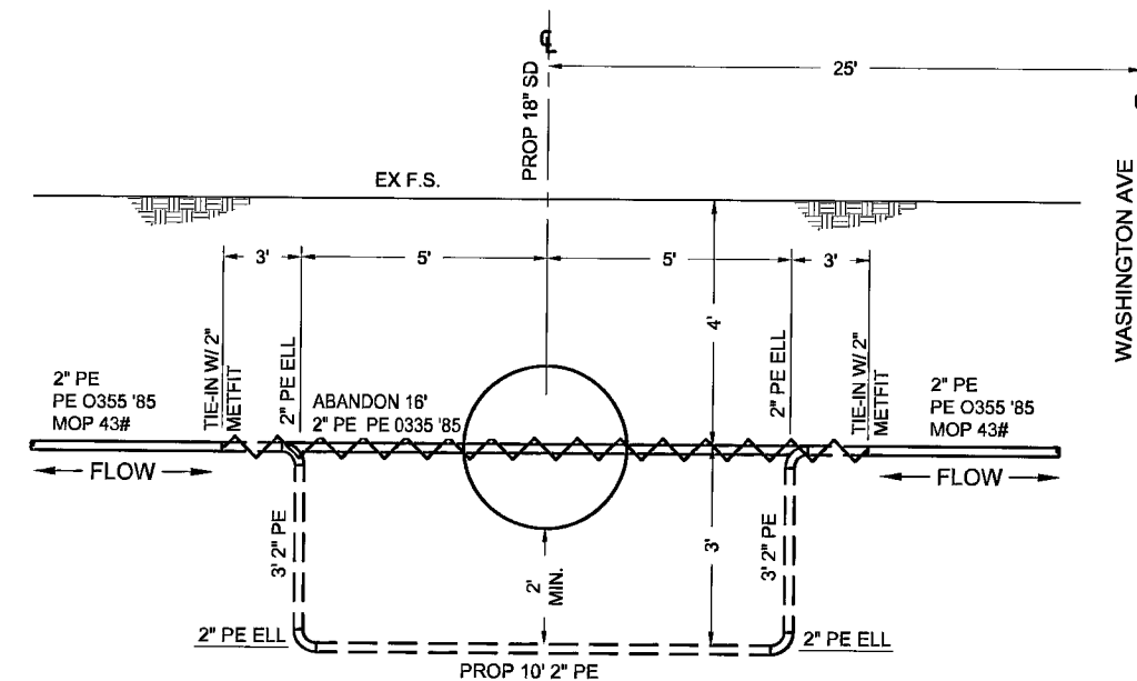
DETAIL "A" VIEW TO WEST NTS
